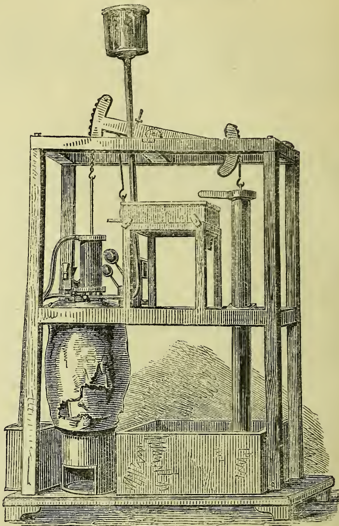
MODEL OF NEWCOMEN'S STEAM-ENGINE.
