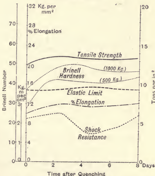
FIG. 47.—Variation in Mechanical Properties with Time after Quenching (from 300°).
