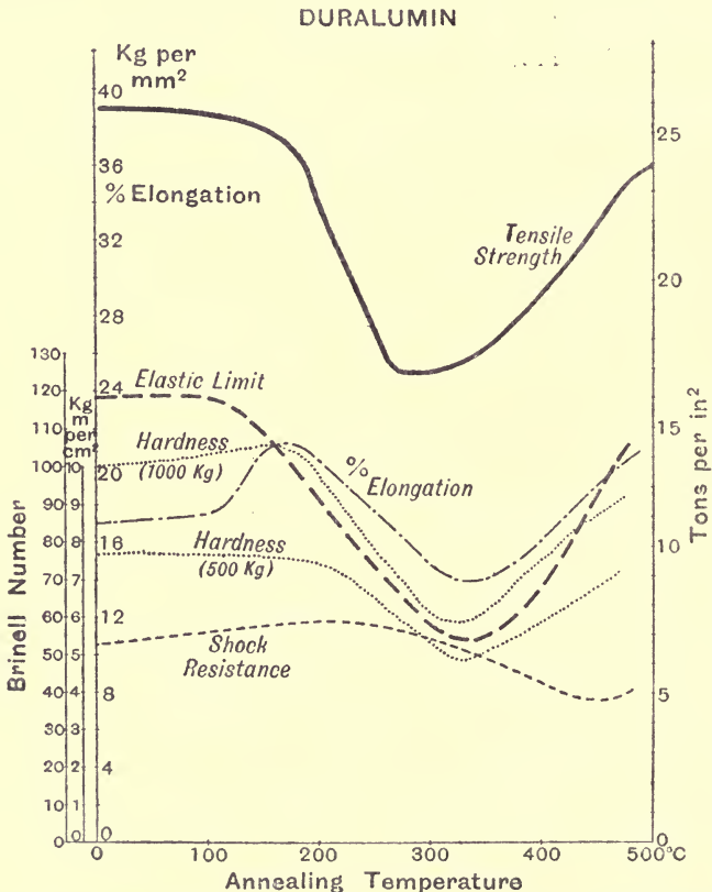
FIG. 58.—Variation in Mechanical Properties with Annealing Temperature. Metal quenched from 475^{\circ} , reannealed, and quenched in water.
