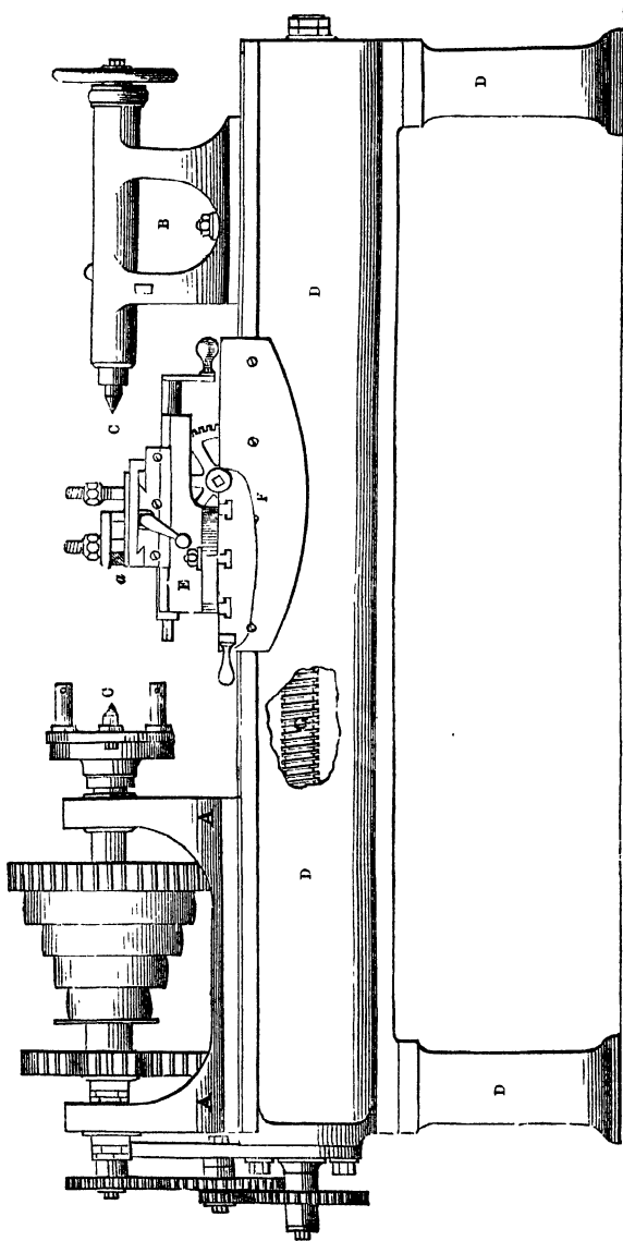
Fig. 2.—Front Elevation.
