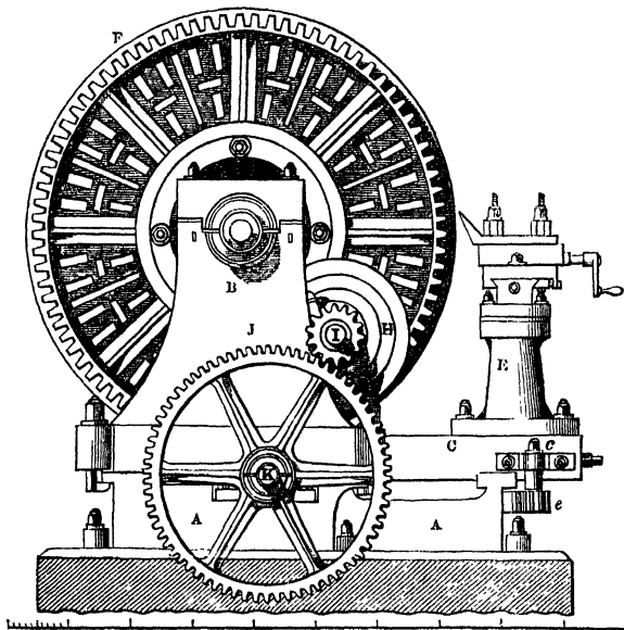
Fig. 8.—End Elevation.
