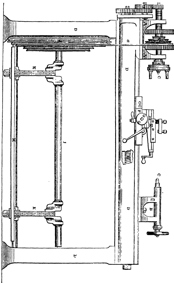
Fig. 1.—Front Elevation.
