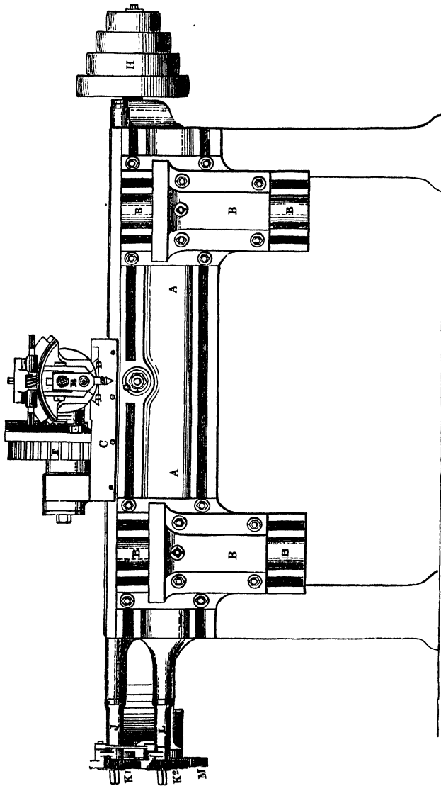
Fig. 5.—Front Elevation.
