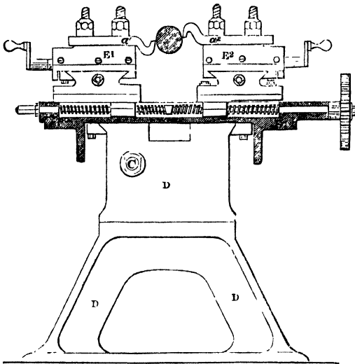
Fig. 3.—End Elevation.
