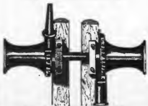
"GYPSEY WINDLASS."
