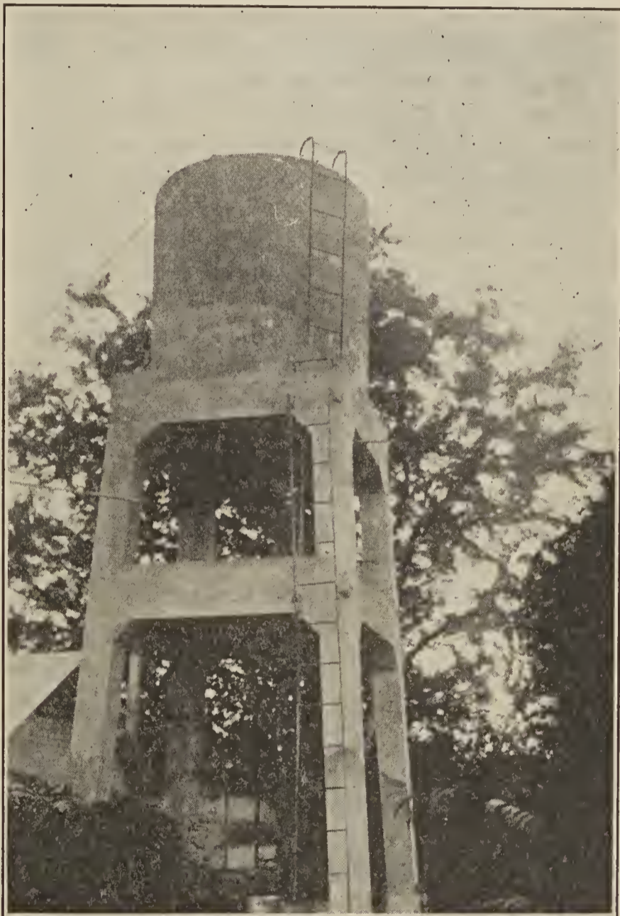
FIG. 2.—Concrete water-supply tank and tower
