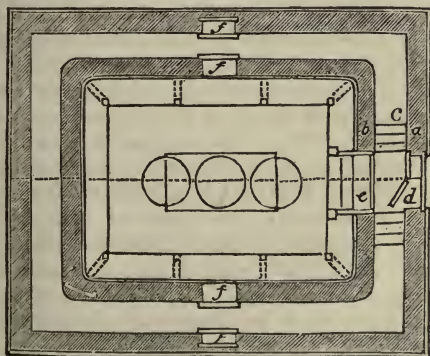
Fig. 24. Ground Plan of a Fruit Room.
