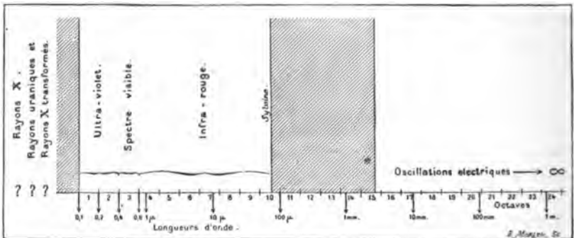
FIG. 2.—The spectrum divided into octaves. The shaded parts have not been exposed.
