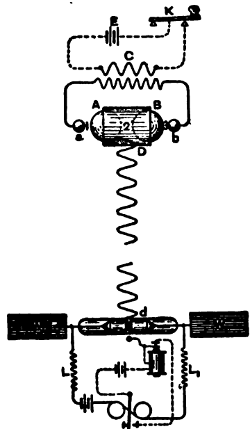
FIG. 2.—Diagram of the Marconi apparatus.
