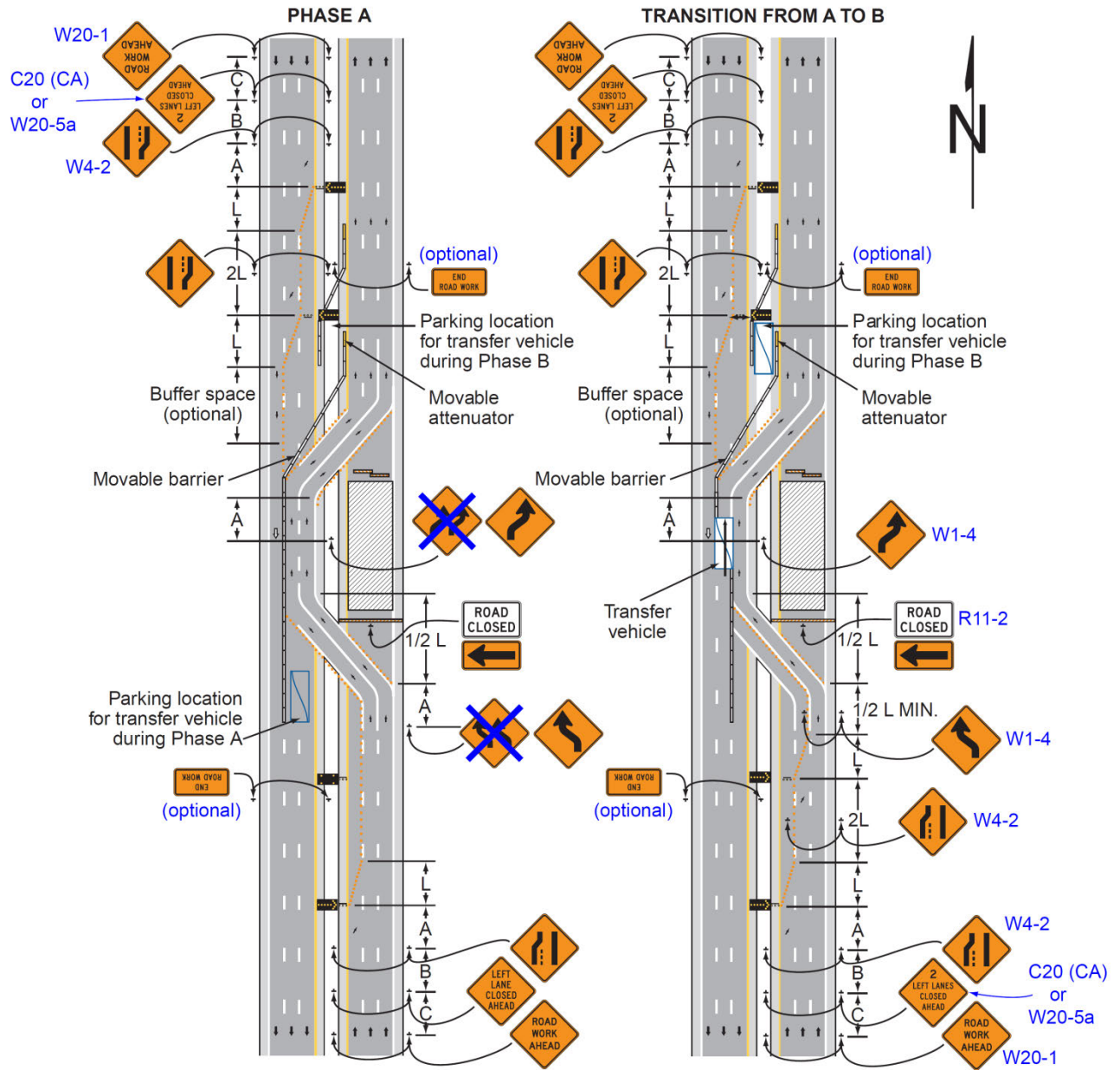
Typical Application 45
