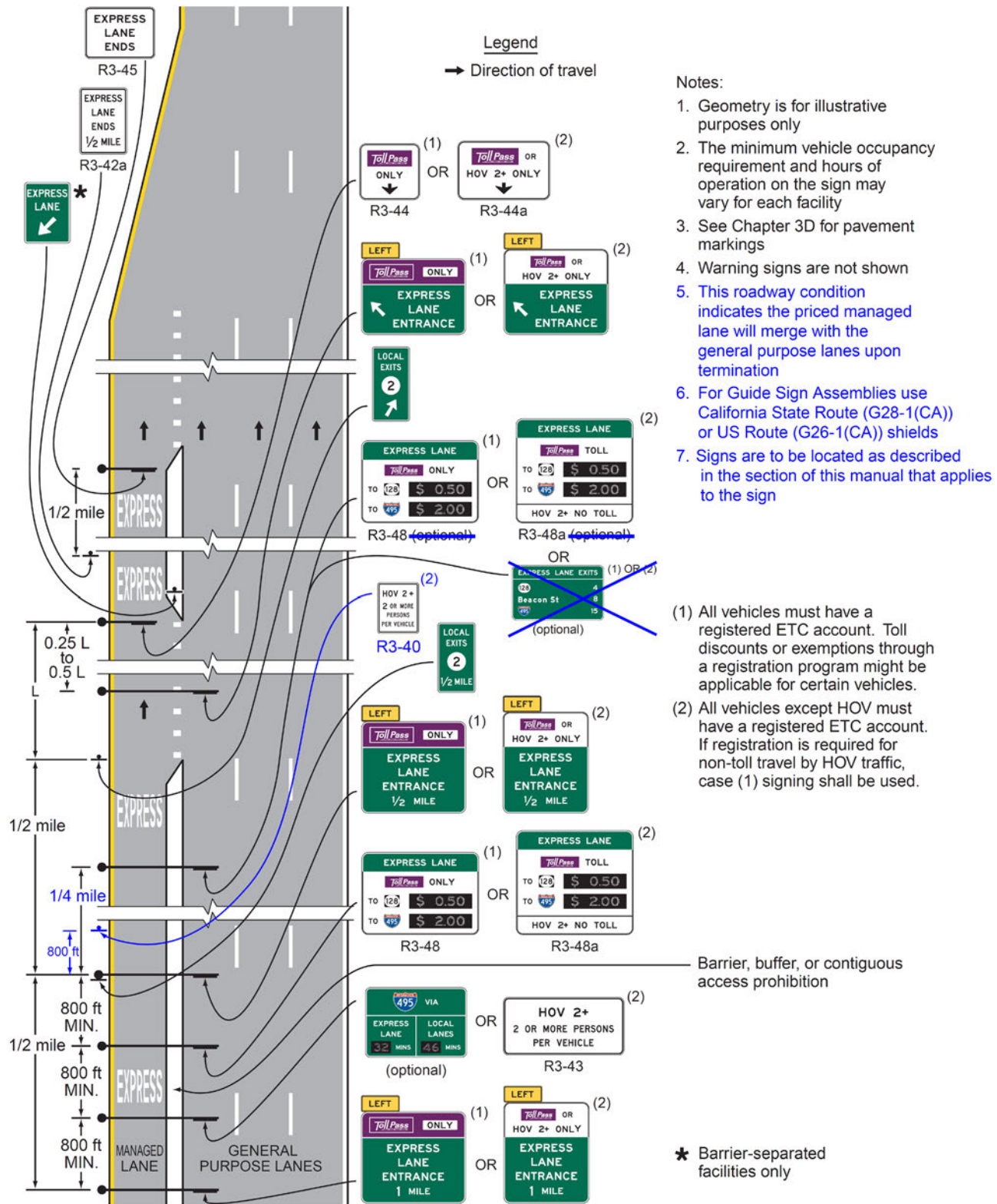
Figure 2G-24. Example of Signing for the Intermediate Entry to, Egress from, and End of Access-Restricted Price Managed Lanes
