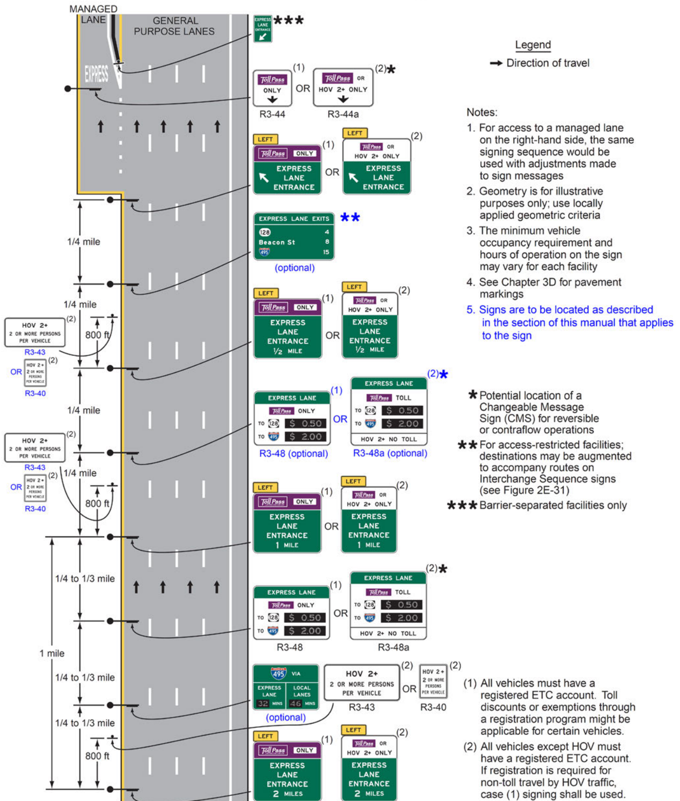
Figure 2G-21. Example of Signing for the Entrance to an Access-Restricted Priced Managed Lane
