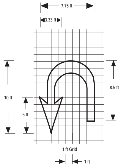
TYPE XI ARROW
