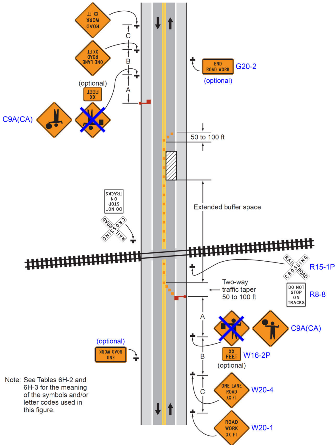
Typical Application 46
