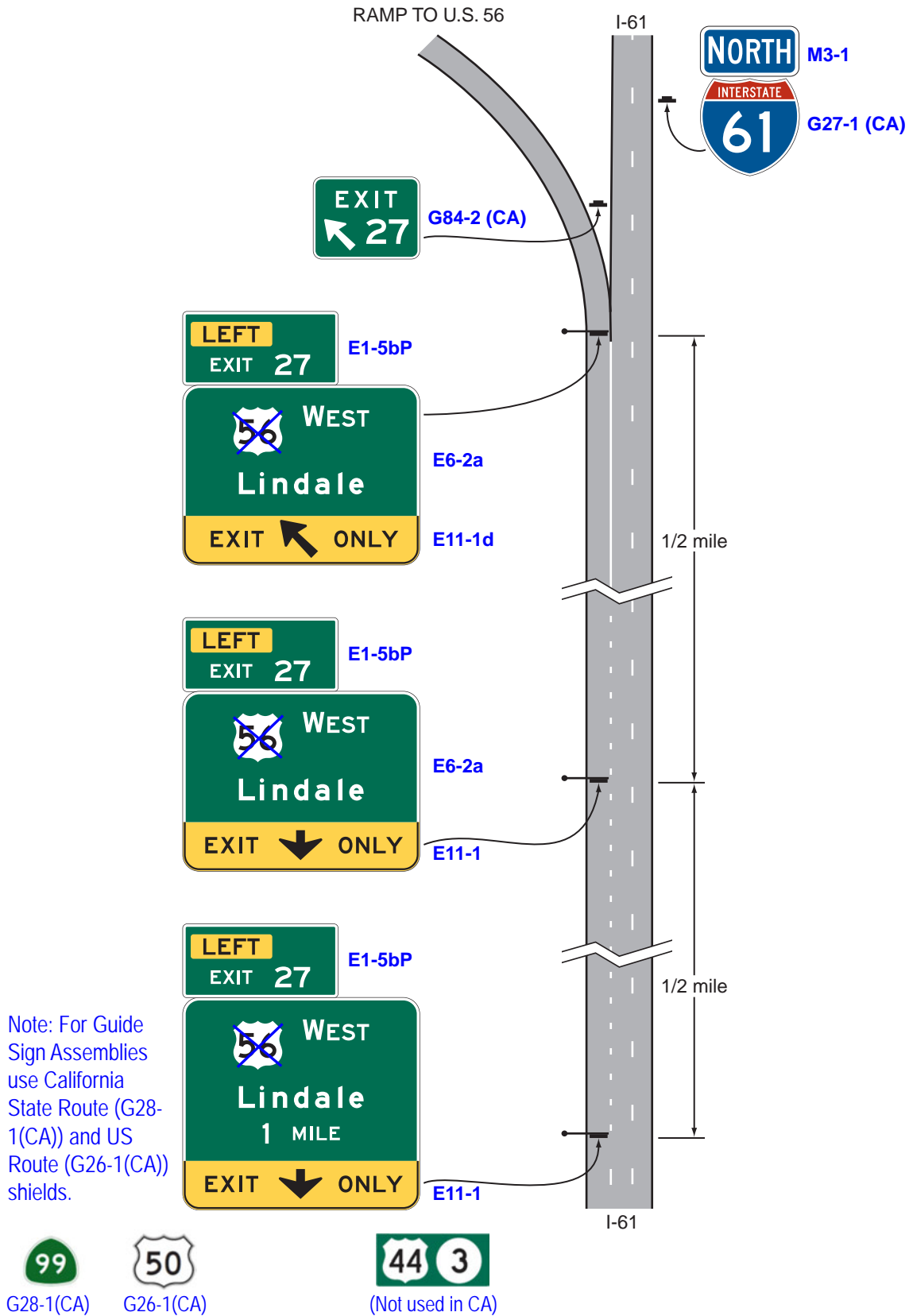
Figure 2E-15. Guide Signs for a Single-Lane Exit to the Left with a Dropped Lane
