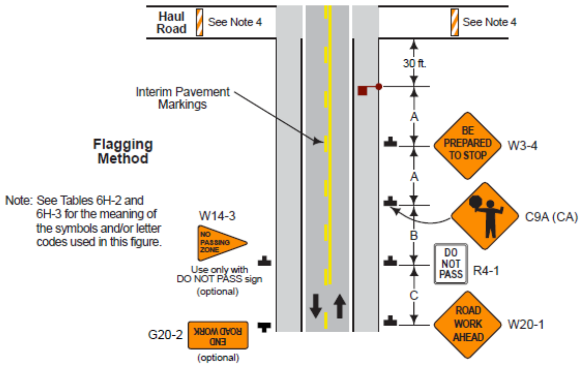
Typical Application 14
