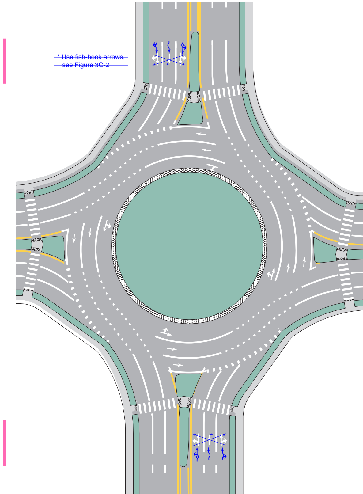
Figure 3C-11. Example of Markings for a Three-Lane Roundabout with Three-Lane Approaches
