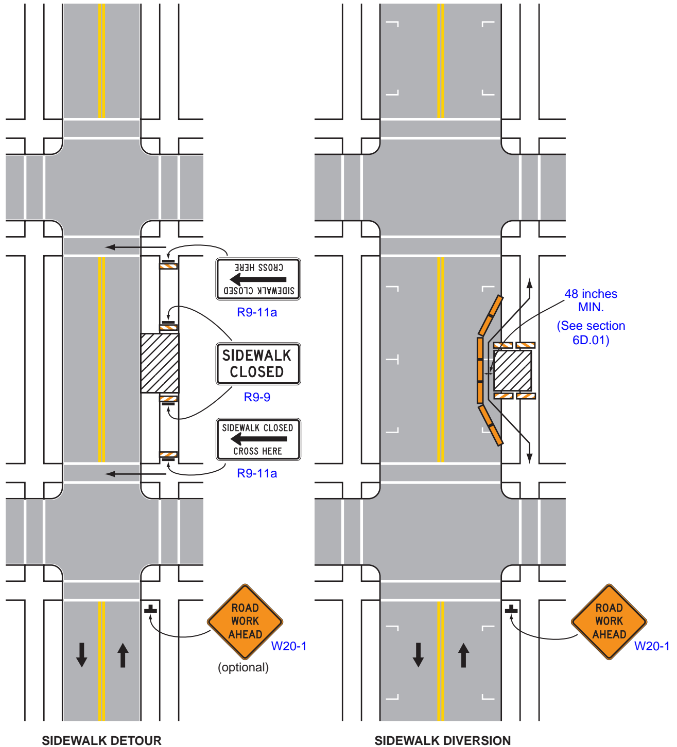
Figure 6H-28. Sidewalk Detour or Diversion (TA-28)
