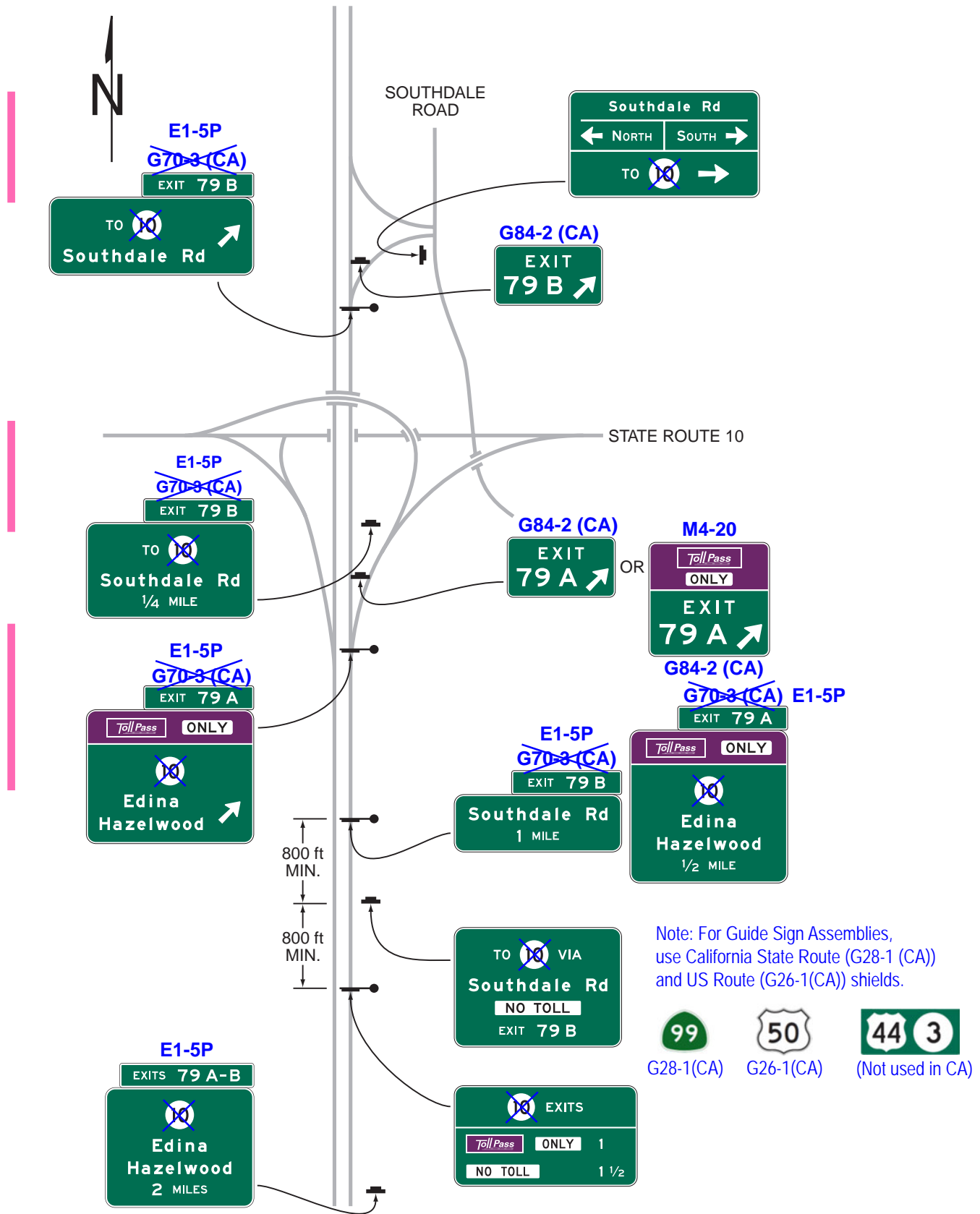
Figure 2F-7. Examples of Guide Signs for Alternative Toll and Non-Toll Ramp Connections to a Non-Toll Highway
