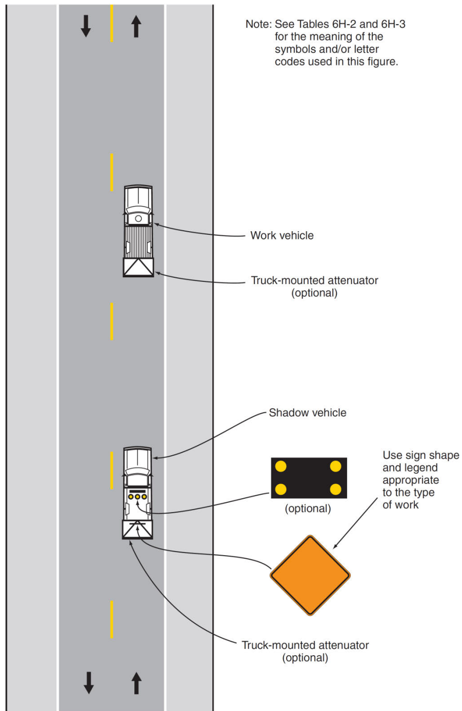
Typical Application 17
