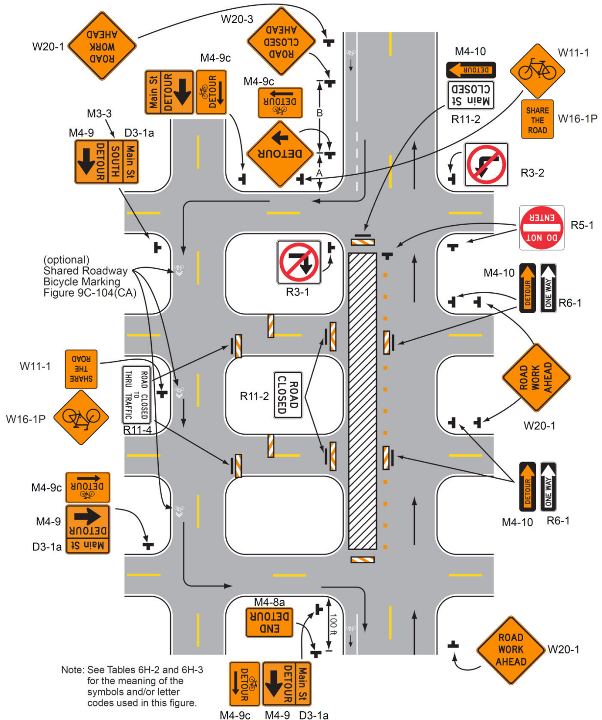
Typical Application 103 (CA)
