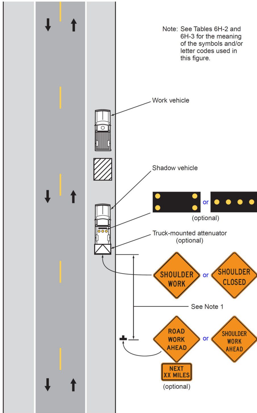
Typical Application 4
