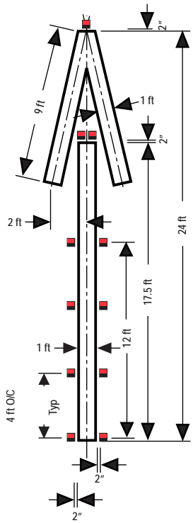
TYPE V ARROW WITH PAVEMENT MARKERS
