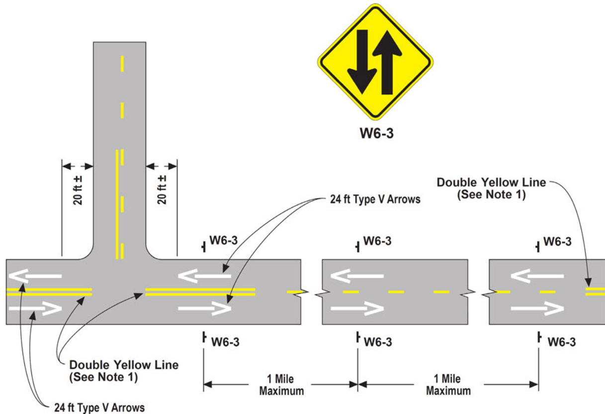
Figure 3B-104 (CA). Treatment for Divided Highway Illusion
