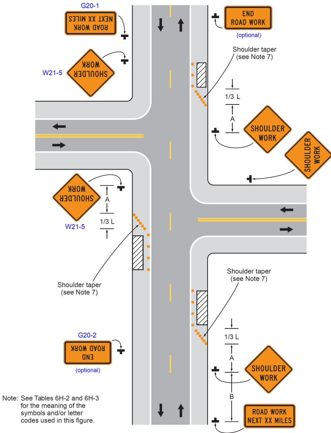
Typical Application 3
