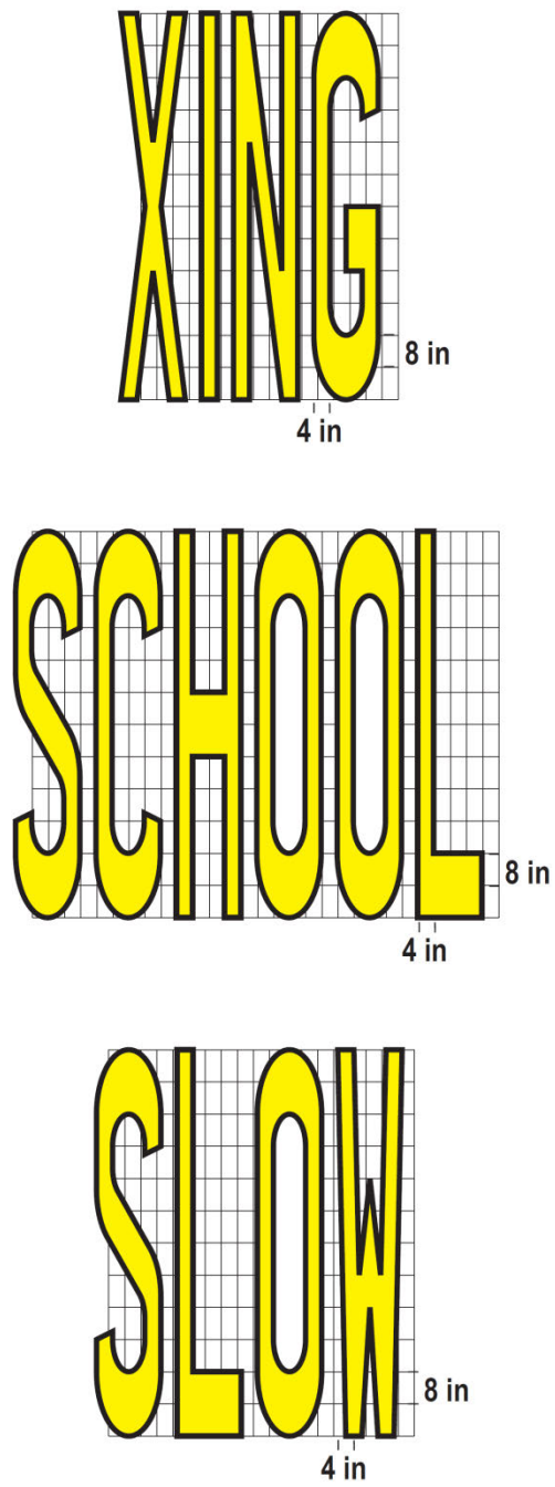
Figure 7C-101 (CA). Pavement Word Markings for School Areas
