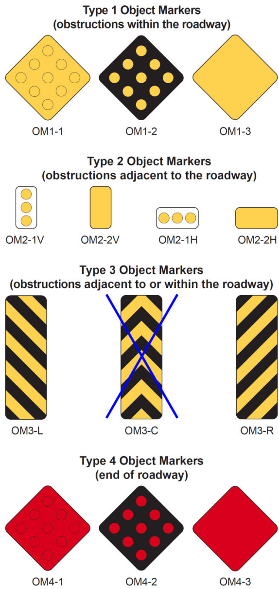
Figure 2C-13. Object Markers
