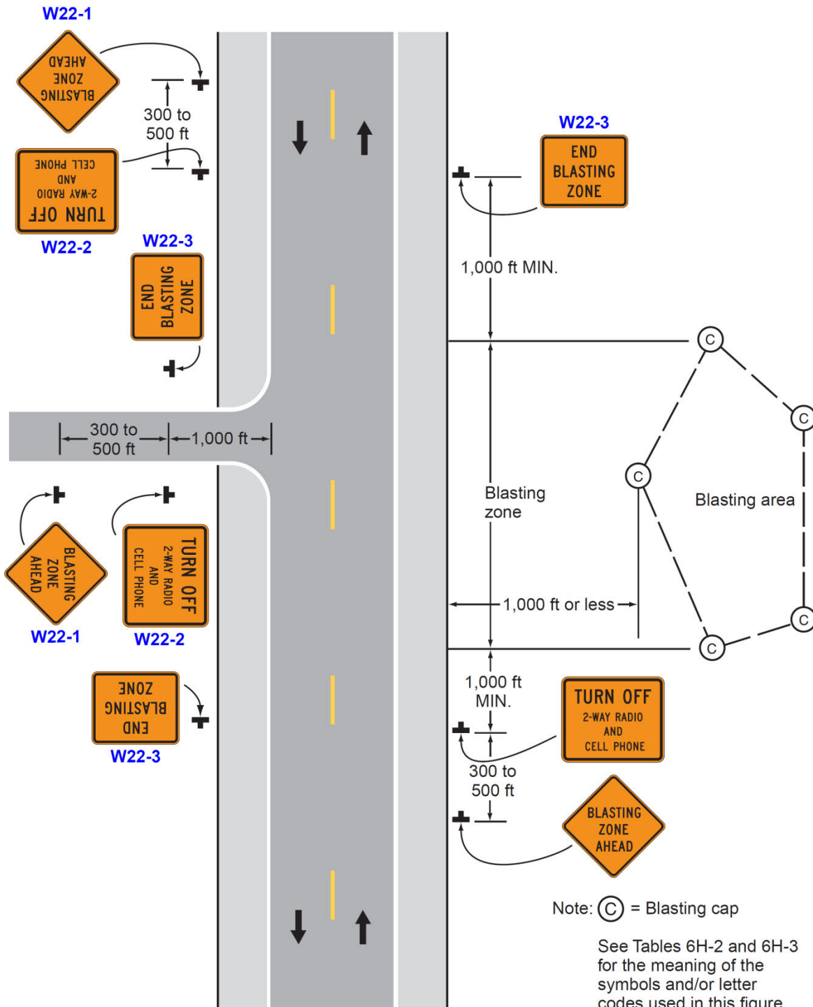
Typical Application 2
