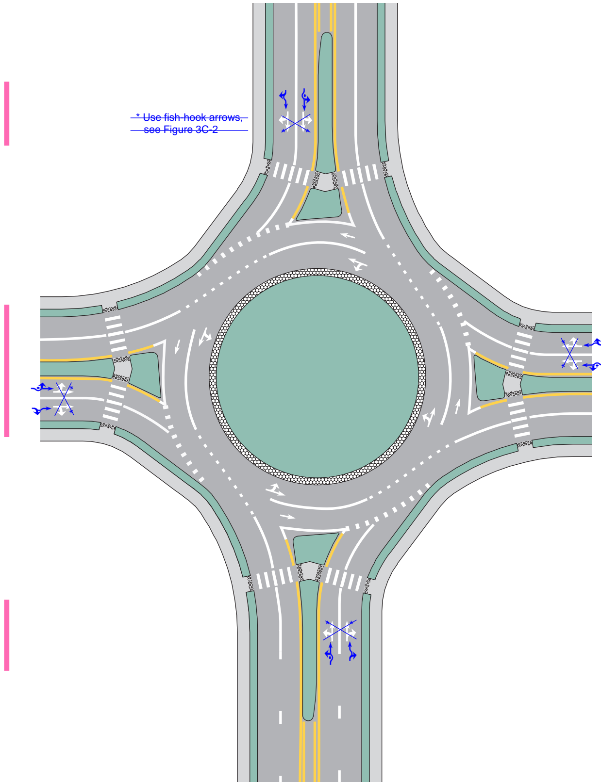
Figure 3C-6. Example of Markings for a Two-Lane Roundabout with Two-Lane Exits
