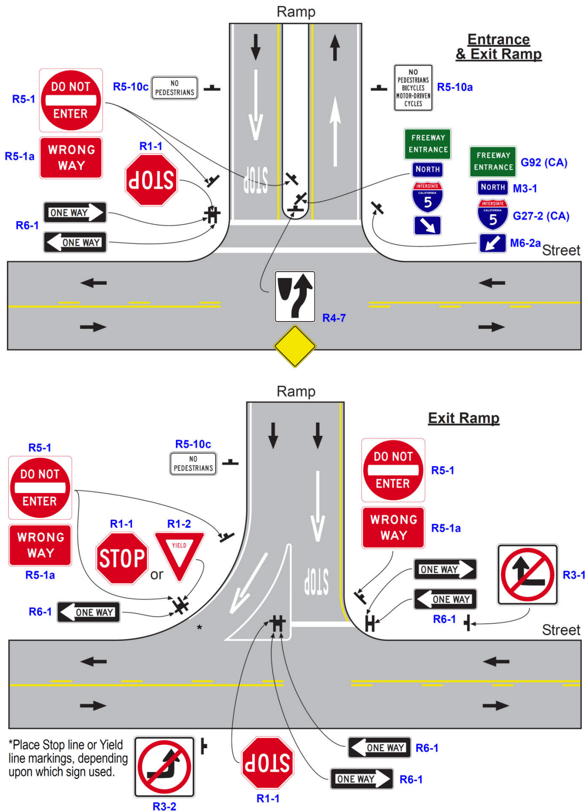
Figure 2B-18 (CA). Example of Application of Regulatory Signing and Pavement Markings at an Exit Ramp Termination to Deter Wrong-Way Entry (Sheet 4 of 5)
