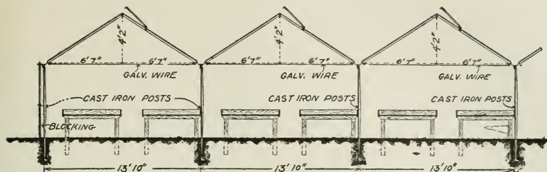
Fig. 181. Ridge- and furrow-houses with iron gutters.
