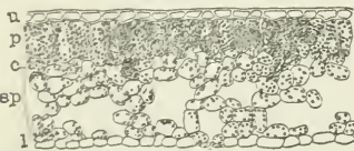
Fig. 33. Cross-section of ivy leaf, which grew in shade, and has only one layer of palisade-cells. u, upper epidermis; p, palisade cells; c, a crystal; sp, spongy parenchyma; i, intercellular space; l, lower epidermis. The plant here intended is the true or English ivy, Hedera helix .
