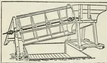
Fig. 226. Machine for seeding pulpy vegetables. The netting about the cylinder is omitted.
