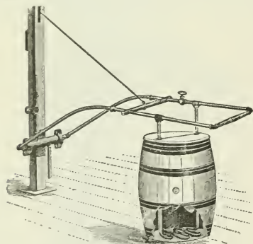
Fig. 250. A steam apple-butter cooker.
