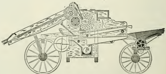
Fig. 638. Skeleton view of combination force-feed sheller.
