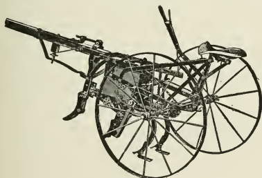
Fig. 207. Riding cotton- and corn-planter.
