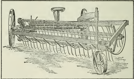
Fig. 127. Side-delivery rake of recent make.
