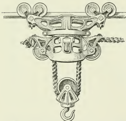
Fig. 669. Wide-mouth engine truck, swivel and reversible steel track carrier for hay forks.
