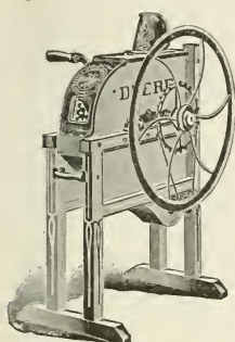
Fig. 634. One-hole corn-sheller.
