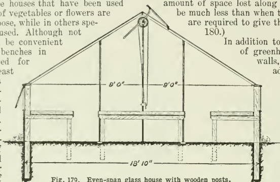
Fig. 179. Even-span glass house with wooden posts.
