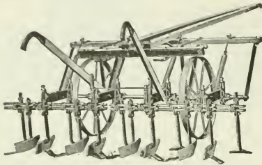
Fig. 120. Four-row beet cultivator of today.
