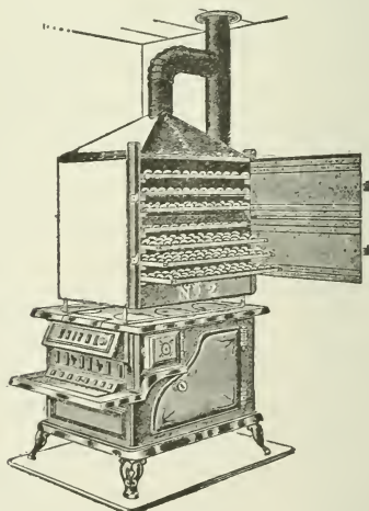
Fig. 256. Fruit evaporator adapted to kitchen stove.
