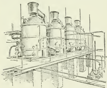
Fig. 848. Vacuum pans used in making tannin extracts.
