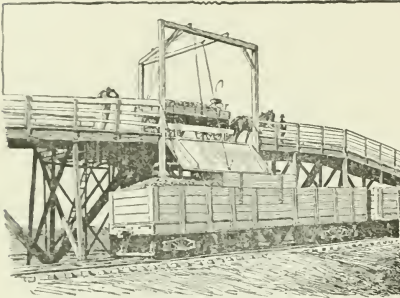
Fig. 822. Use of wagon-dump in unloading sugar-beets.
