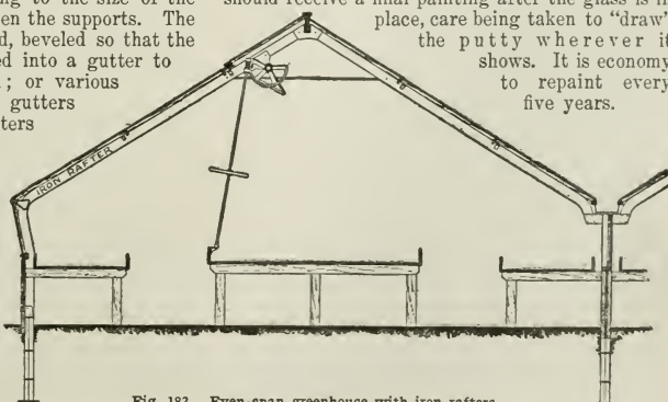
Fig. 182. Even-span greenhouse with iron rafters.
