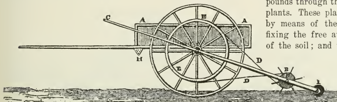
Fig. 117. Woodside's machine for harrowing, sowing and rolling, 1833. The seeder or sieve is at H; harrow at B; roller at I. "From the above it will be perceived that I can of a truth affirm, that I can sit in the front of my cart, under a canvas covering, sow the grain, harrow and roll it in, without exposure to the sun, leaving the ground without any impression of the horses' feet, my own feet, or the cart wheels."
