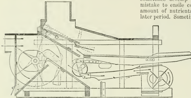
Fig. 636. Skeleton view of a corn-cleaner.
