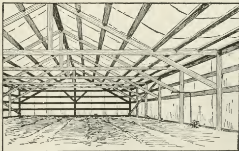
Fig. 176. Interior construction of house shown in Fig. 175.
