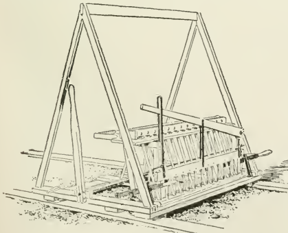
Fig. 408. Nursery planting machine used in breeding experiments.
