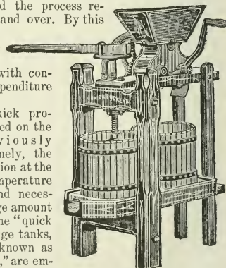
Fig. 269. Farm cider press.
