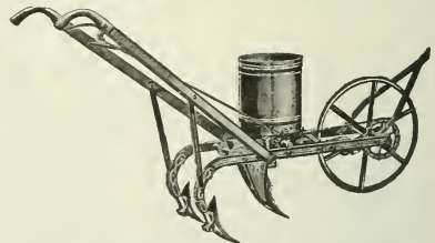
Fig. 201. One-horse combined cotton- and corn-planter.
