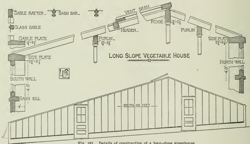
Fig. 183. Details of construction of a long-slope greenhouse.
