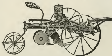
Fig. 208. A sulky lister, for planting corn.
