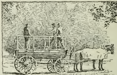
FIG. 68. Spraying outfit that will give good service in an apple orchard of forty to sixty acres.
