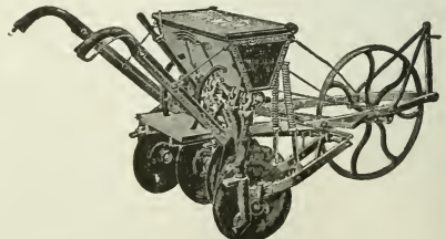
Fig. 203. A five-disk grain-drill.
