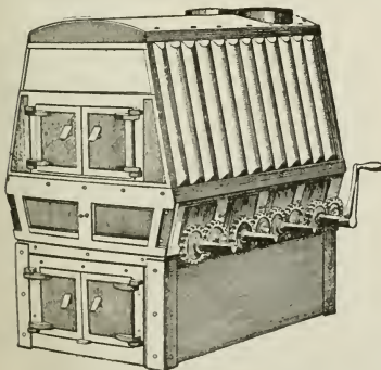
Fig. 258. Fruit evaporator and furnace.
