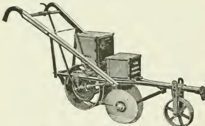
Fig. 197. A one-horse disk corn-planter.
