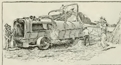
Fig. 571. Hemp-cleaning machine in operation in Kentucky.
