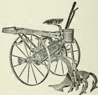
Fig. 621. Combined sulky lister and planter.
