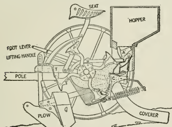
Fig. 754. A potato planter in cross-section.
