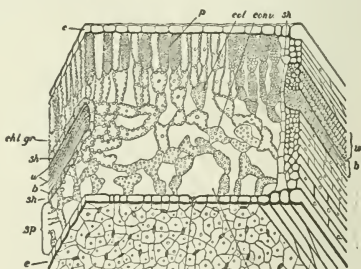
Fig. 34. Leaf of common wild yellow mustard; e, epidermis; p, palisade cells; sp, spongy parenchyma; chl, collecting cells; conv, conveying cells; sh, conducting sheath of vein; w, woody tissue of vein; b, bast of vein; s, stoma; a, air-space; chl-gr., chlorophyll granules.
