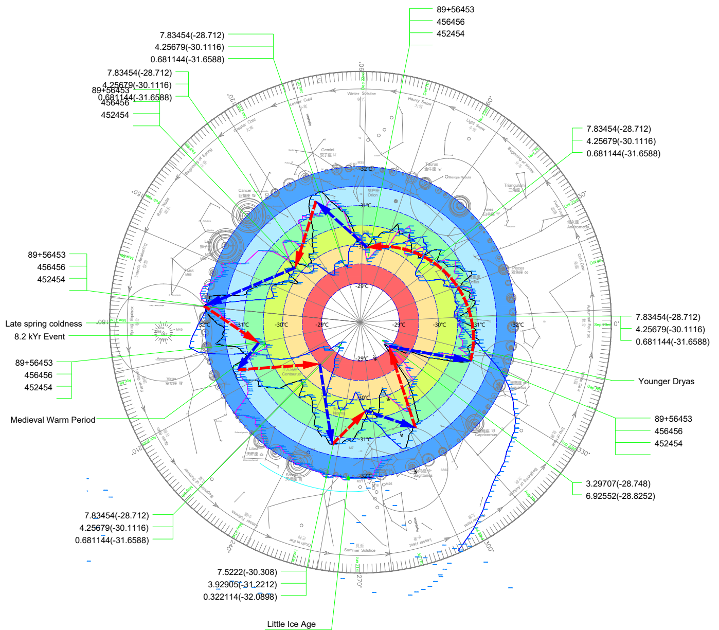
Fig.5 A 3,600-year cycle of ice core reconstruction temperatures in Greenland (GISP2)
