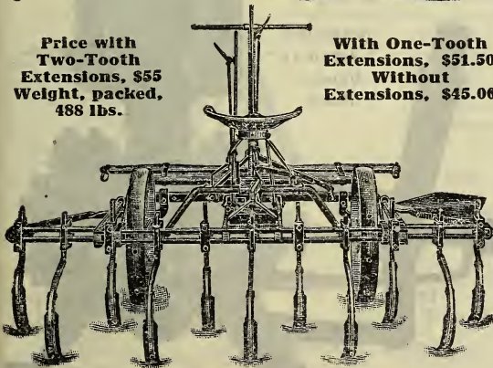
No. 41 Planet Jr. Orchard and Universal Cultivator
