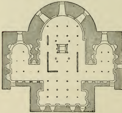
Fig. 194. St. Mark's. Plan of Crypt.
