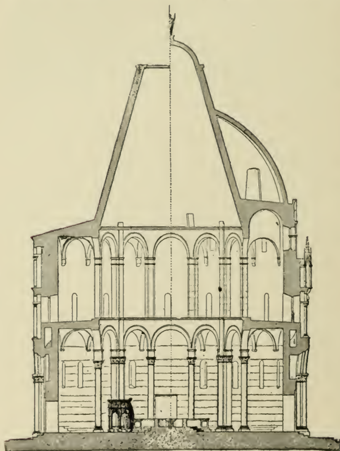
Fig. 218. Pisa. Section of Baptistery.
