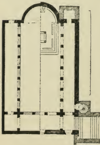
Fig. 22. Plan of St. Agnes.
