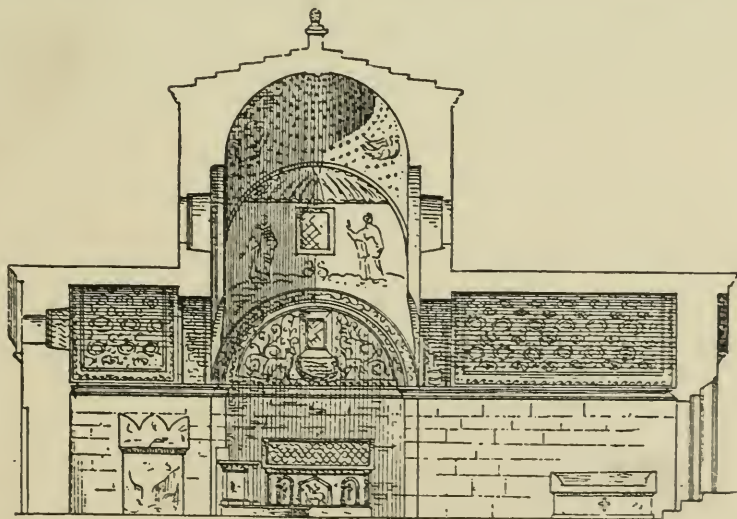
Fig. 40. Mausoleum of Galla Placidia. Section.
