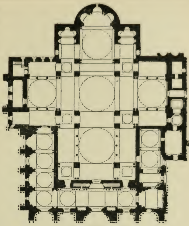
Fig. 191. Plan of St. Mark's, Venice.
