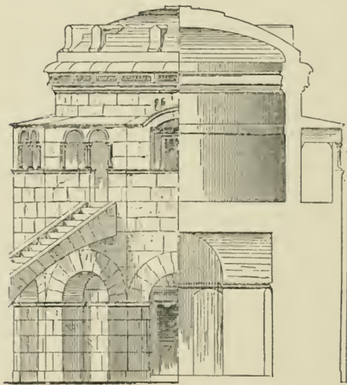
Fig. 53. Elevation and Section of Mausoleum of Theodoric.
