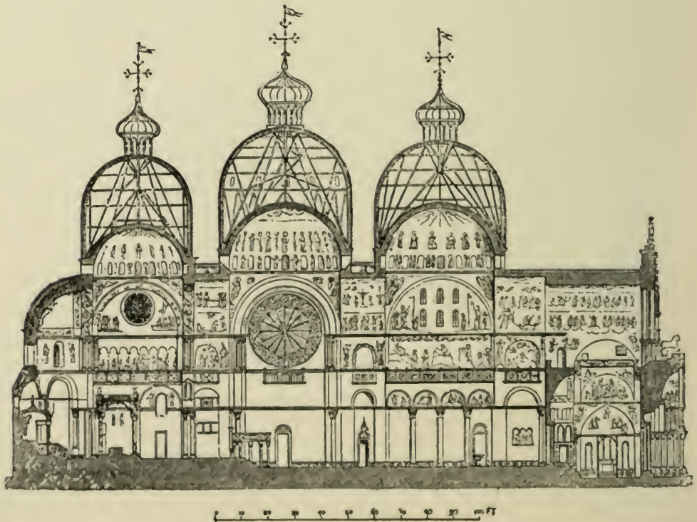
Fig. 192. Longitudinal Section of St. Mark's.
