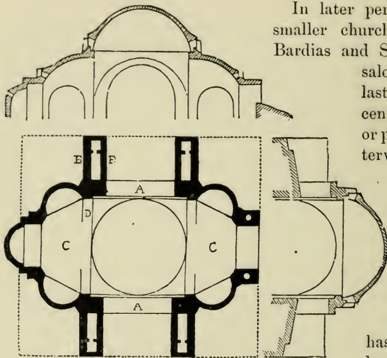
Fig. 141. Plan and Sections, S. Sofia.
