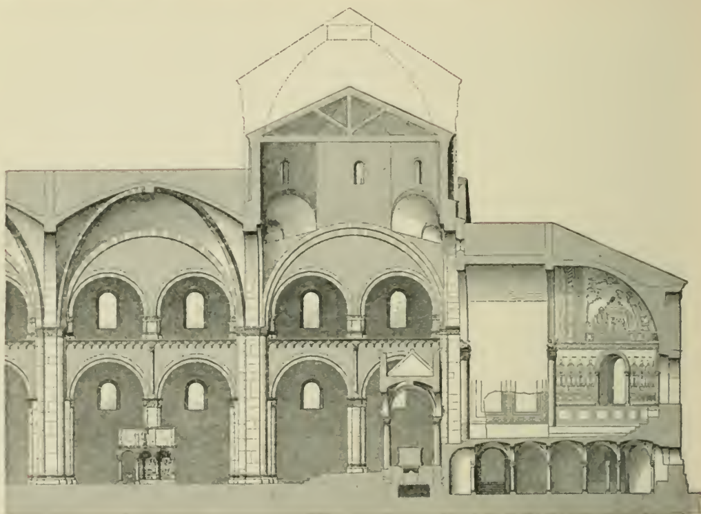
Fig. 64. Section of eastern portion of S. Ambrogio.
