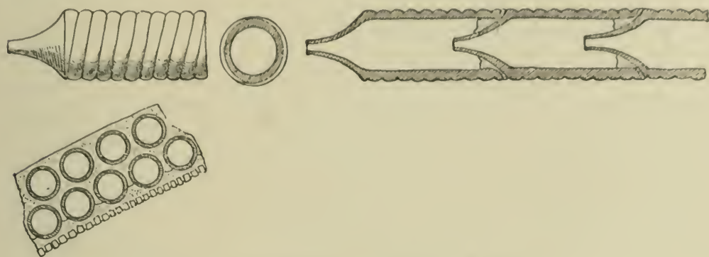
Fig. 49. Details of Dome, Ravenna Baptistery.
