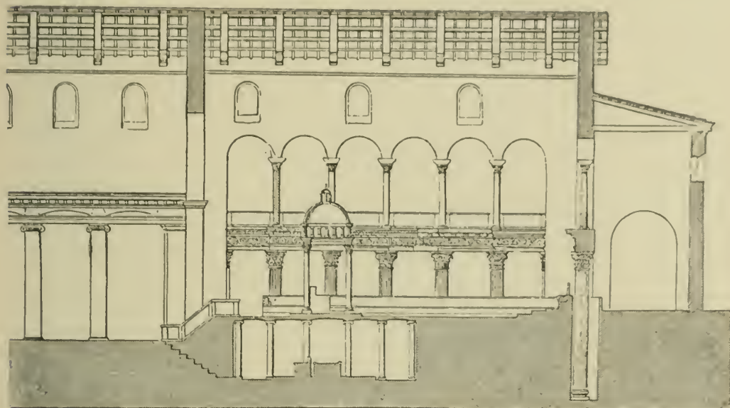
Fig. 25. S. Lorenzo. Section of the Early Church.
