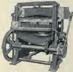
B. & C. Automatic Clamp
