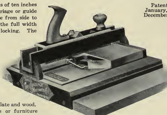
Three machines in one—Combination Shoot-Board Type-High Planer, Shaver and Miter Cutter
