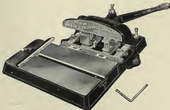
No. 214 S. & T. Punch Press, Hand Power. Punches holes to 13\frac{1}{2} inches apart, any length sheet
