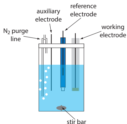
Figure 11.37 Typical electrochemical cell for voltammetry.
