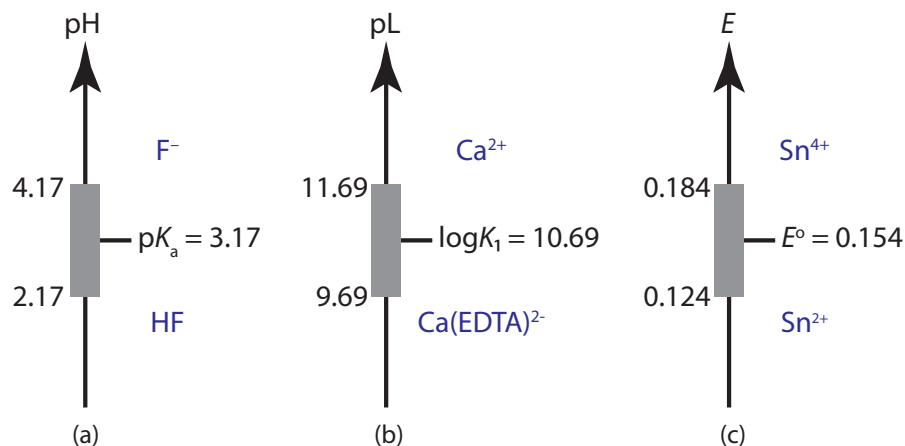
Figure 6.14 Ladder diagrams showing buffer regions shaded in grey for (a) an acid–base buffer of HF and \text{F}^- ; (b) a metal–ligand complexation buffer of \text{Ca}^{2+} and \text{Ca}(\text{EDTA})^{2-} ; and (c) an oxidation–reduction (redox) buffer of \text{Sn}^{4+} and \text{Sn}^{2+} .
