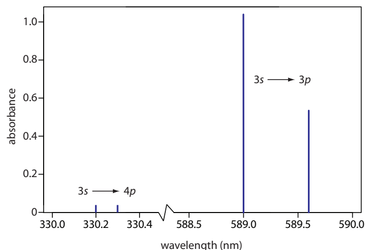
Figure 10.20 Atomic absorption spectrum for sodium. Note that the scale on the x -axis includes a break.
