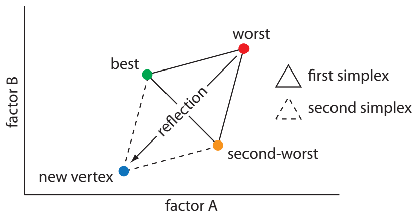
Figure 14.10 Example of a two-factor simplex. The original simplex is formed by the green , orange , and red vertices. Replacing the worst vertex with a new vertex moves the simplex to a new position on the response surface.
