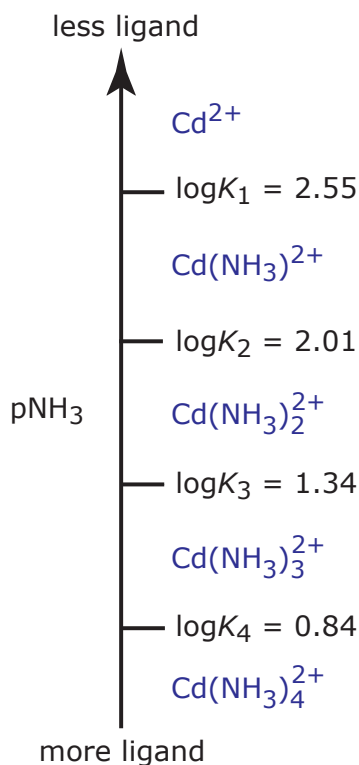
Figure 6.7 Metal–ligand ladder diagram for Cd 2+ –NH 3 complexation reactions. Note that higher-order complexes form when pNH 3 is smaller (which corresponds to larger concentrations of NH 3 ).
