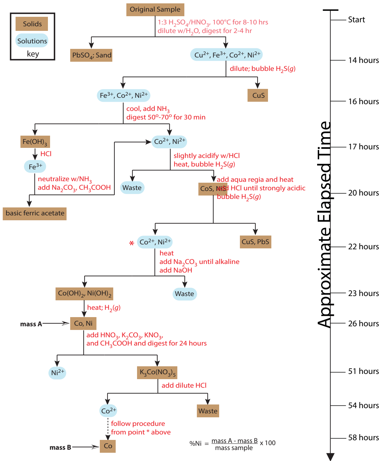
Figure 1.1 Fresenius' analytical scheme for the gravimetric analysis of Ni in ores. After each step, the solid and the solution are separated by gravity filtration. Note that the mass of nickel is not determined directly. Instead, Co and Ni first are isolated and weighed together ( mass A ), and then Co is isolated and weighed separately ( mass B ). The timeline shows that it takes approximately 58 hours to analyze one sample. This scheme is an example of a gravimetric analysis, which is explored further in Chapter 8.
