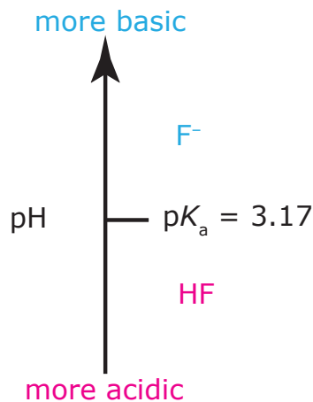
Figure 6.6 Acid–base ladder diagram for HF. To minimize the solubility of CaF 2 , we need to keep the pH above 3.17, with more basic pH levels leading to smaller solubility losses. See Chapter 8 for a more detailed discussion.
