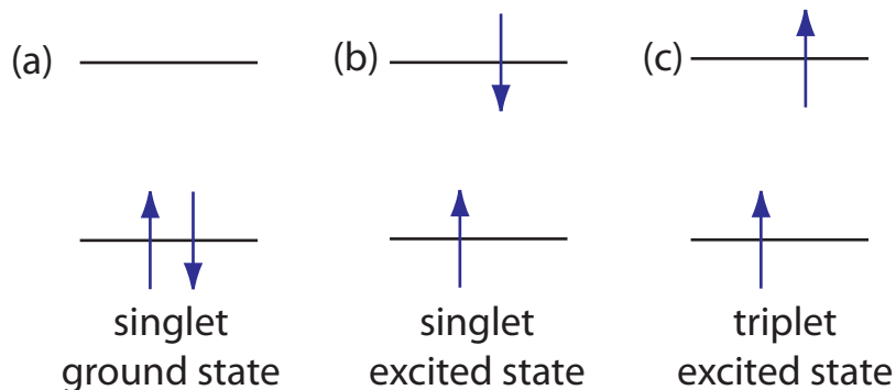
Figure 10.47 Electron configurations for (a) a singlet ground state; (b) a singlet excited state; and (c) a triplet excited state.
