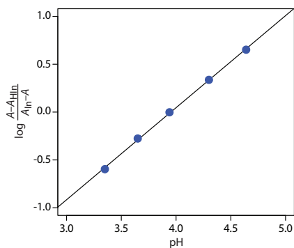
Figure 10.69 Determining the \text{p}K_a of bromothymol blue using the data in Practice Exercise 10.10.
