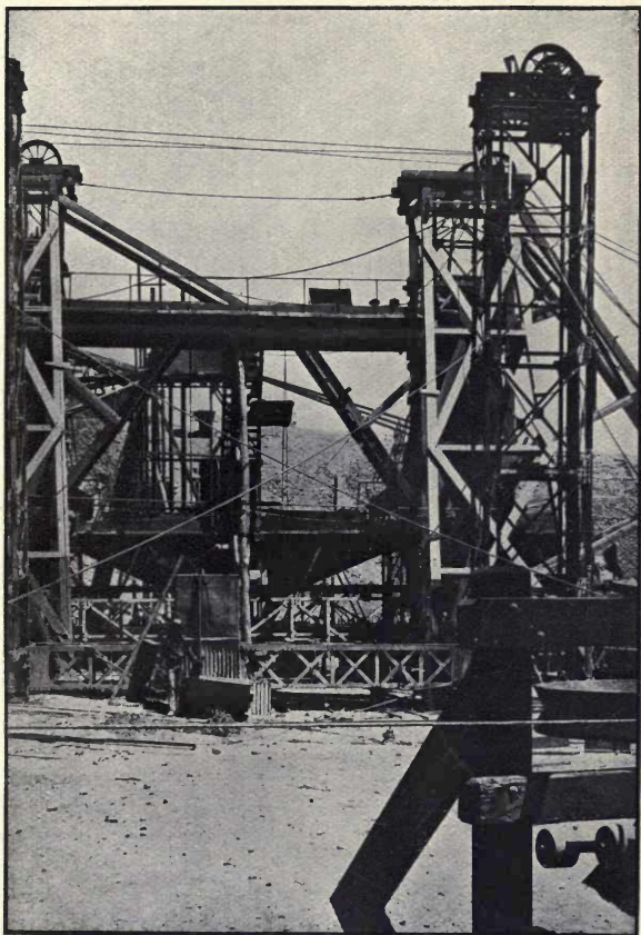
FIG. 8. DE BEERS WASHING AND CONCENTRATING MACHINERY.
