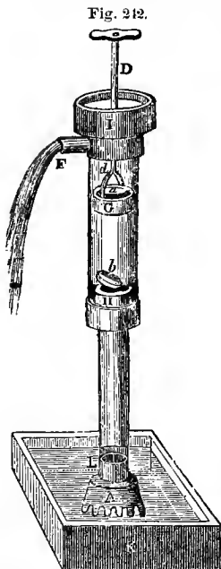
Common Pump : b , lower or fixed valve, G , piston with valve, a , opening upward; D , piston-rod; F , spout.
