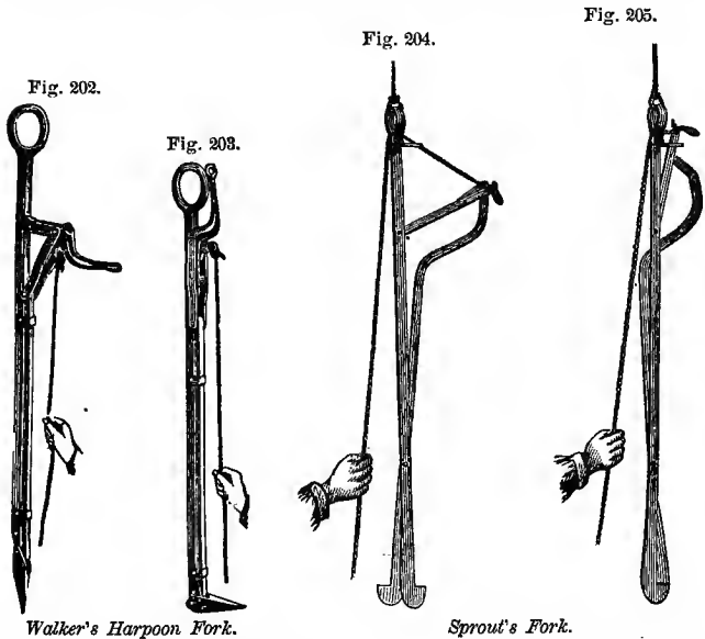
Walker's Harpoon Fork.
