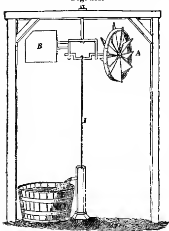
Wind-mill for pumping water on farms: A, wind-mill; B, vane; I, pump-rod.
