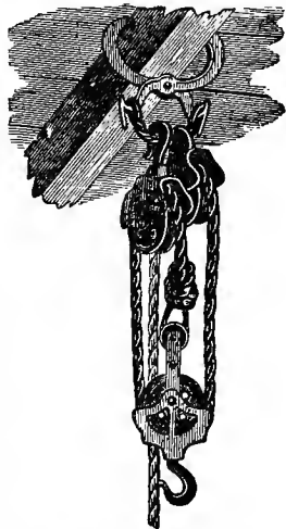
Grappling Irons and Hoisting Tackle.
