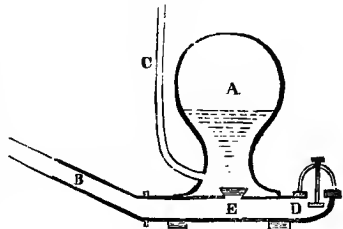
Water-ram.
