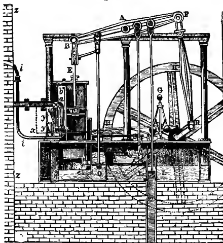
Low-pressure Steam-engine.
