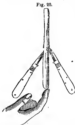
Fig. 20. Centre of gravity maintained by two penknives.
