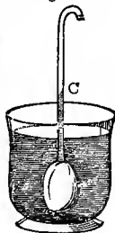
Apparatus explaining the rising of sap.
