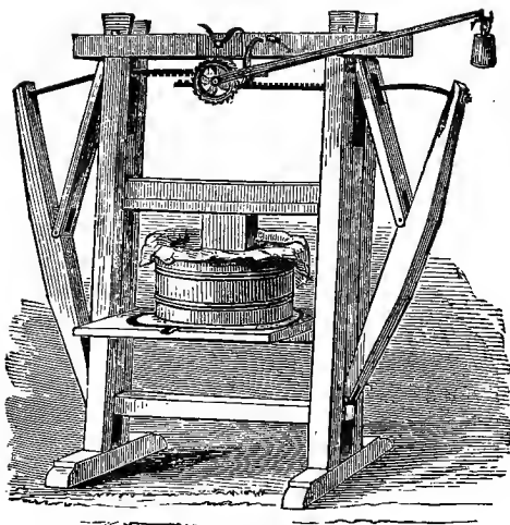
Kendall's Cheese-press.
