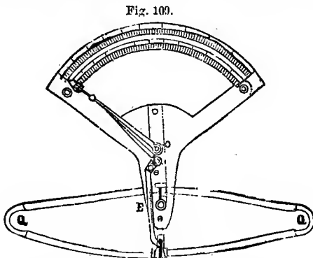
Elliptic Dynamometer.
