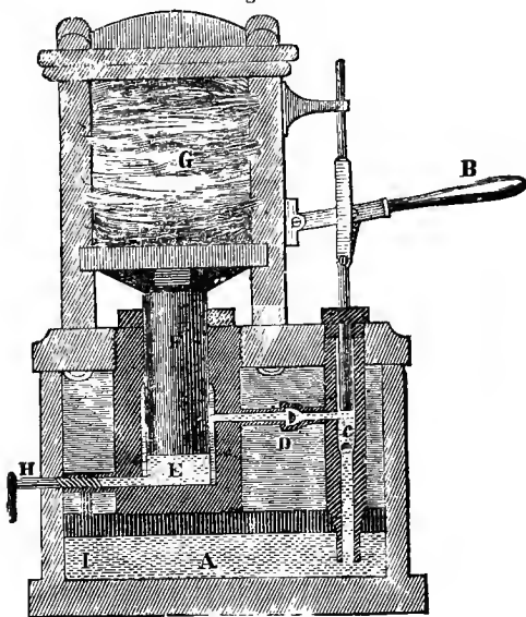
Hydrostatic Press.
