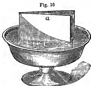
Capillary attraction between two panes of glass.
