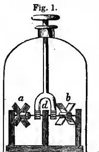
Fig. 1. Fans revolving in a vacuum.
