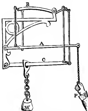
Compound levers.
