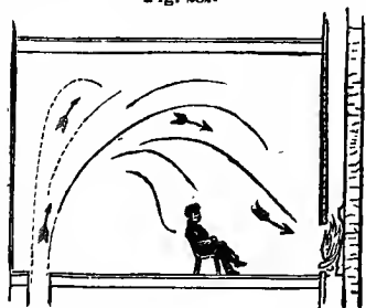
Furnace and Open Fire-place Combined.
