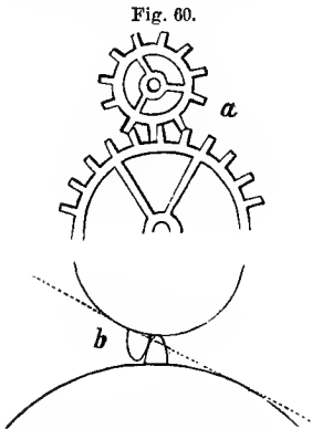
Form of cogs— a , badly formed; b , proper form.
