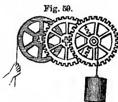
Combined cog-wheels.
