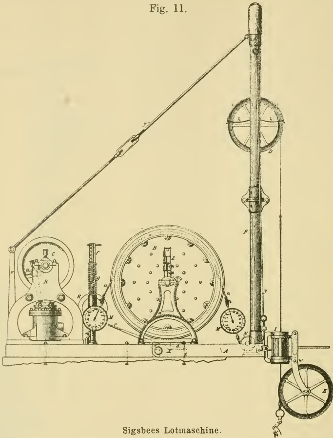
Sigsbees Lotmaschine.
