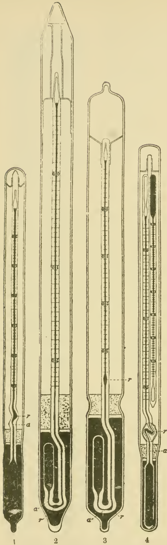
Moderne Umkippthermometer.
