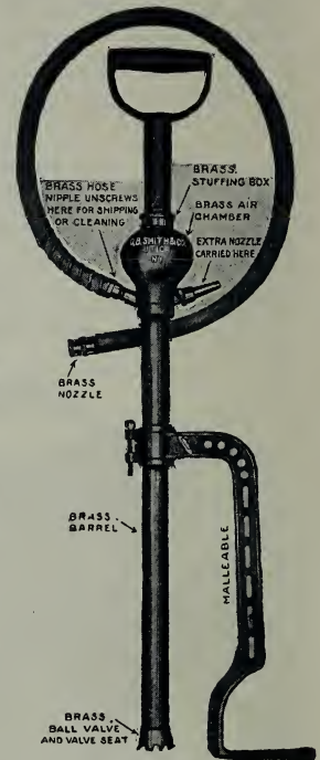
No. 32 Bucket Pump
