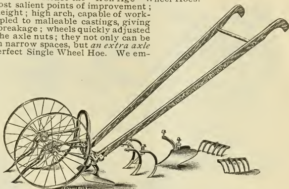
IRON AGE DOUBLE OR SINGLE WHEEL HOE.
