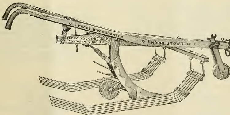
HALLOCK'S POTATO DIGGER. Price, $14.00.
