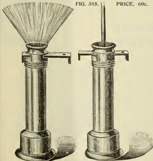
VERMORELL NOZZLE.
