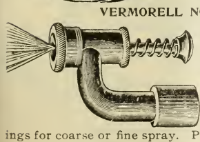
VERMORELL NOZZLE.
