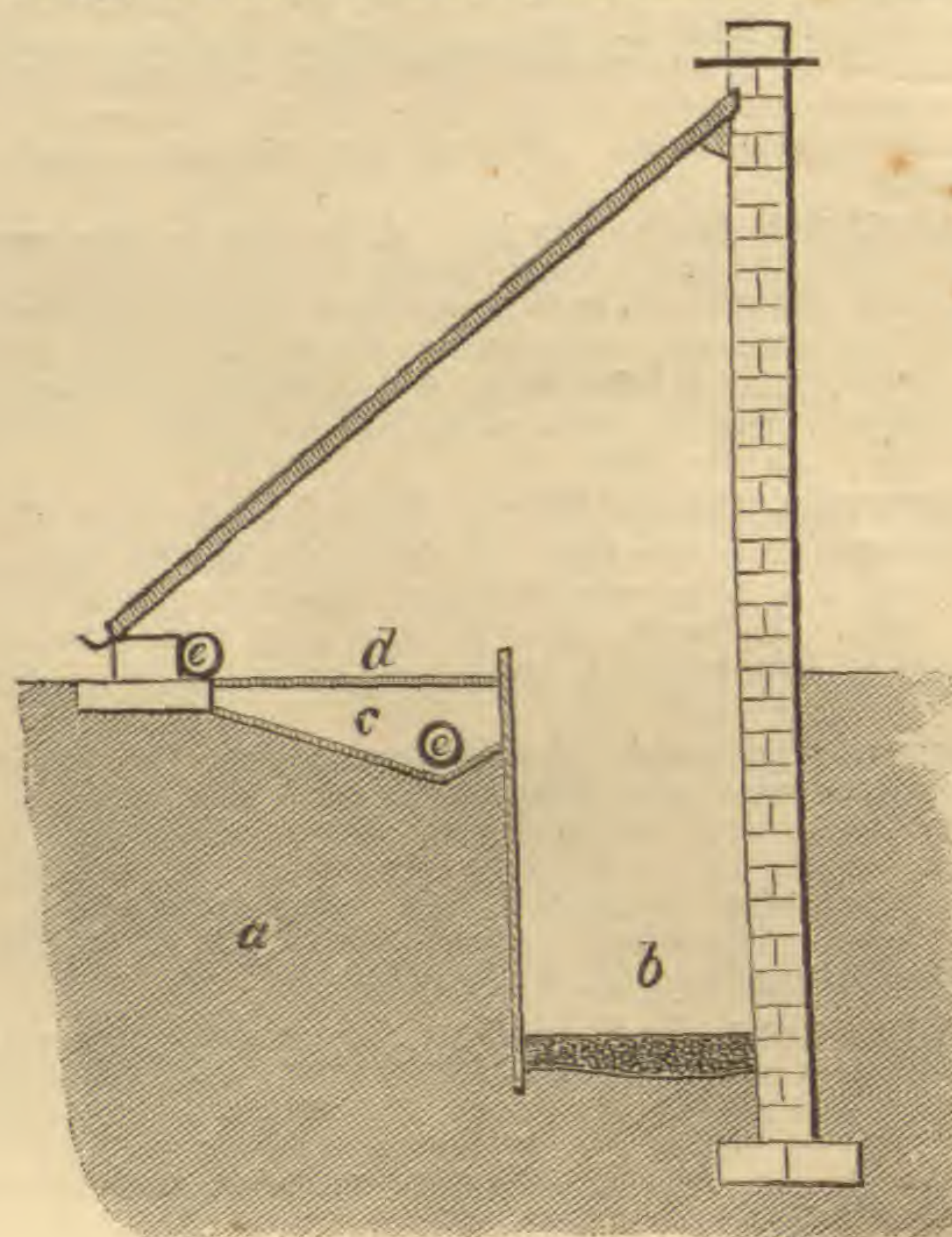
FIG. 191. SECTION OF LEAN-TO PIT.
