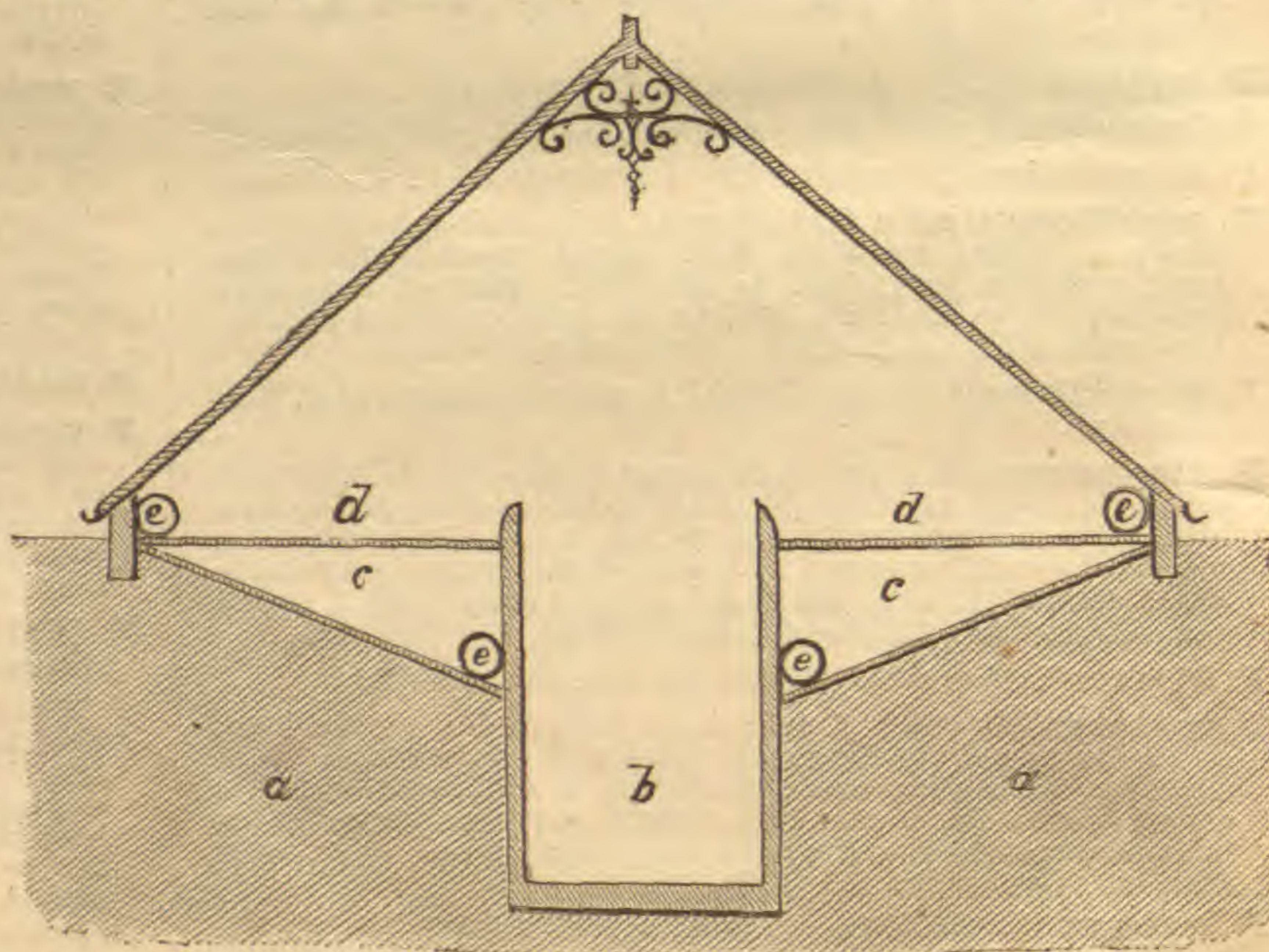
FIG. 192. SECTION OF SPAN-ROOFED PIT.
