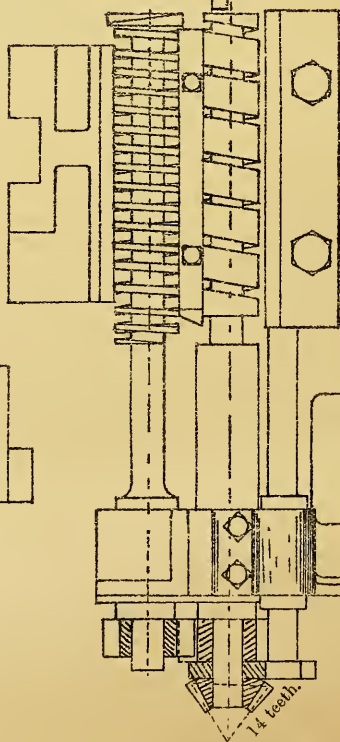
Cross Section of Bend showing Screws for gill bars.
