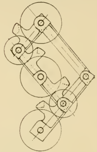
END ELEVATION OF GEAR LINK MOTION
