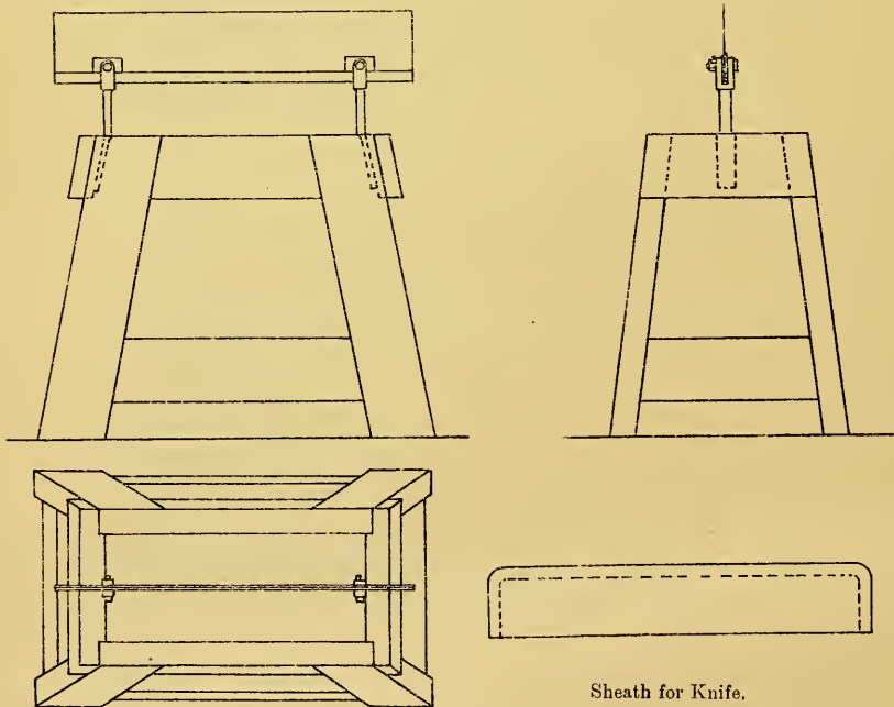
Sheath for Knife.
