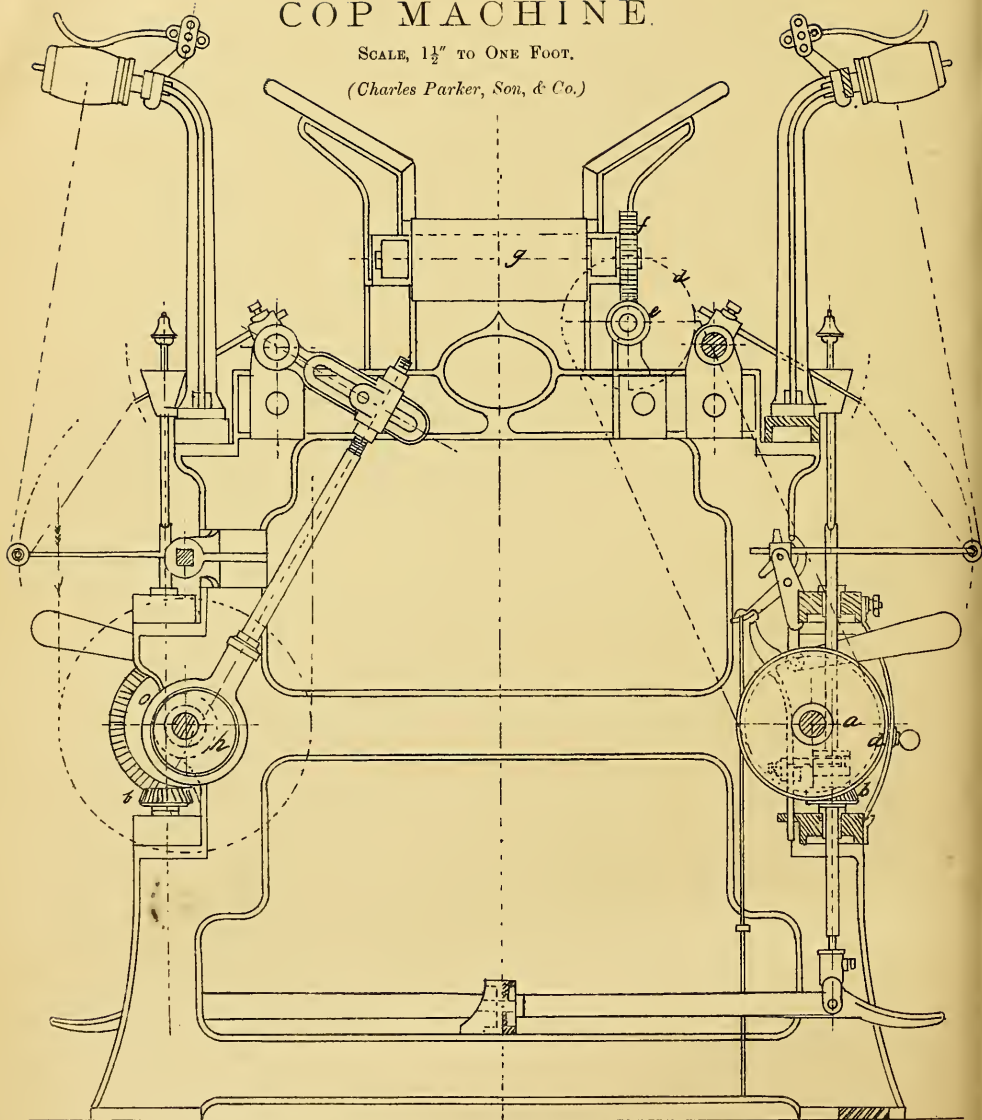
HALF END ELEVATION
