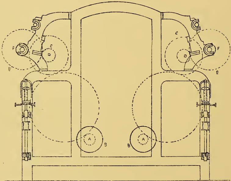
ELEVATION DRIVING END SHOWING TWIST GEARING.*
