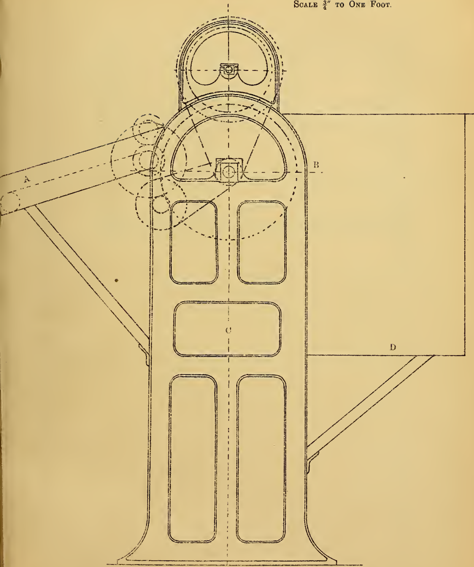
End Elevation.
