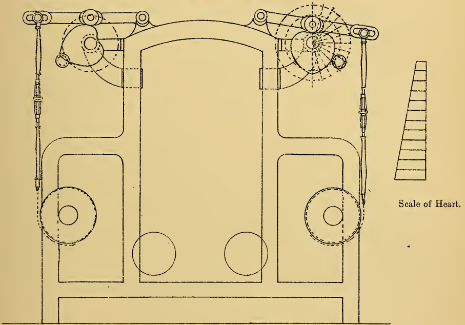
ELEVATION PASS END SHOWING HEART MOTION ARRANGEMENT FOR TRAVERSE OF BOBBIN.
