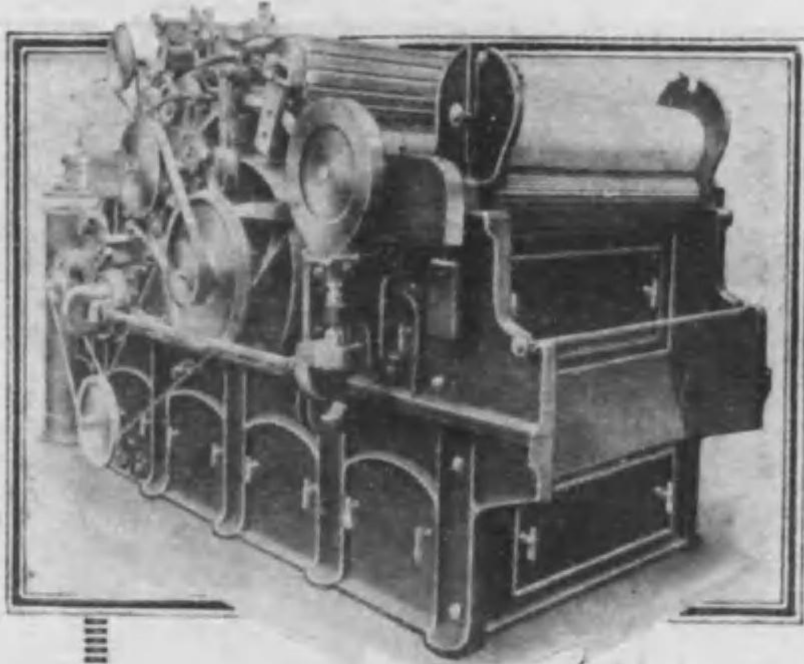
PATENT SIMPLIFIED "shirley" CARDING ENGINE
