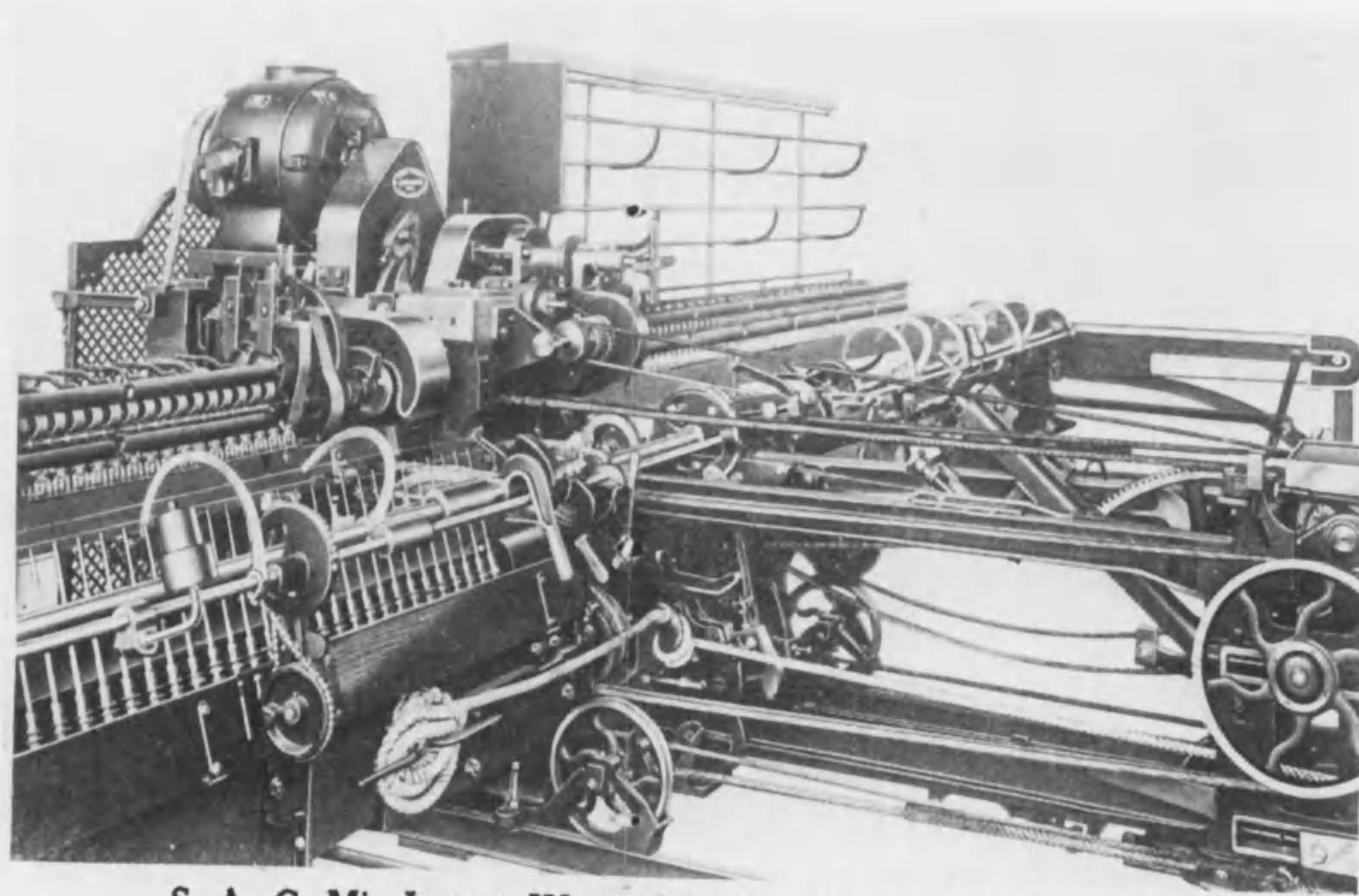
S. A. C. M's Latest Worsted Mule with differential motion
