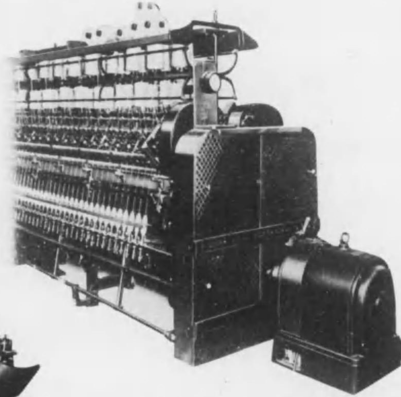
Ring Spinning Frame (woolen), Individual Motor Drive.
