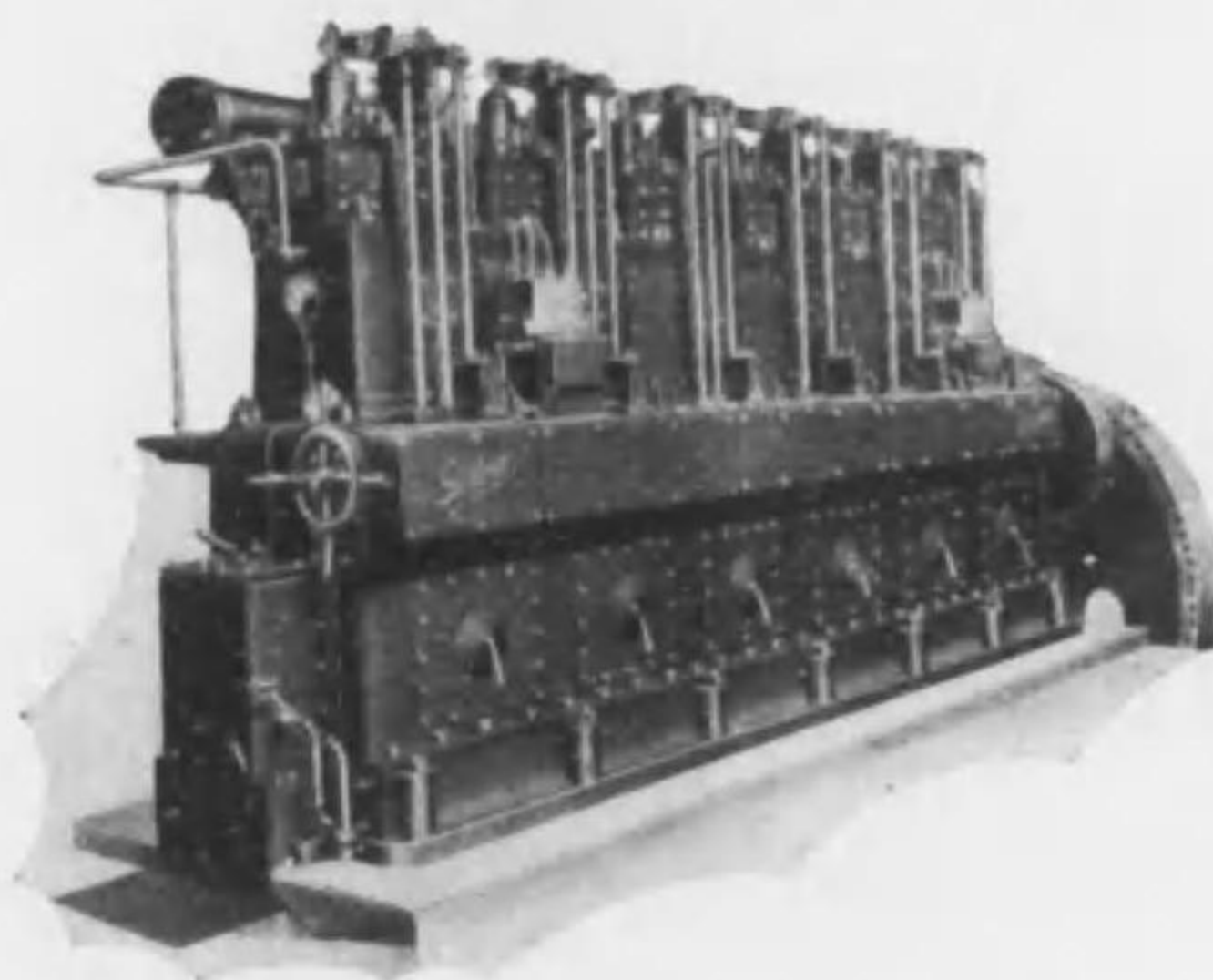
4 Cycles Compressorless Diesel Engine, (50-1,200 B.H.P.)
