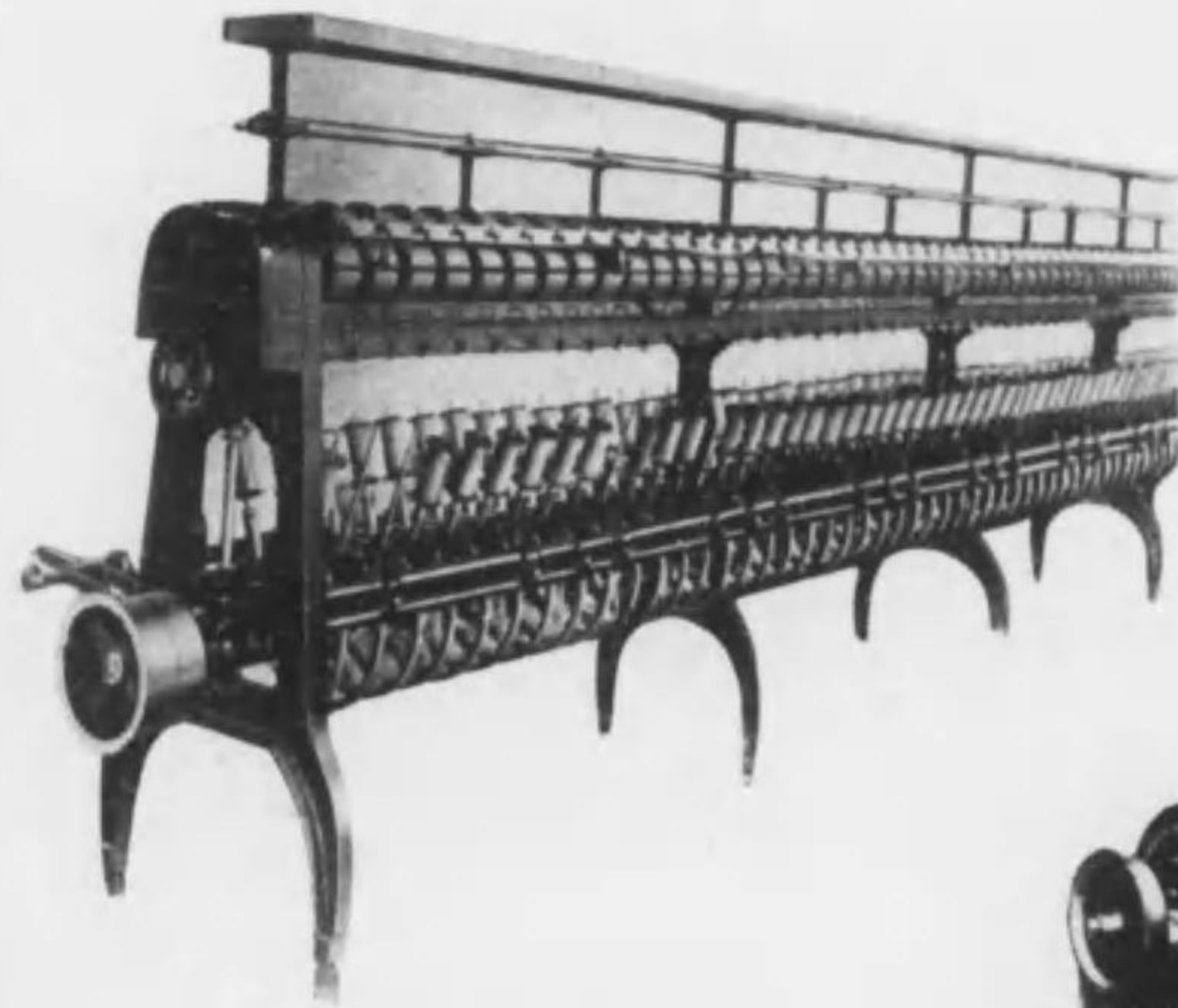
Super High Speed, Twisting Frame, (Silk Yarn)
