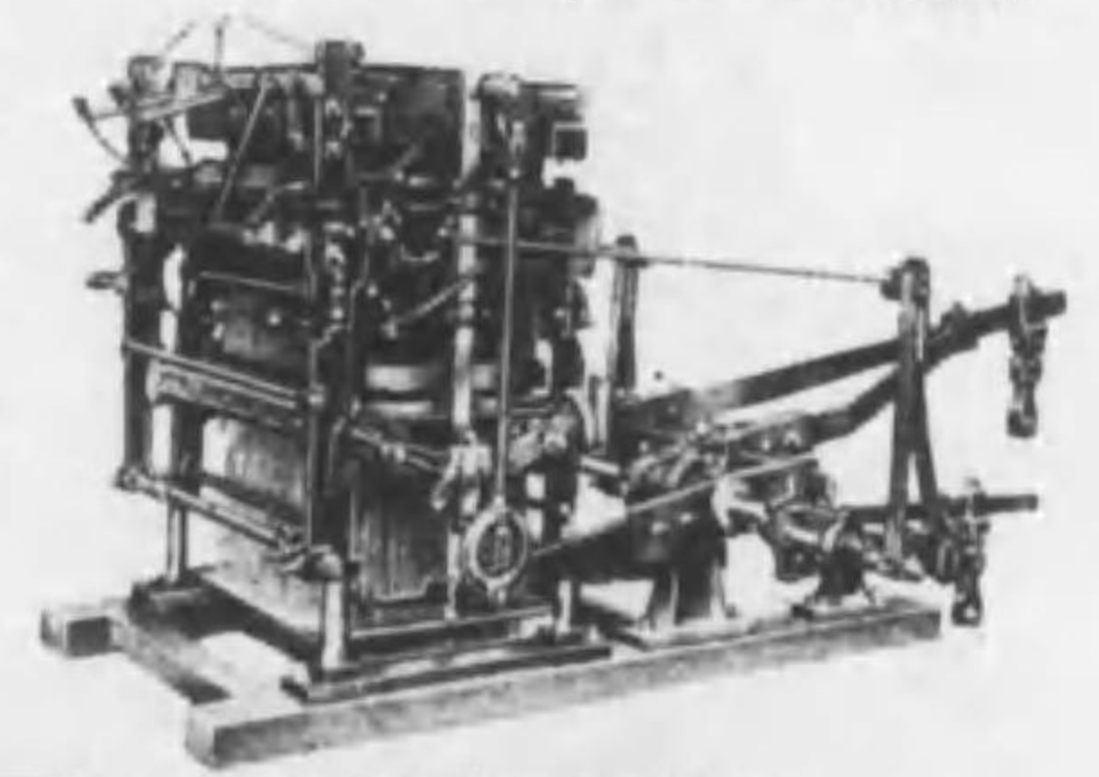
A. Model, Single Lift, Center Shed Jacquard Machine.
