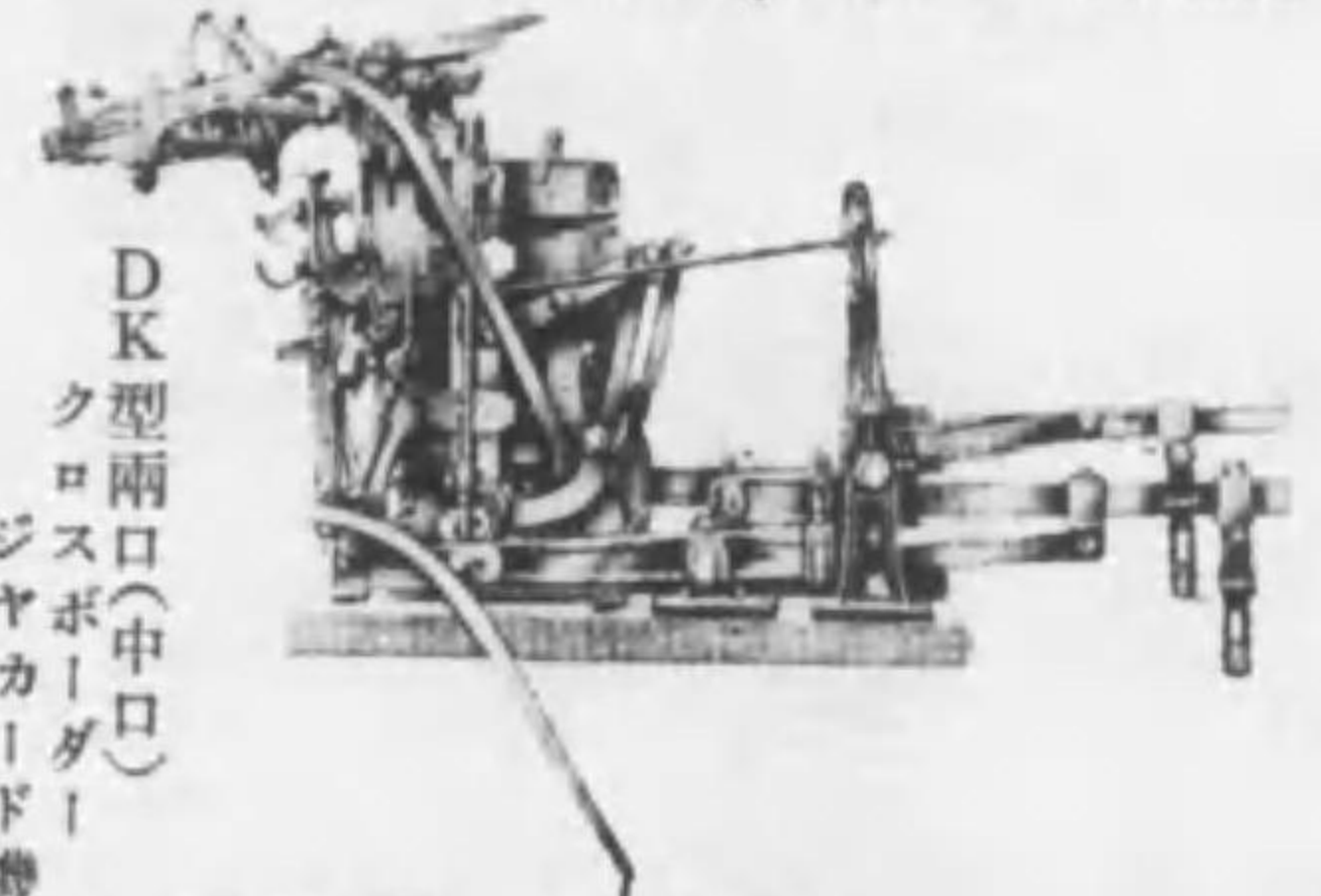
D. K. Model, Single Lift, Cross Boarder Jacquard Machine.
