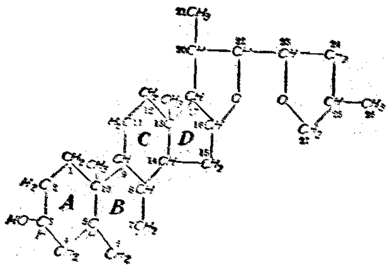
(III) Tigogenin
