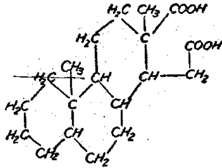
(VI) Aetioallobiliansaeure
