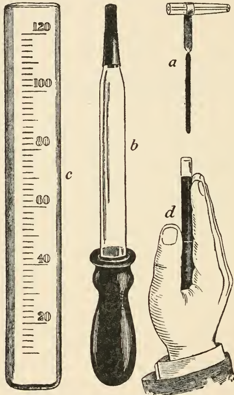
FIG. 8.—THE HÆMACYTOMETER.
