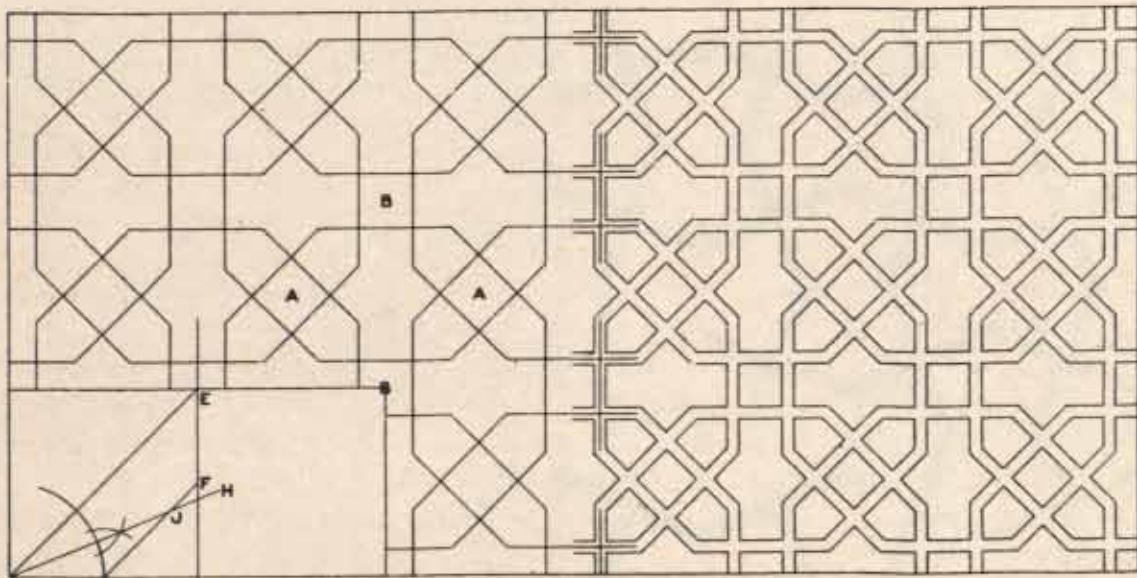
Pattern of trellis screen in a window of the Daftar Khana, Fathpur-Sikri.
