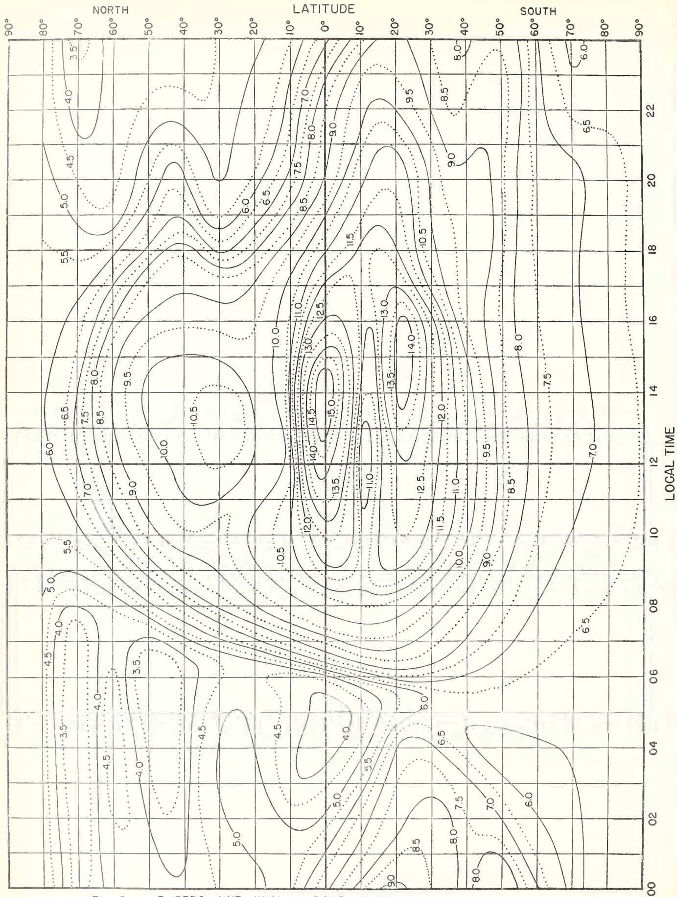
Fig. 5. F_2 ZERO-MUF, IN Mc, W ZONE, PREDICTED FOR JANUARY, 1947.
