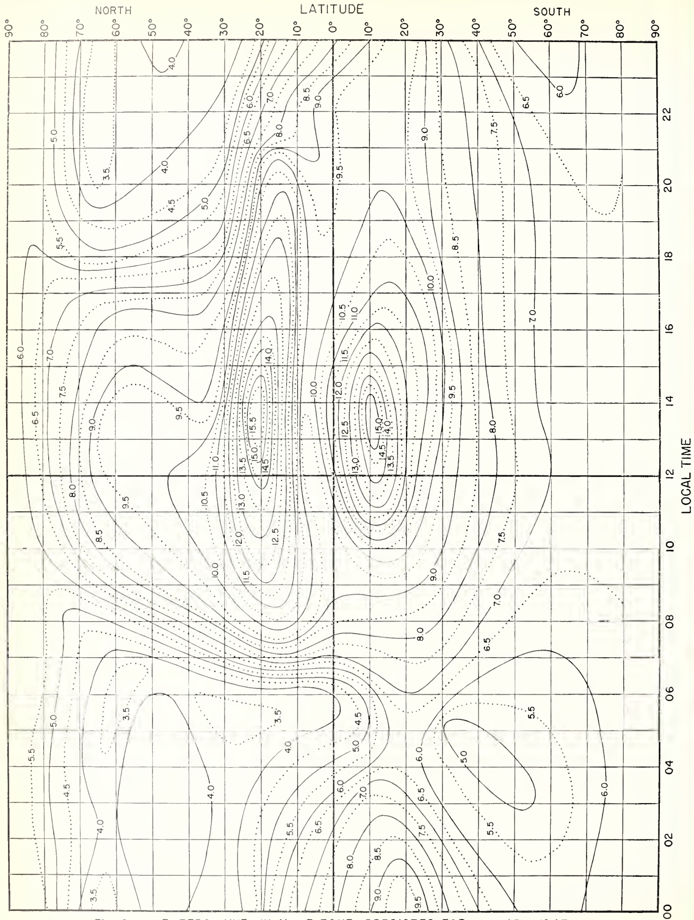
Fig. 9. F_2 ZERO-MUF, IN Mc, E ZONE, PREDICTED FOR JANUARY, 1947.
