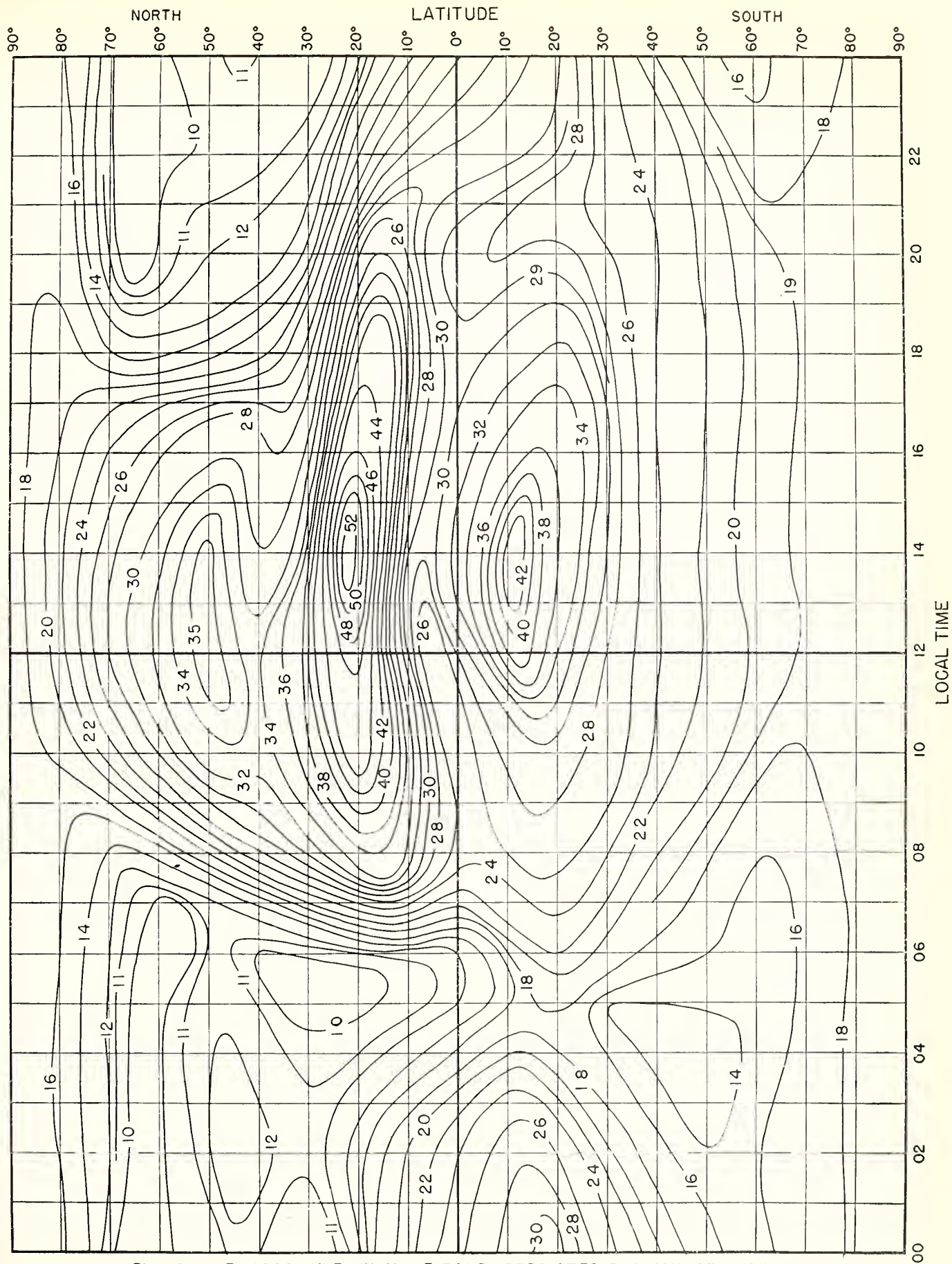
Fig. 10. F 2 4000-MUF, IN Mc, E ZONE, PREDICTED FOR JANUARY, 1947.
