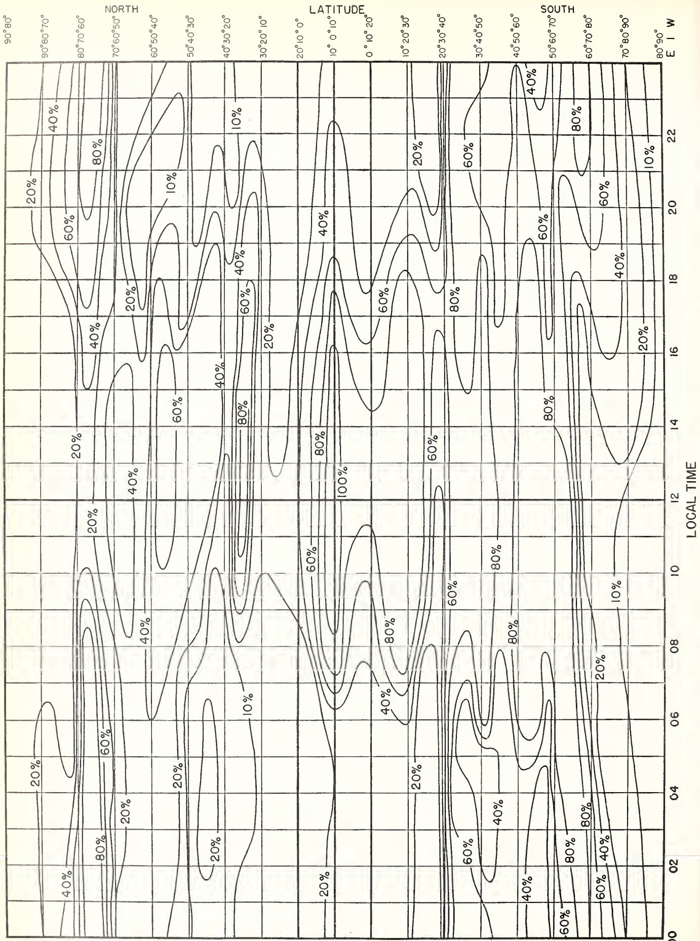
Fig. 15. PERCENTAGE OF TIME OCCURRENCE FOR E_s 2000-MUF IN EXCESS OF 15 Mc, PREDICTED FOR JANUARY, 1947
