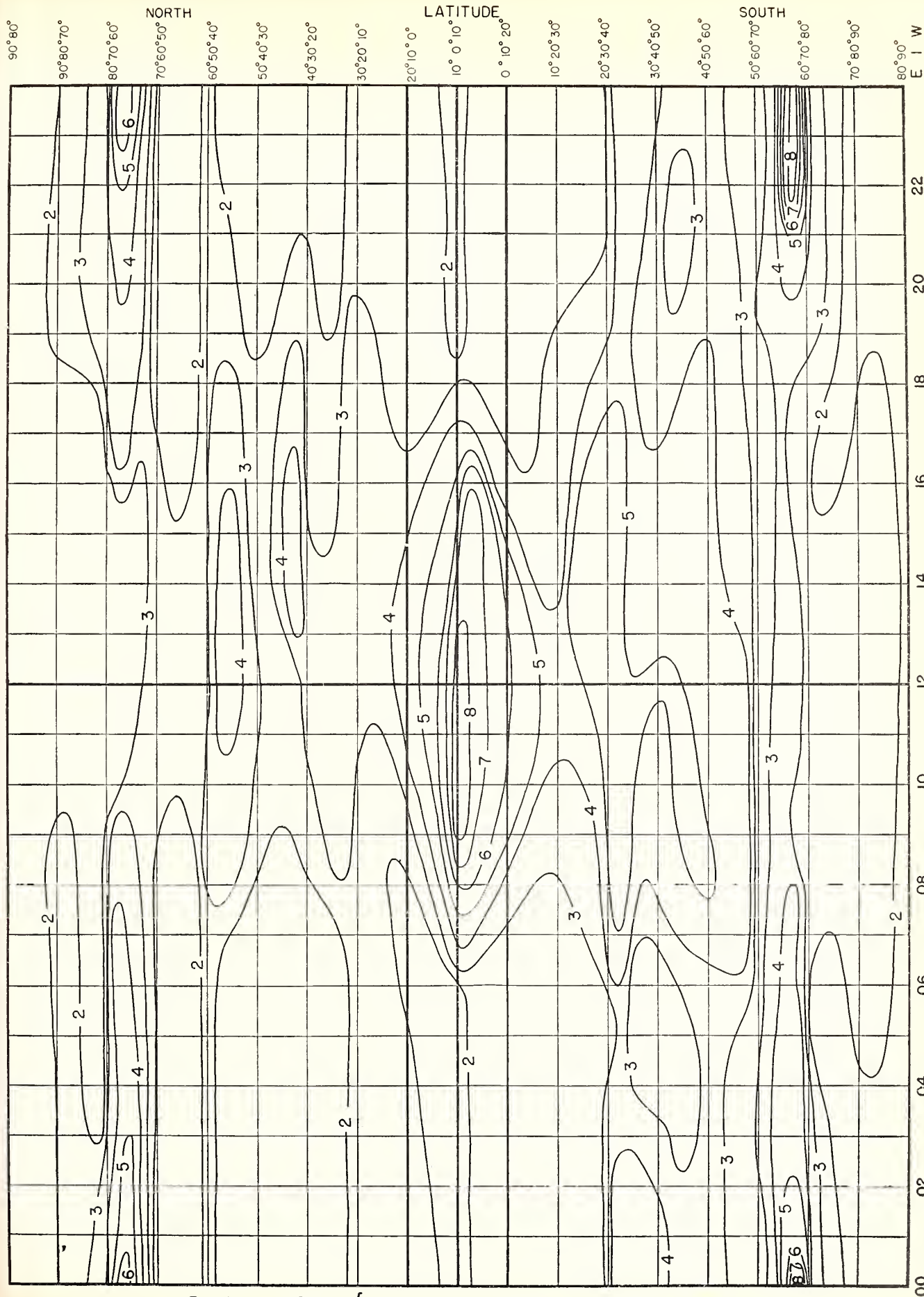
Fig. 12. MEDIAN fE_s , IN Mc, PREDICTED FOR JANUARY, 1947
