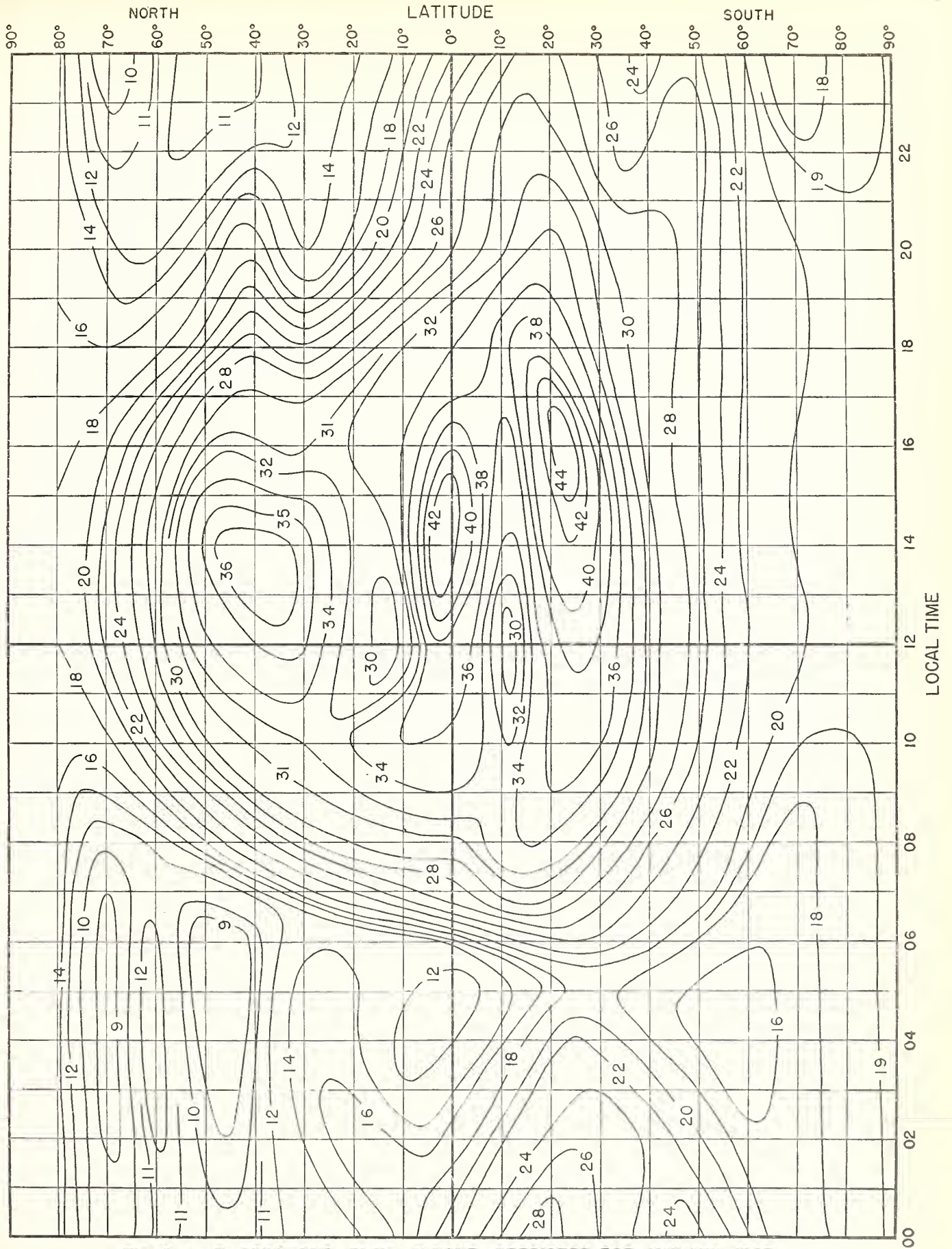
Fig. 6. F_2 4000-MUF, IN Mc, W ZONE, PREDICTED FOR JANUARY, 1947.
