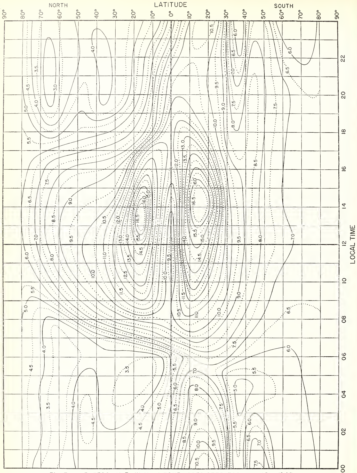
Fig. 7. F_2 ZERO-MUF, IN Mc, I ZONE, PREDICTED FOR JANUARY, 1947.
