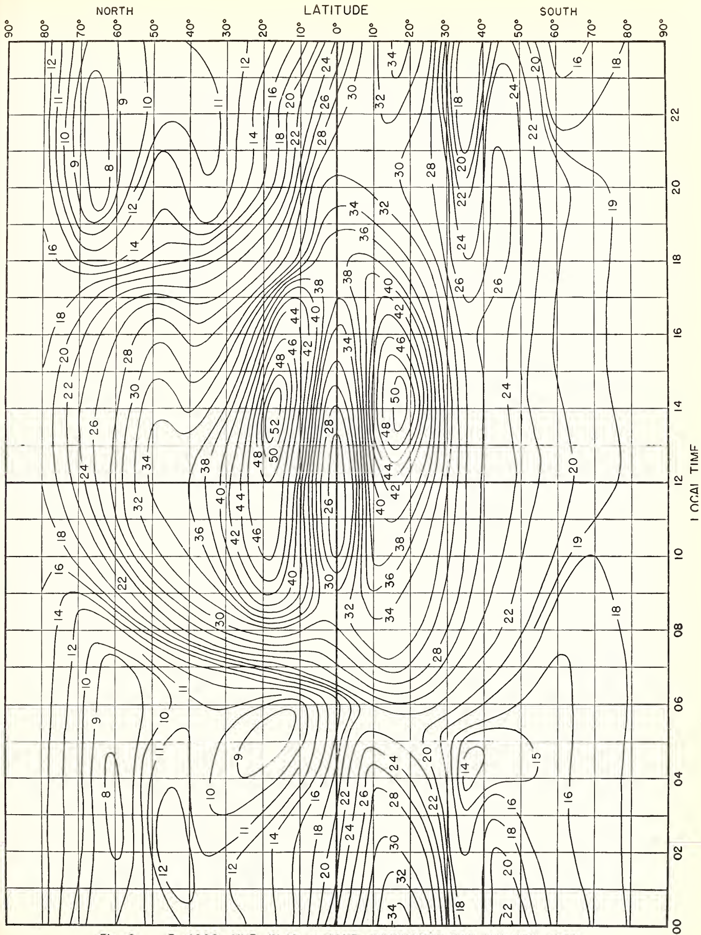
Fig. 8. F_2 4000-MUF, IN Mc, I ZONE, PREDICTED FOR JANUARY, 1947.
