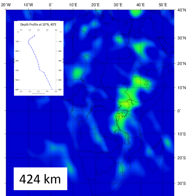
Africa.ANT.Emry-etal.2018 (Vs km/s) – 424 km
