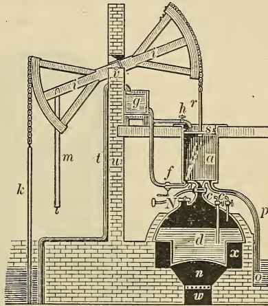
FIG. 159. NEWCOMEN'S STEAM ENGINE
