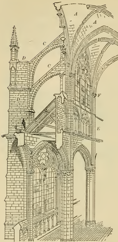
FIG. 58. CROSS SECTION OF AMIENS CATHEDRAL
