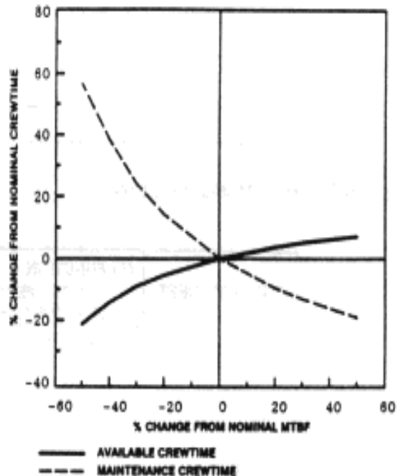
Figure B-12 — Effect of MTBF on Crew Time.
