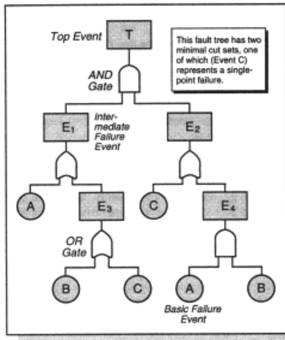
Figure 30 — A Simple Fault Tree.
