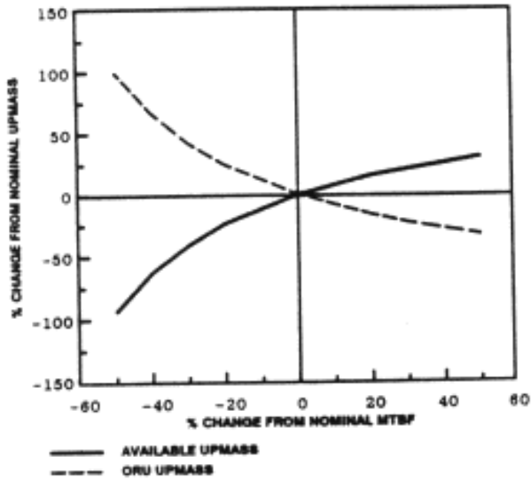
Figure B-13 — Effect of MTBF on Upmass.
