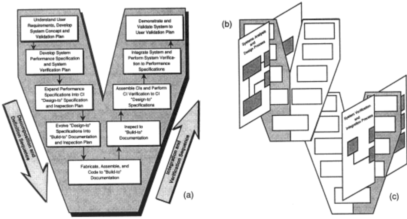
Figure 7 — Overview of the Technical Aspect of the NASA Project Cycle.
