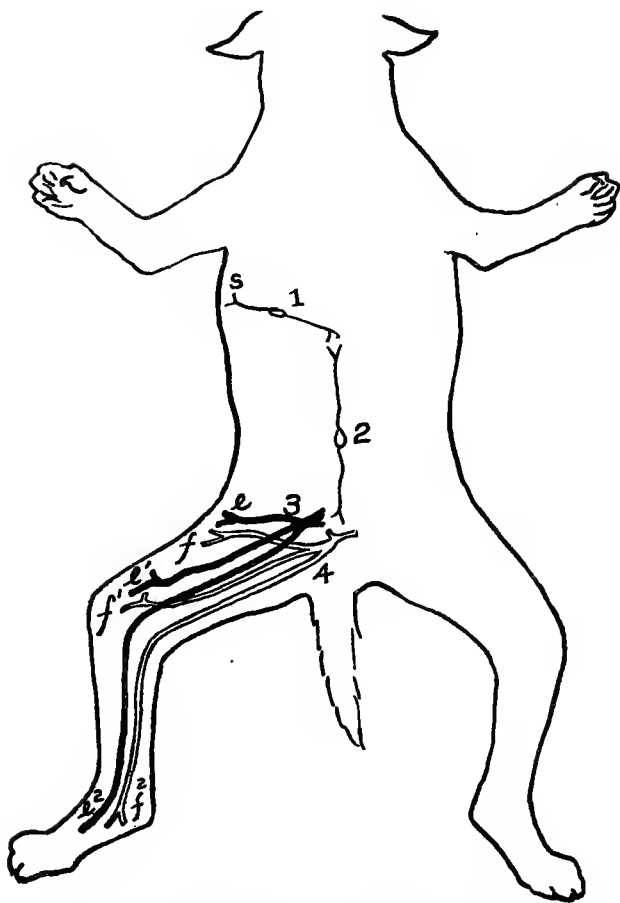
DIAGRAM ILLUSTRATING SCRATCH-REFLEX IN DOG
