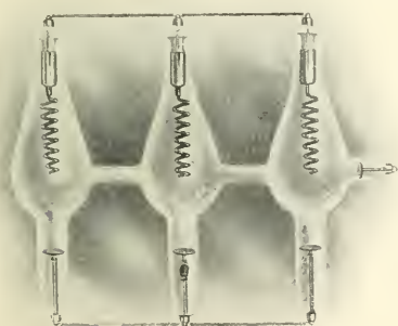
FIG. 194.—Triple valve tube (C. Andrews).
