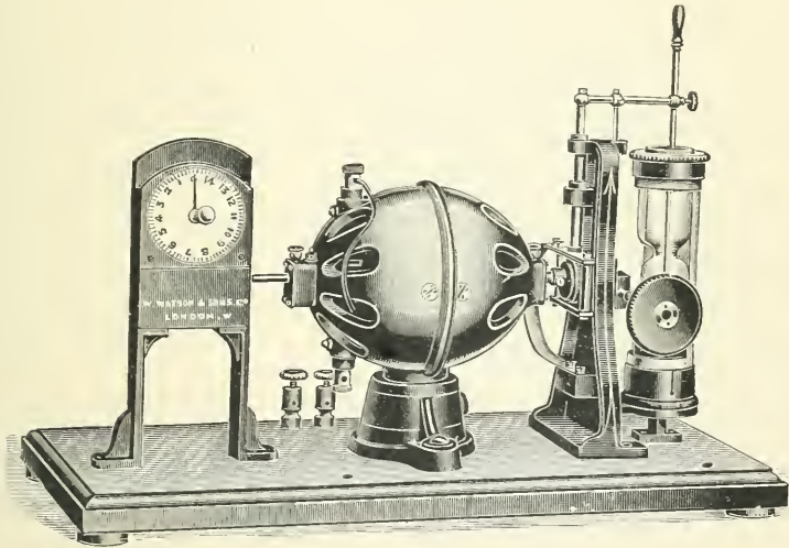
FIG. 191.—Dipping interrupter with revolution counter or tachymeter.
