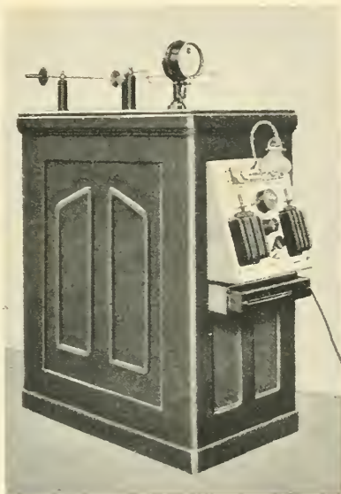
FIG. 2.—Alternating current high-tension rectifier. (Siemens.)
