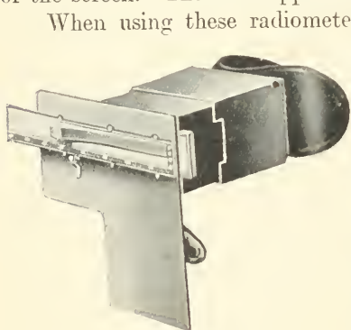
FIG. 59.—Welmelt's crypto-radiometer. (Siemens.)
