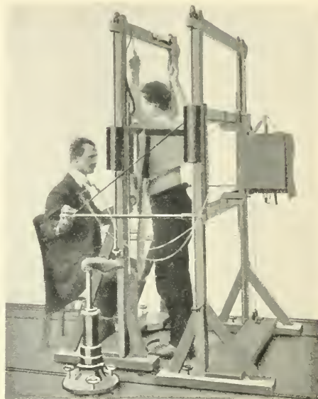
FIG. 75.—Wenckebach screening stand. (Siemens.)
