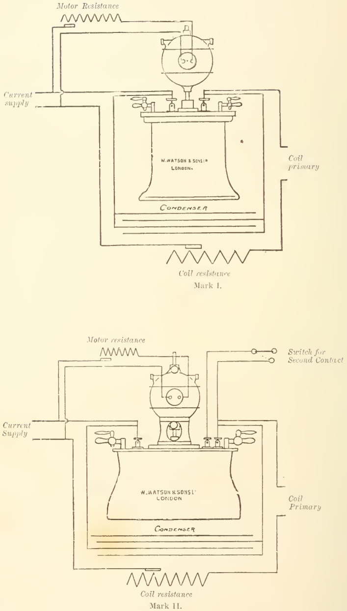
FIG. 13.—Plan of connections for Dreadnought interrupter.
