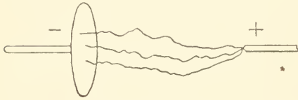
FIG. 36.—Connections of the X-ray tube to the coil, showing the route travelled by the spark when the point is the positive pole and the negative the plate.
