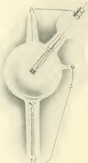
FIG. 28.—Water-cooled tube arranged for overhead work. (C. Andrews.)
