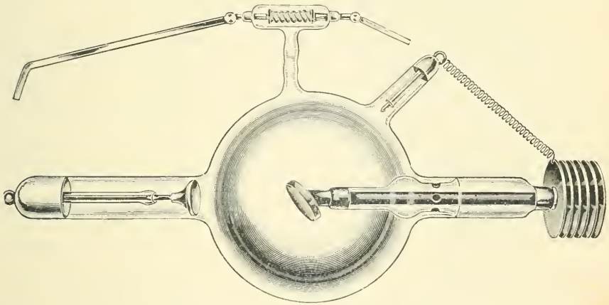
FIG. 26.—Radiator tube constructed for heavy discharges. (Cossar.)
