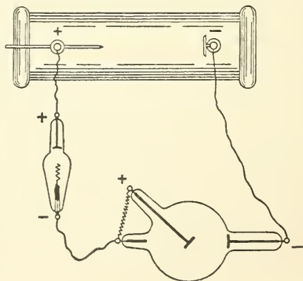
FIG. 39.—Connection of the X-ray tubes to coil. Valve tube on positive pole.
