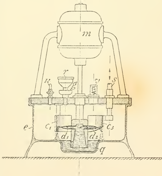
FIG. 12.—Diagram to illustrate construction of a centrifugal mercury interrupter. (Siemens.)
