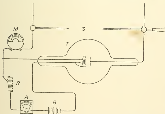
FIG. 35.—Diagram of connections for Coolidge tube.
