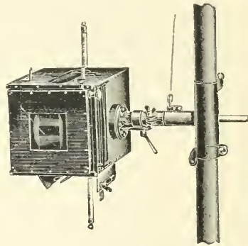
FIG. 65.—Tube-box with rectangular diaphragm.
