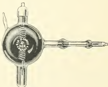
FIG. 47.—Oliver Lodge valve tube. (Cossar.)
