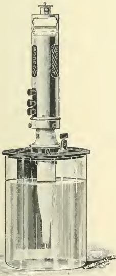
FIG. 21.—Single-point electrolytic interrupter. (Watson.)
