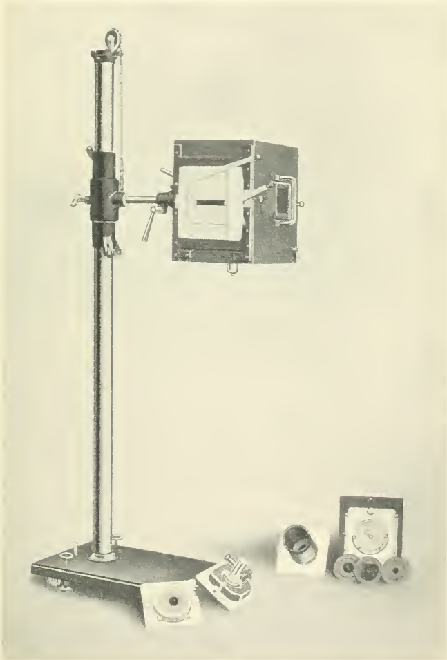
FIG. 61.—Pillar stand, protected tube-box and accessories. (Siemens.)
