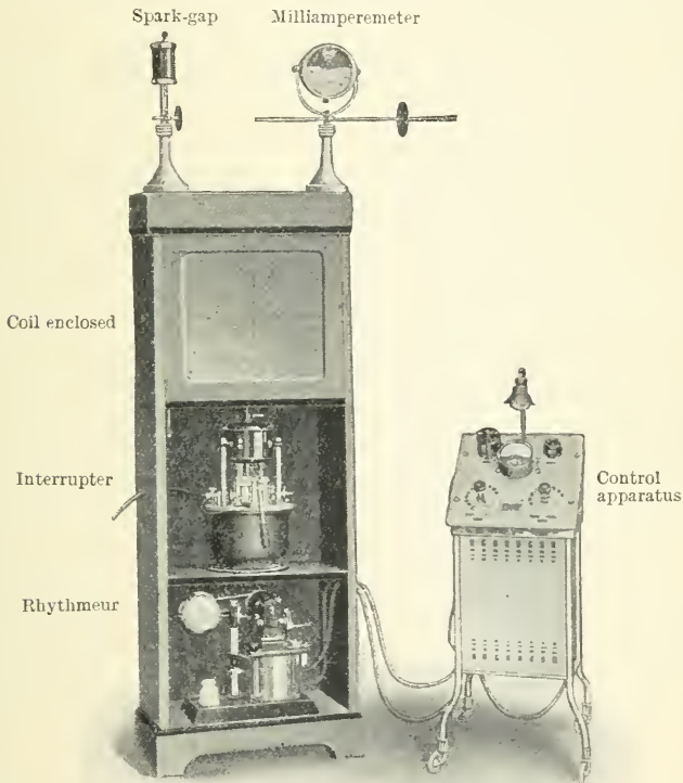
FIG. 188.—Therapeutic outfit suitable for deep therapy. (Schall.)
