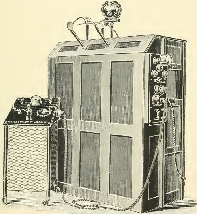
FIG. 4.—Snook apparatus. (Newton and Wright.)
