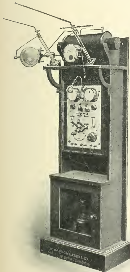
FIG. 199.—Apparatus arranged on an upright cabinet. FIG. 200.—Diagram to show arrangement of apparatus on an upright cabinet.
