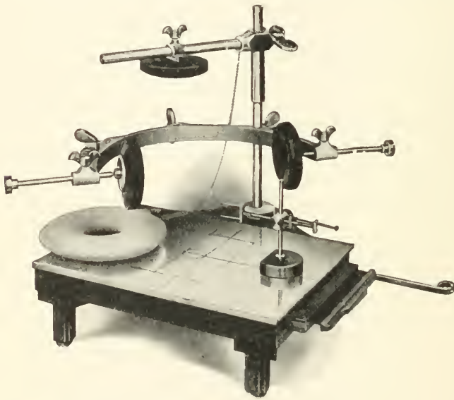
FIG. 104.—Sweet localiser.
