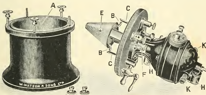
FIG. 15.—Dreadnought interrupter showing detail.
