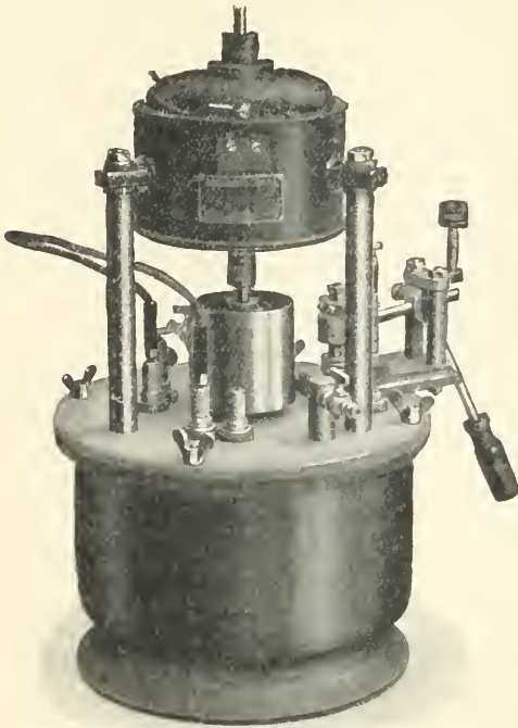
FIG. 189.—Mercury interrupter with gas di-electric. (Schall.)
