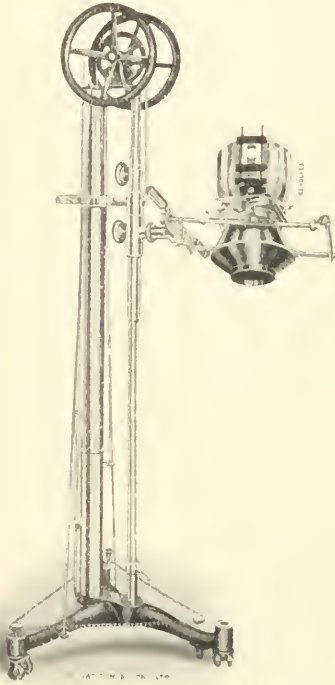
FIG. 62.—A form of tube-stand, which combines many useful mechanical movements. (Watson.)
