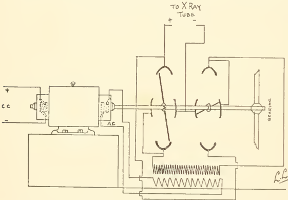
FIG. 5.—Diagram of Snook apparatus. (Newton and Wright.)
