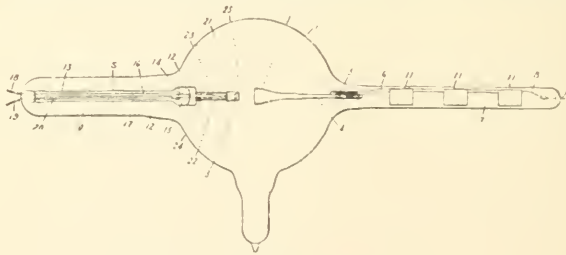
FIG. 33.—Diagram of Coolidge tube.
