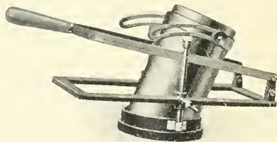
FIG. 69.—Extension tube of a Kidwig compressor to show method of compression. (Siemens.)
