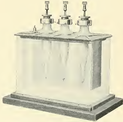
FIG. 20.—Three-point electrolytic interrupter. (Siemens.)
