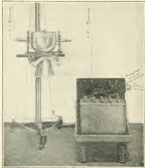
FIG. 34.—Complete Coolidge X-ray equipment in position. (B. T. H.)
