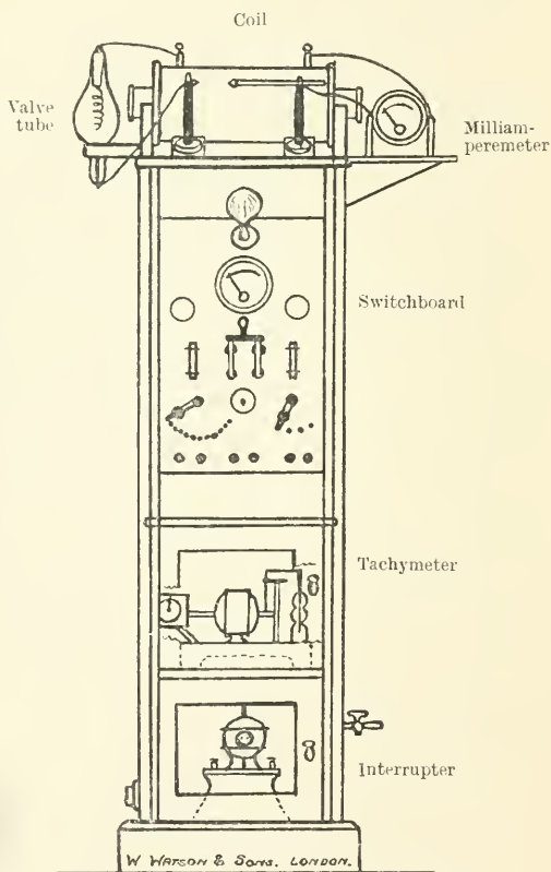
FIG. 199.—Apparatus arranged on an upright cabinet. FIG. 200.—Diagram to show arrangement of apparatus on an upright cabinet.
