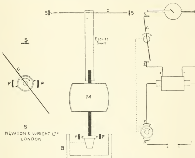
FIG. 193.—Diagram of connections for Morton rectifier.
