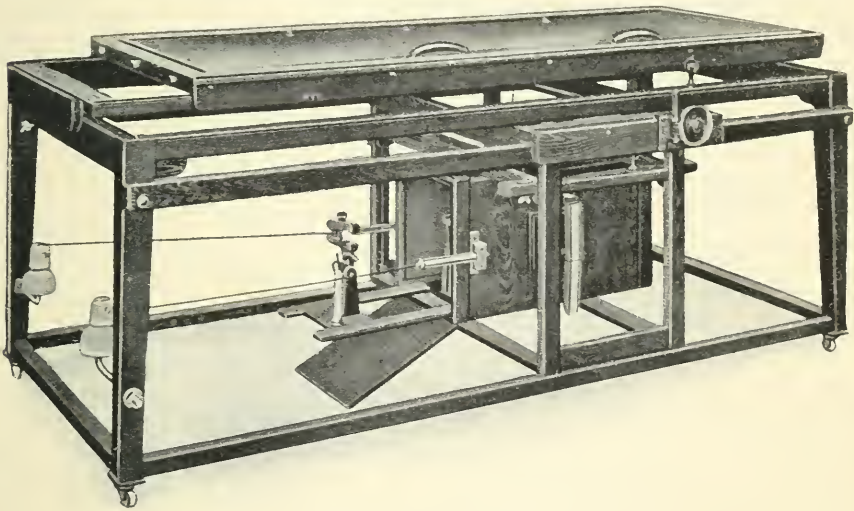
FIG. 66.—A convenient form of X-ray couch. (Siemens.)
