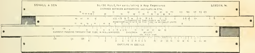
FIG. 85.—Slide rule.
