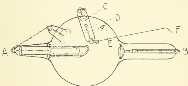
FIG. 40.—Mica regulator. (C. Andrews.)
