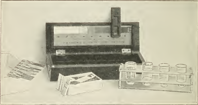
FIG. 201.—Complete Kienböck quantimeter. (Schall.)
