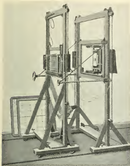
FIG. 74.—Wenckebach screening stand. (Siemens.)
