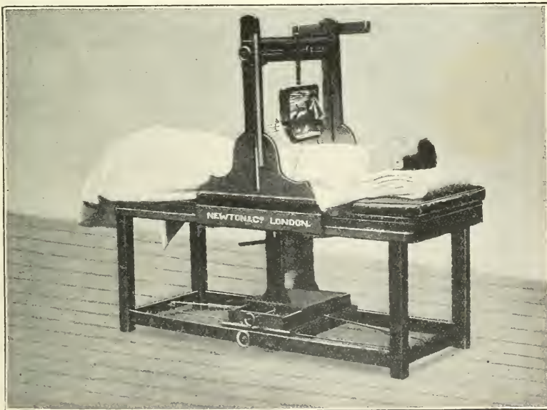
FIG. 180.—X-Ray couch to illustrate method of compression.
