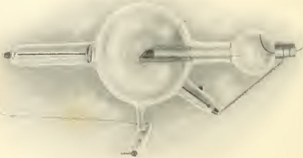
FIG. 29.—Water-cooled tube for overhead or under the couch work, showing mica and carbon regulator. (C. Andrews.)
