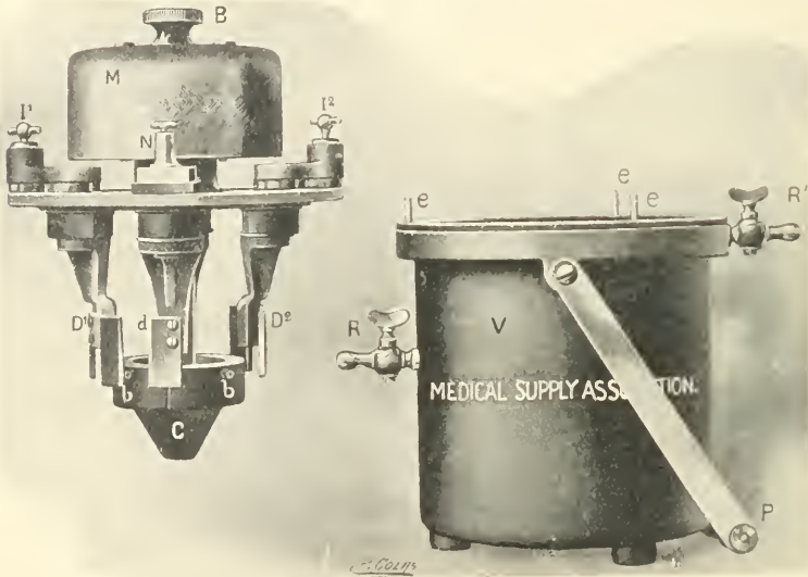
FIG. 24.—Gaiffe interrupter.
