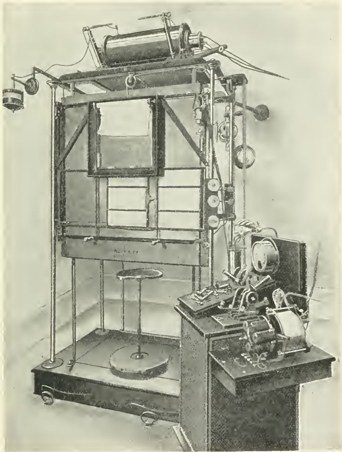
FIG. 153.—Upright screening stand, with automatic stereoscopic movements of tube- and plate-holder controlled from the switch-board. Suitable for taking radiographs of the thorax. (Butt and Co.)
