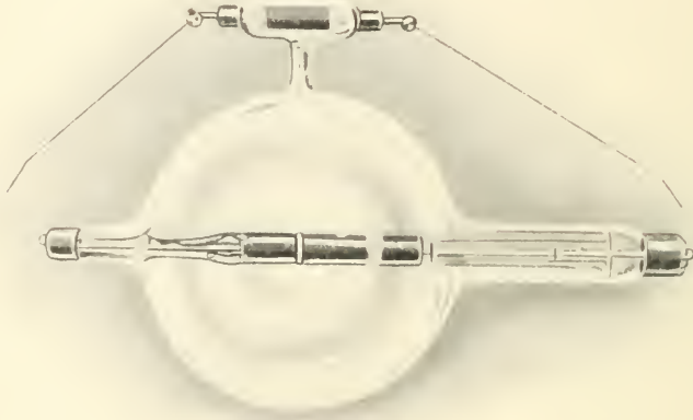
FIG. 48.—Gündelach valve tube. (Siemens.)
