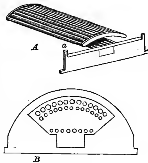
Vertical transverse section of same boiler.
