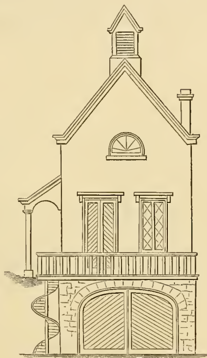
End Elevation.
