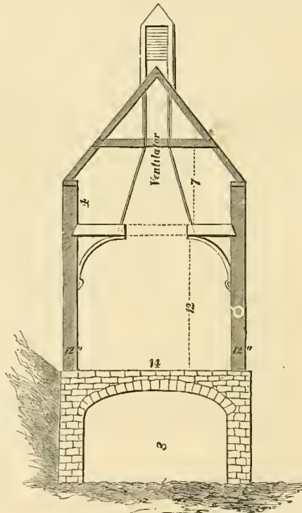
End Section.
