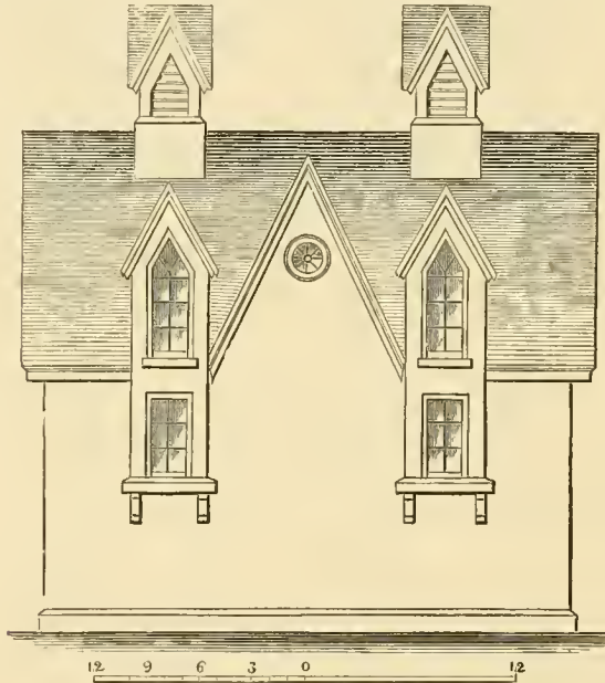
End Elevation.
