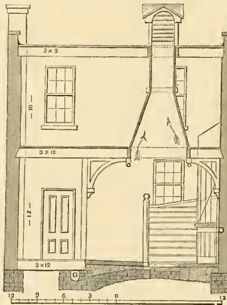
Transverse Section T T on Plan.
