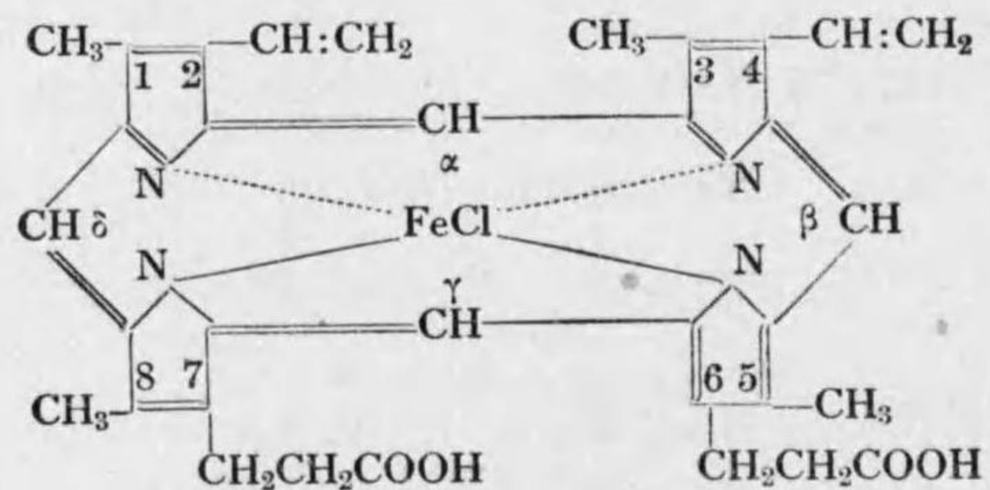
Hemin C 34 H 32 N 4 FeO 4 Cl
