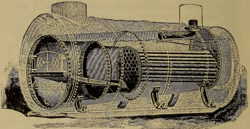
THE MONARCH ECONOMIC BOILER.
