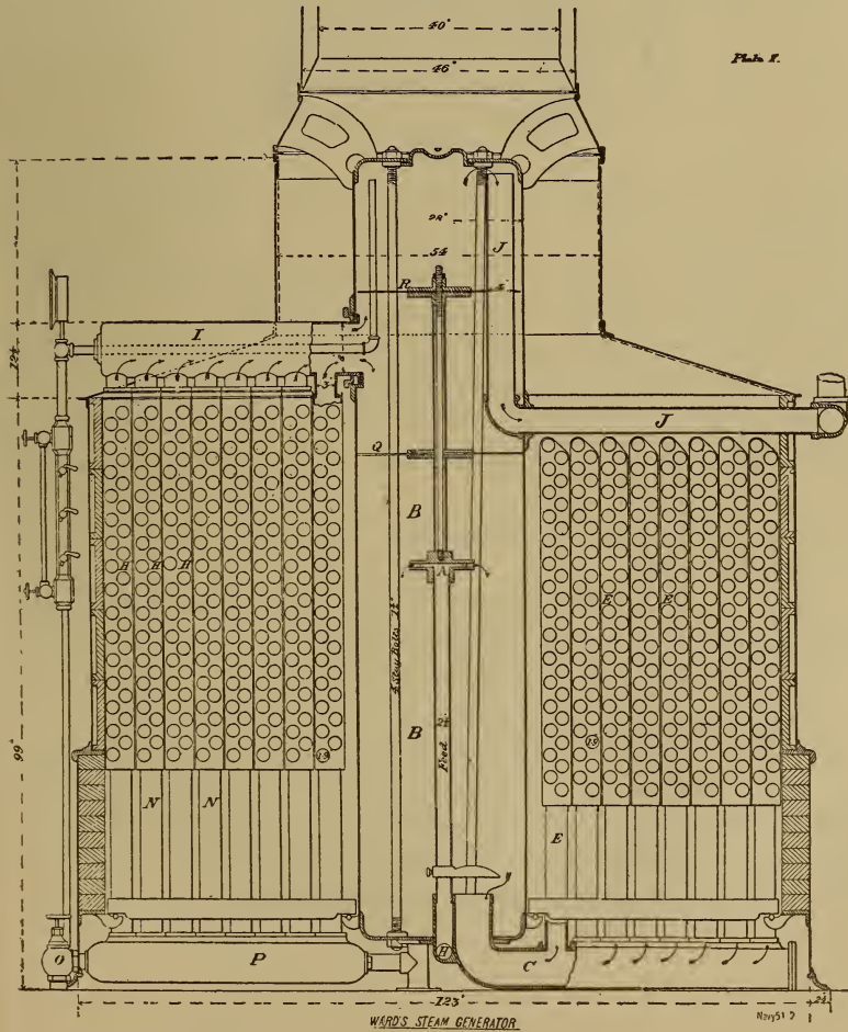
WARD'S STEAM GENERATOR. See P. 30. As Tested by Board of U. S. Naval Engineers.
