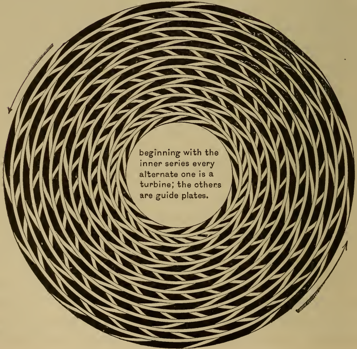
FIG. 44.—SECTION OF DOW TURBINE.
