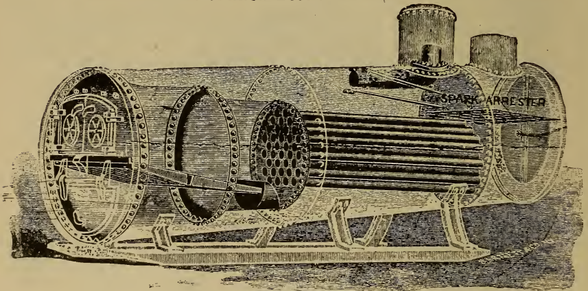
THE MONARCH PORTABLE BOILER.
