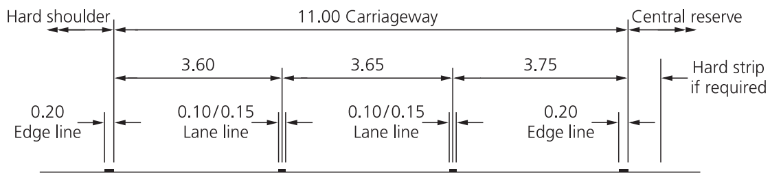
Dual three-lane motorway See table 4-2 for guidance on appropriate line width
