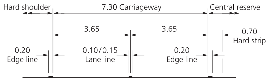
Dual two-lane motorway See table 4-2 for guidance on appropriate line width
