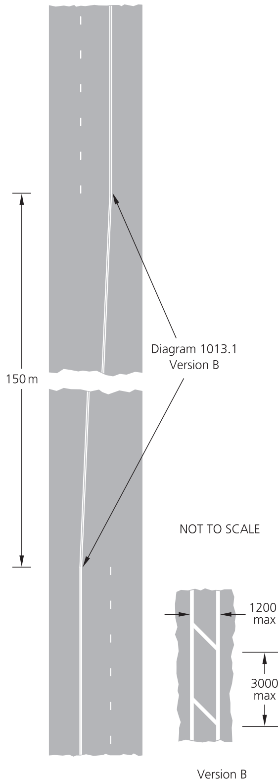
Layout of markings at sag between two climbing lanes
