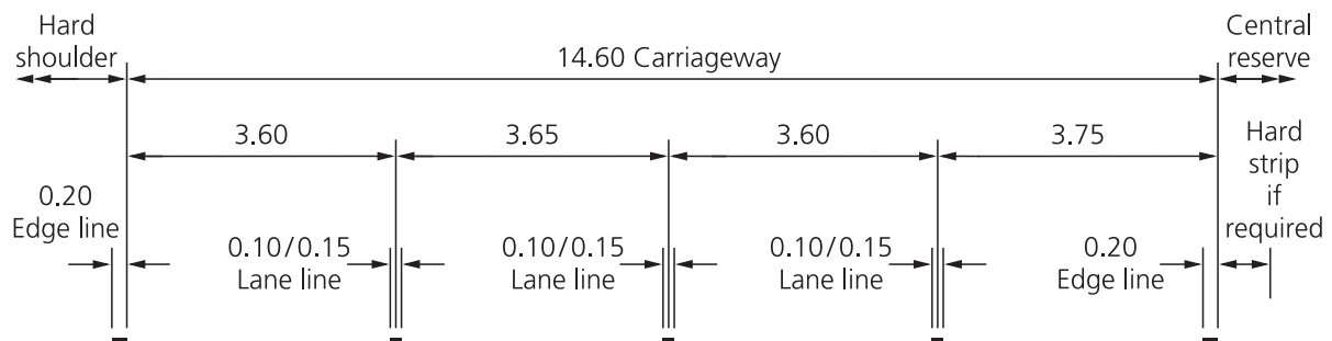
Dual four-lane motorway See table 4-2 for guidance on appropriate line width
