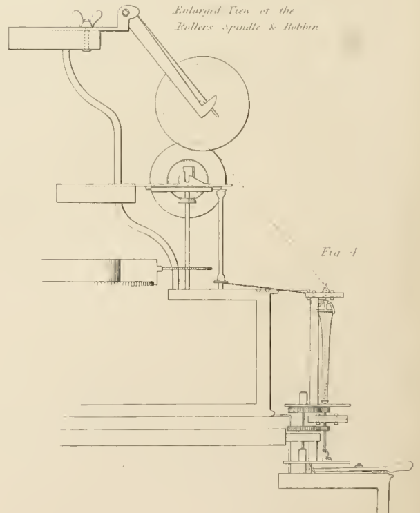
Lewis Pauls Spinning Machine Patent 1758
