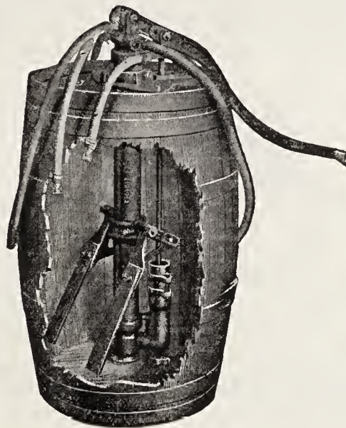
Gould's Pomona Spray Pump.
