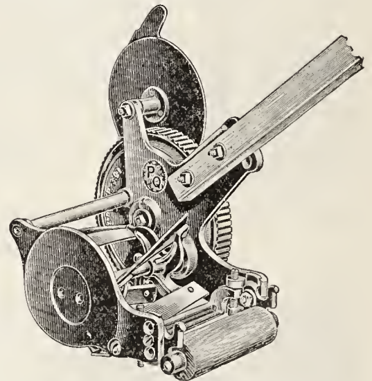
Pennsylvania Combined Trimmer
