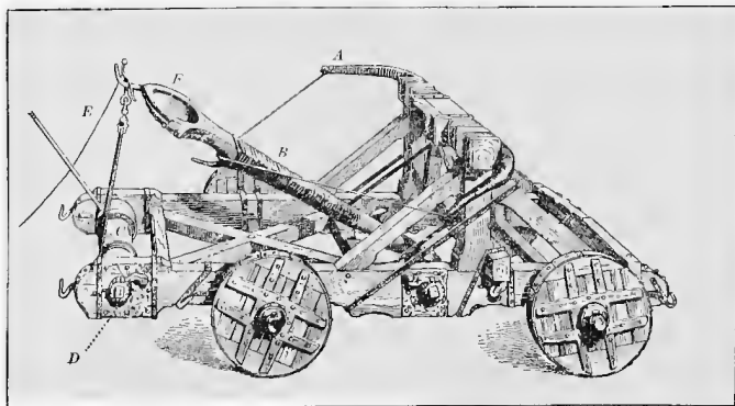
FIG. 153. MACHINE FOR HURLING STONES
