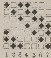
Weave No. 24.
