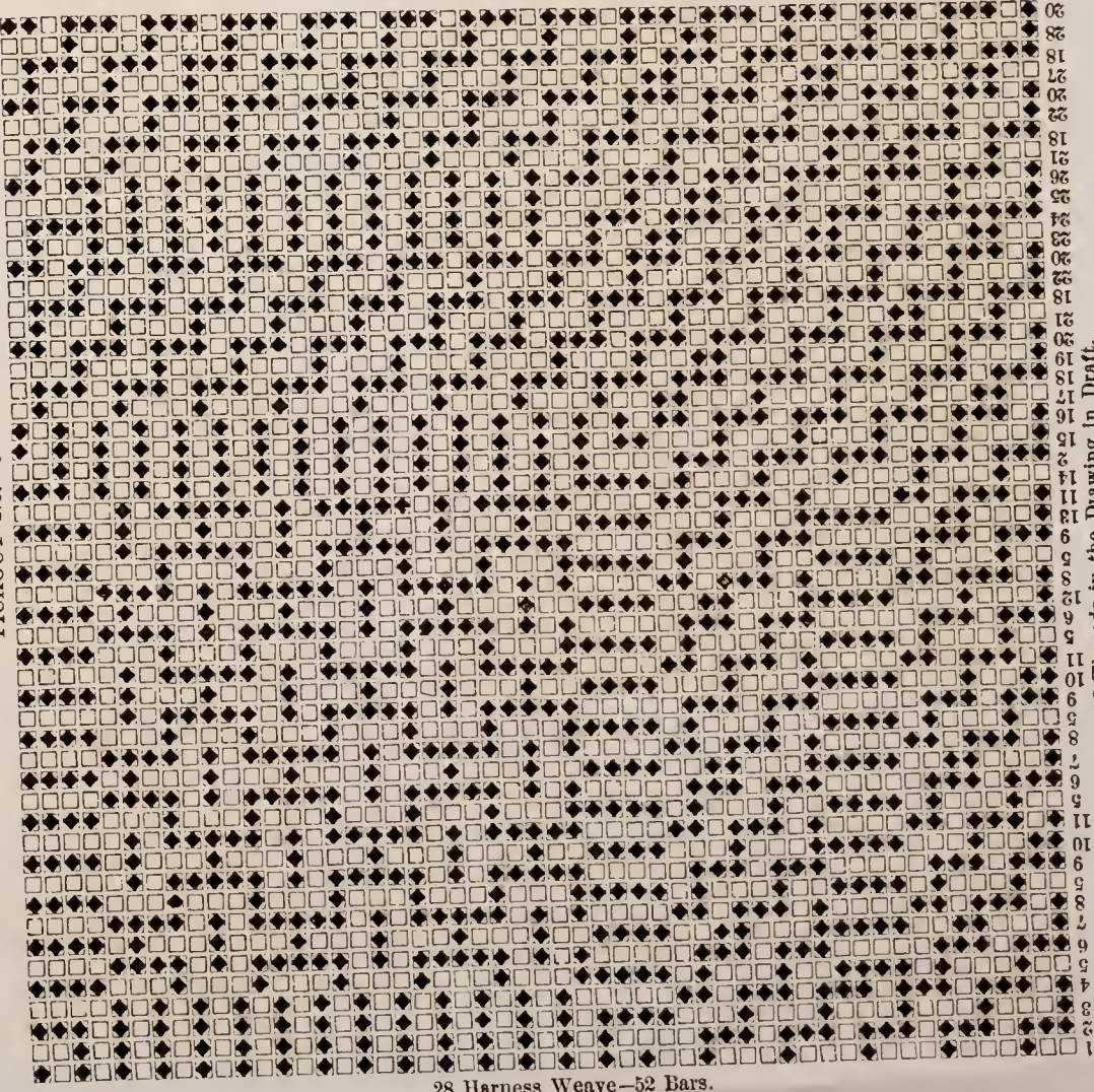
28 Harness Weave—52 Bars. Front.
