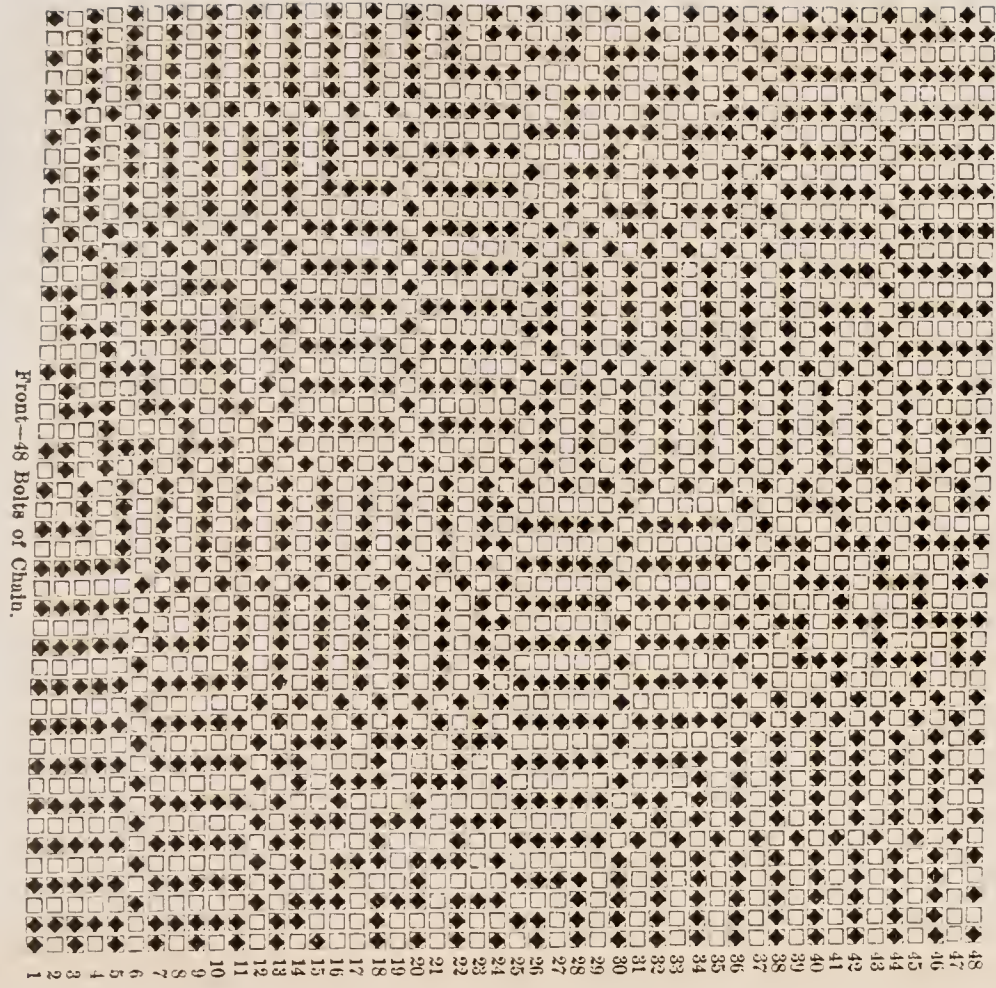
WEAVE No. 82.
