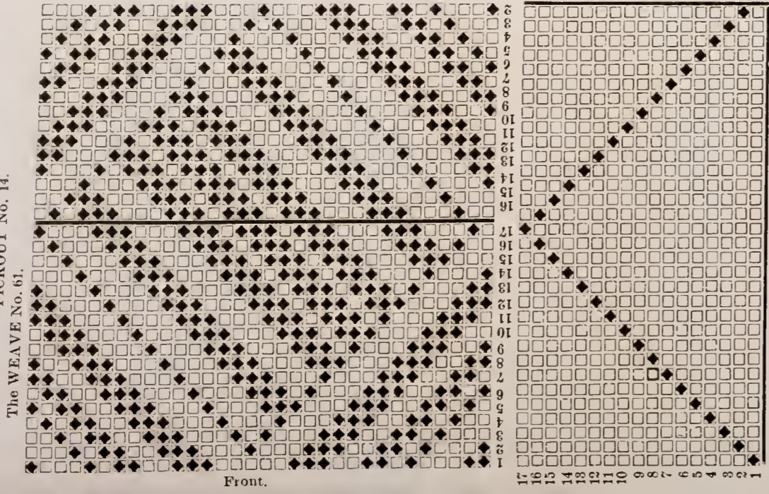
Drawing in Draft.—32 Threads in Pattern.
