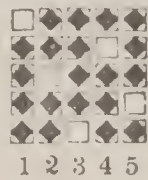
Weave No. 55.
