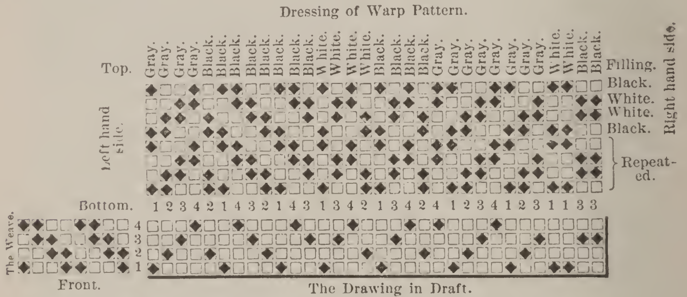
Reading from top to bottom shows the manner each warp thread is woven in. Reading from right to left, shows the manner each filling thread is woven in.
