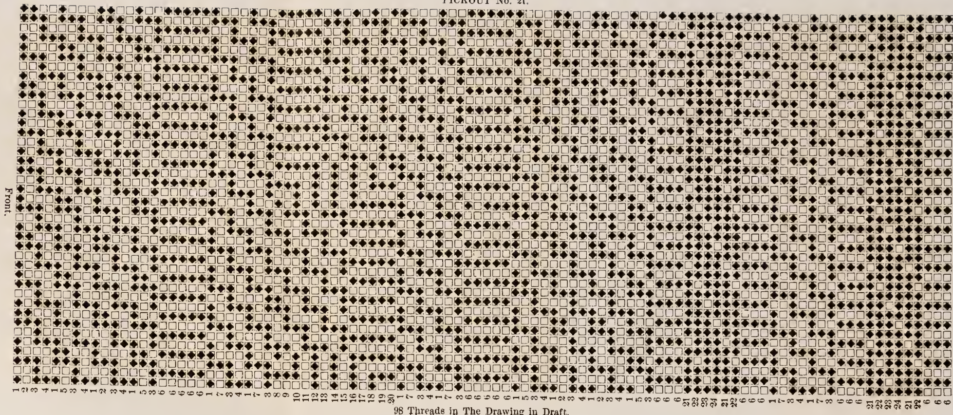
24 harness Weave. 40 Bars.
