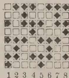
Weave No. 67.
