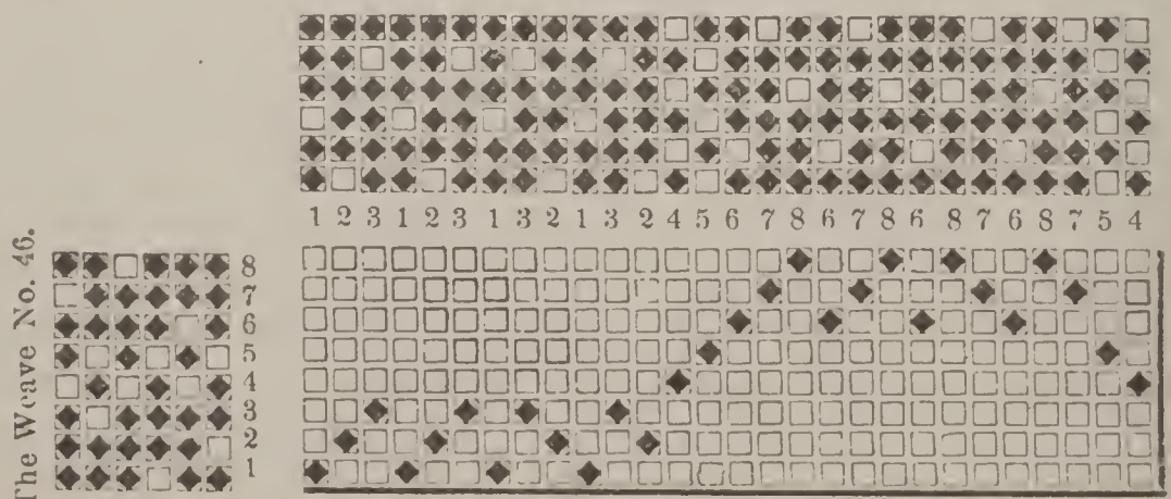
The Drawing in draft, 28 threads in pattern.
