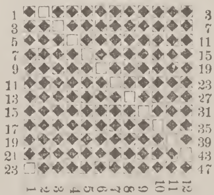
Weave No. 4.
