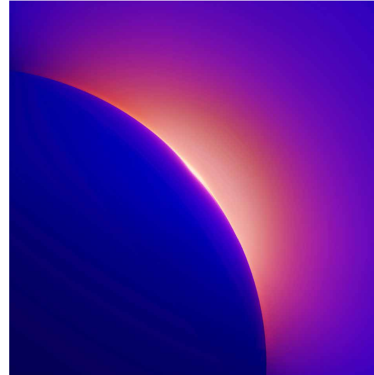
Curvature Extended Artemis_SingleHorizon-Extended_Curvature_Warm
