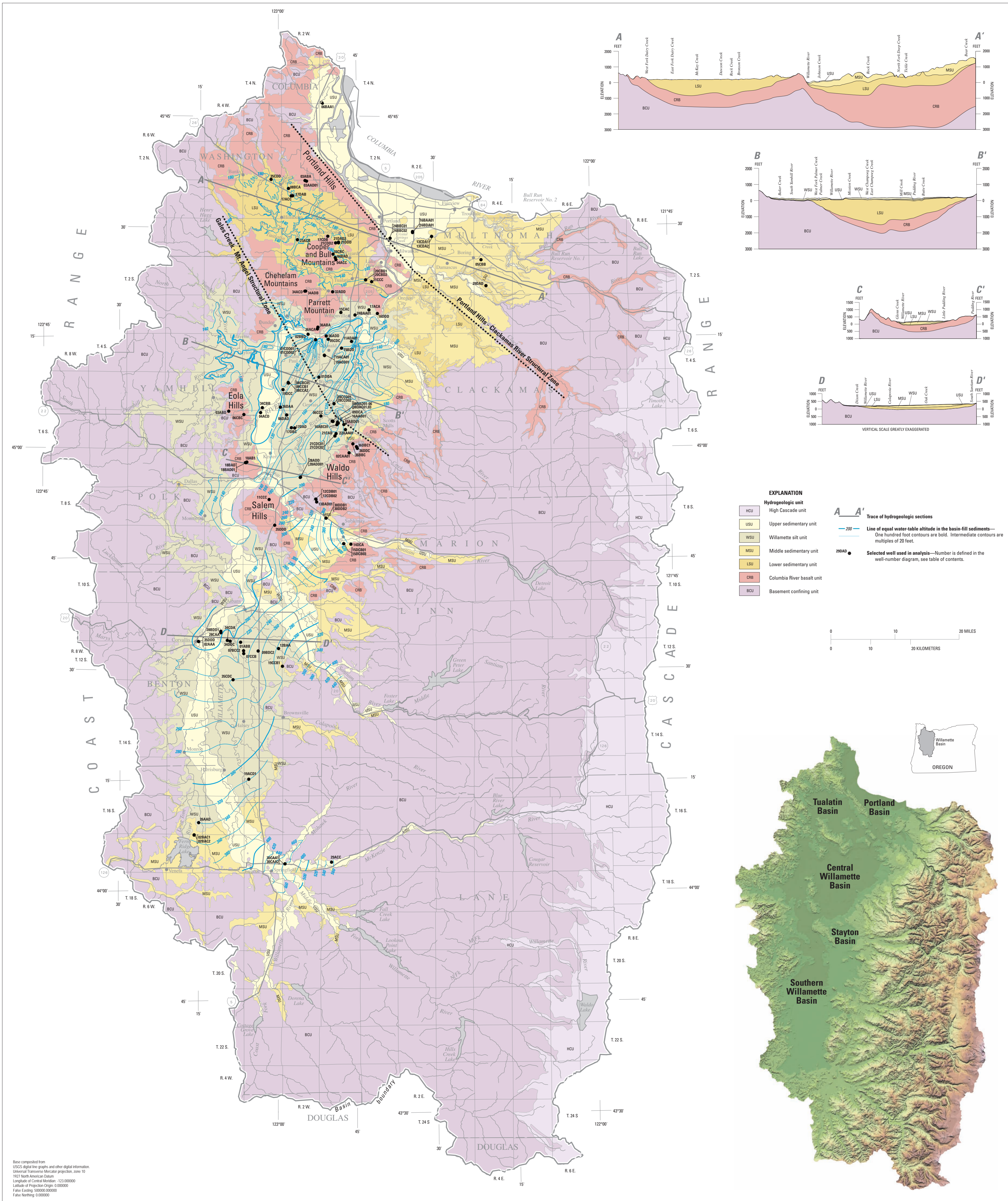
MAP AND CROSS SECTIONS SHOWING THE GENERALIZED HYDROGEOLOGY AND WATER TABLE OF THE WILLAMETTE BASIN AND LOCATIONS OF SELECTED WELLS
