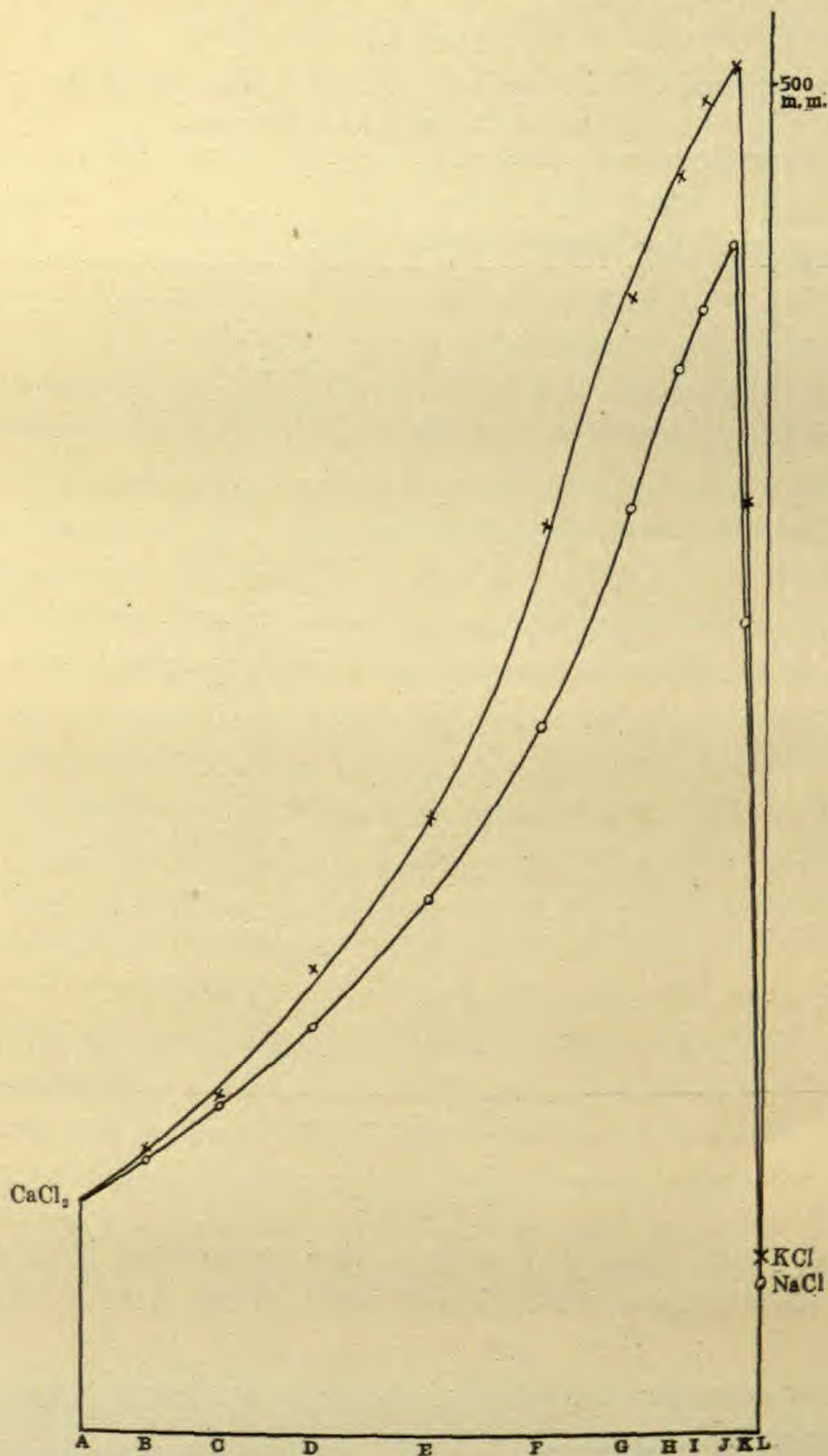
FIG. 4.—Antagonism curve, \text{CaCl}_2 vs. \text{KCl} (upper curve -x-x-x-) and \text{CaCl}_2 vs. \text{NaCl} (lower curve o-o-o). Each ordinate represents the amount of growth of wheat roots in a solution whose composition is given opposite the corresponding letter in table IV.
