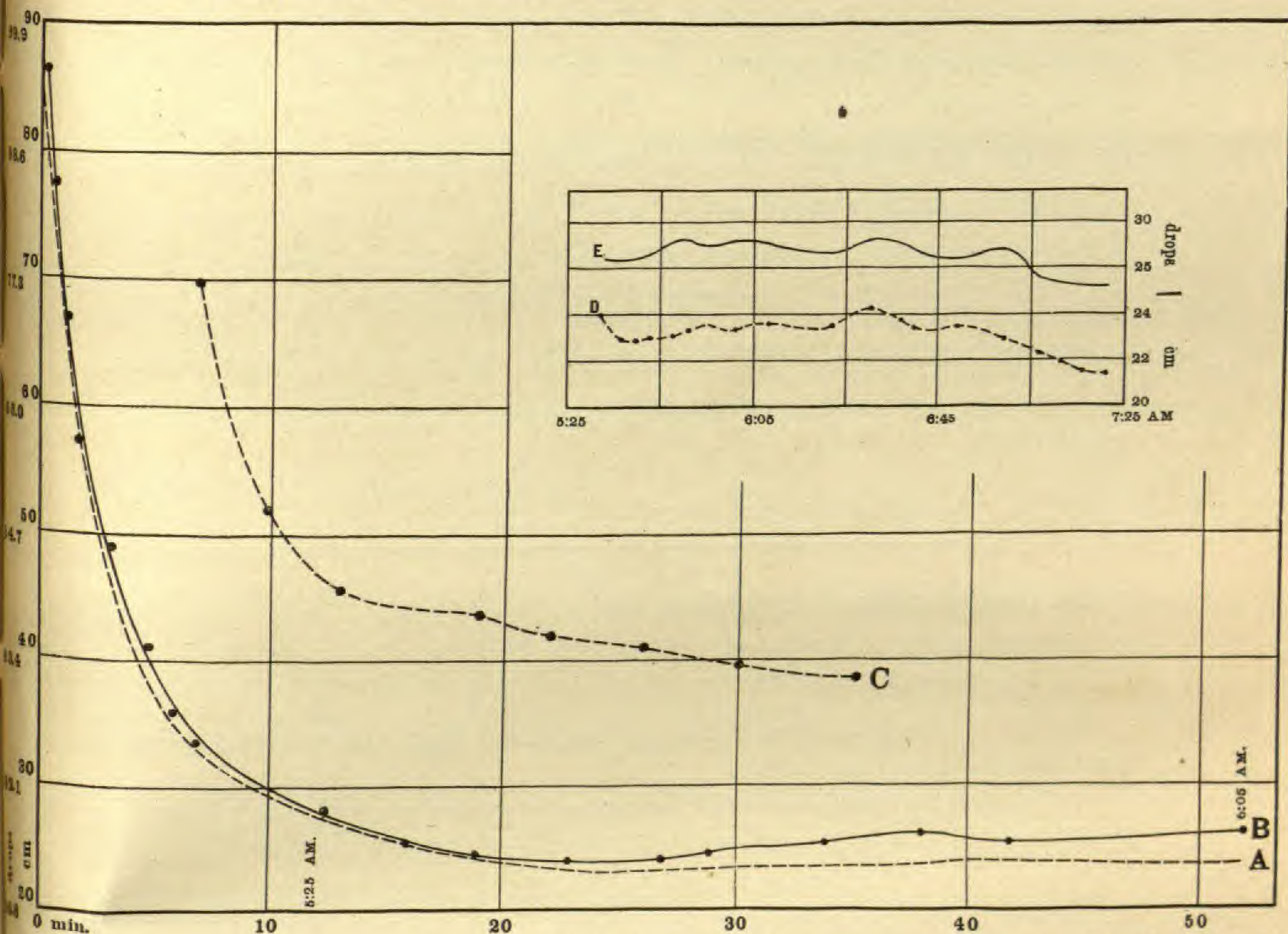
FIG. 5.— A , pressure at the base of a white birch, April 16, 1906, while flow was taking place from a hole higher up; B , rate of flow in drops per minute of the hole above A ; the continuation of curves A and B are D and E ; in another tree the decline of pressure while sap was flowing freely is shown by C .
