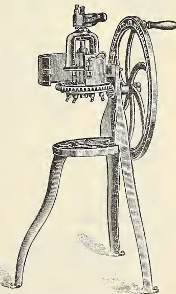
MANN'S GREEN BONE CUTTER, NO. 7
