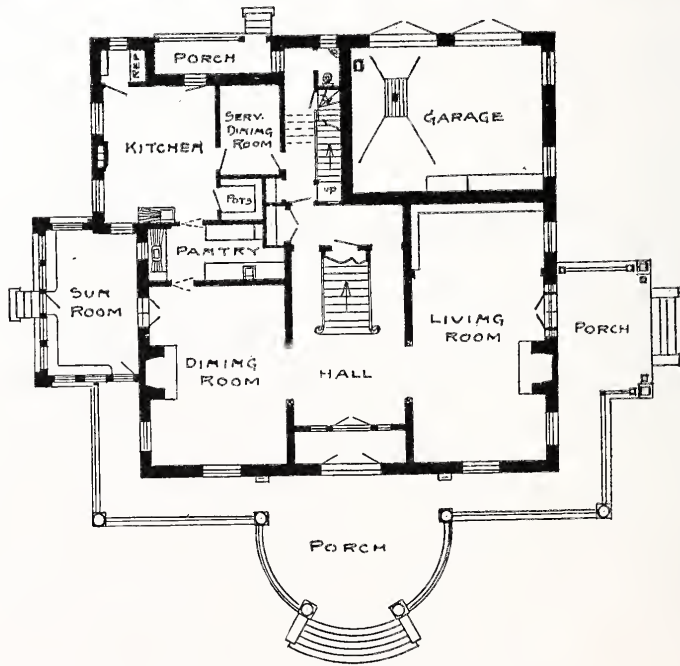
FIG. 28. VIEW AND FIRST FLOOR PLAN. HOUSE OF J. C. FENNEL, ESQ., KANSAS CITY, MO. ROOT & SIEMENS, ARCHITECTS.
