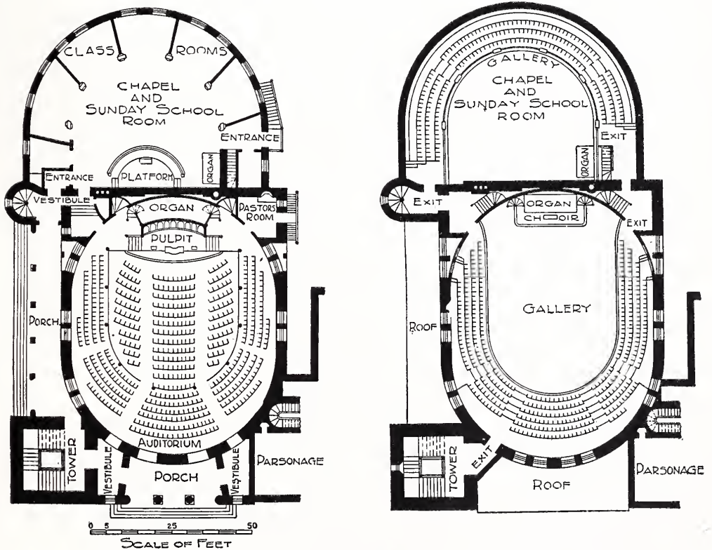
FIG. 12. FIRST M. E. CHURCH, BALTIMORE, MD. OVAL AUDITORIUM PLAN. McKim, Mead & White, Architects.
