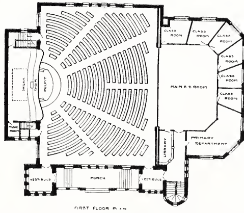
FIG. 24. FIRST PRESBYTERIAN CHURCH, GOVERN-NEUR, N. Y. S. R. Badgley, Architect.
