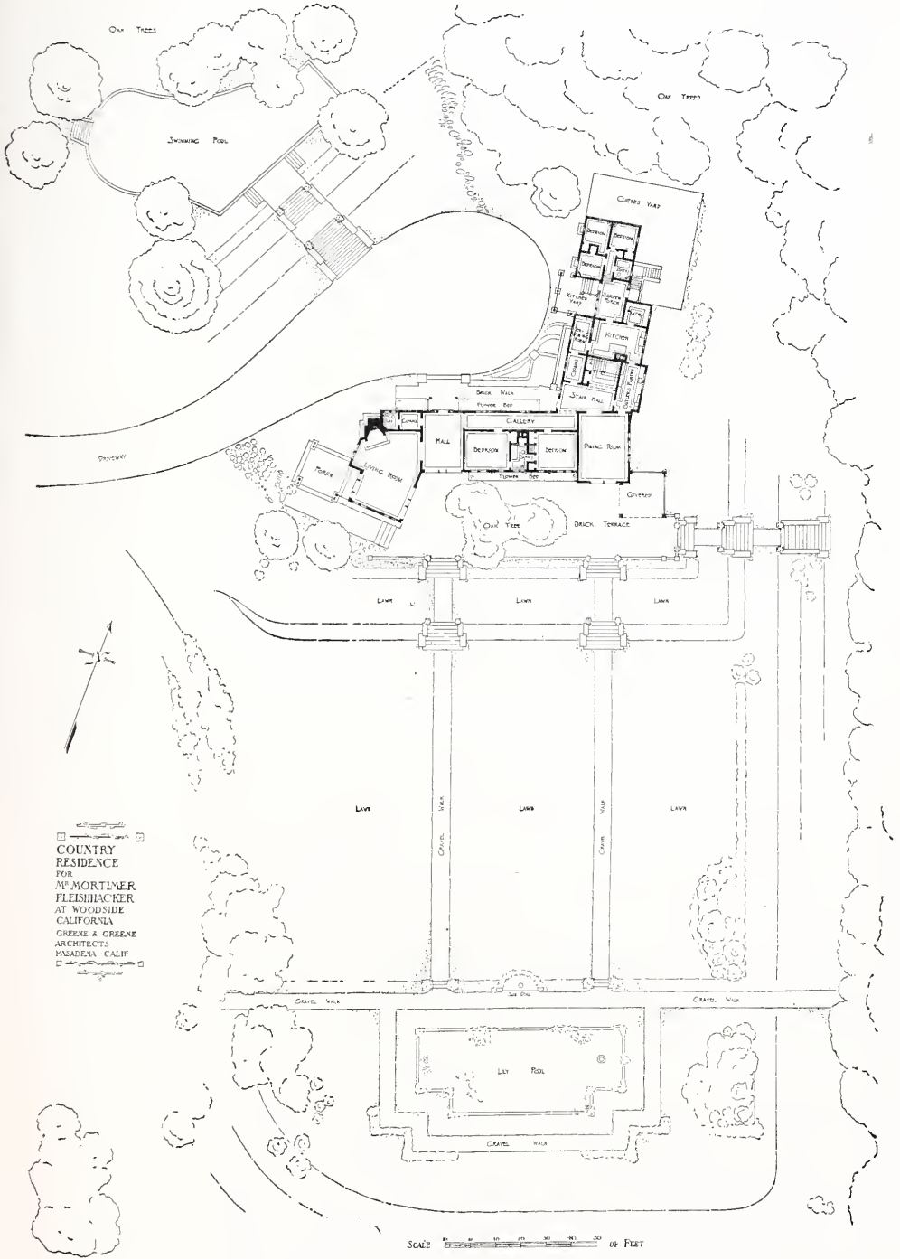
BLOCK PLAN—HOUSE OF MORTIMER FLEISHACKER, ESQ., WOODSIDE, CAL. GREENE & GREENE, ARCHITECTS.
