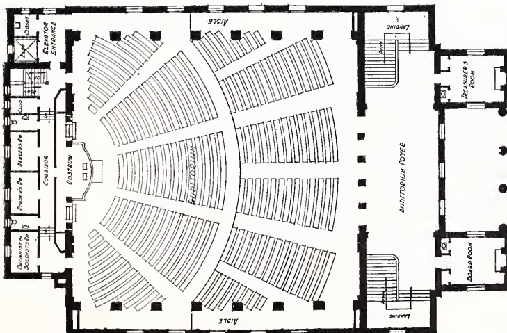
FIG. 21. FIRST CHURCH OF CHRIST SCIENTIST, LONG BEACH, CAL. SQUARE AUDIENCE HALL PLAN. Elmer Grey, Architect.
