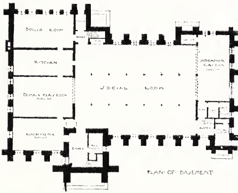
FIG. 24. FIRST PRESBYTERIAN CHURCH, GOVERN-NEUR, N. Y. S. R. Badgley, Architect.
