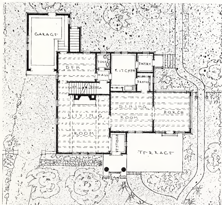
VIEW AND FIRST FLOOR PLAN—OWN HOUSE AT DES MOINES, IOWA. FRANK B. WETHERELL, ARCHITECT.
