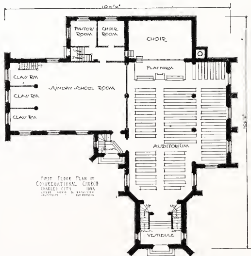
FIG. 25. CONGREGATIONAL CHURCH, CHARLES CITY, IOWA. Liebbe, Nourse & Rasmussen, Architects.
