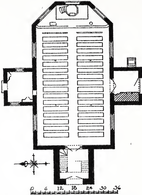
FIG. 1. OLD SWEDES' CHURCH, PHILADELPHIA, BUILT 1703. ADDITIONS OF SOUTH PORCH AND VESTRY MADE TO STRENGTHEN SIDE WALLS, 1702.
