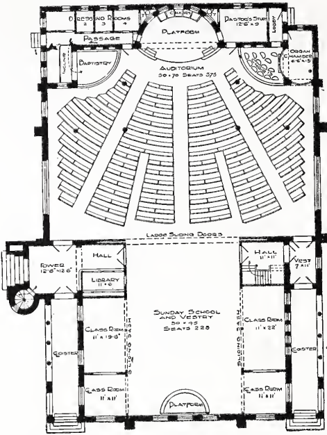
FIG. 8. FIRST BAPTIST CHURCH, COLORADO SPRINGS, CO. RECTANGULAR AUDIENCE HALL PLAN, PULPIT MIDDLE OF LONGER SIDE. L. B. Valk & Son, Architects.
