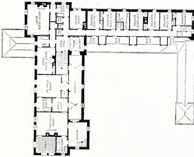
HOUSE AT EASTERN POINT-GLOUCESTER, MASS F-00 F-G HALL EQQ ARCHITECTS WILLIAM A. ALDRICH DESIGNED 1904
