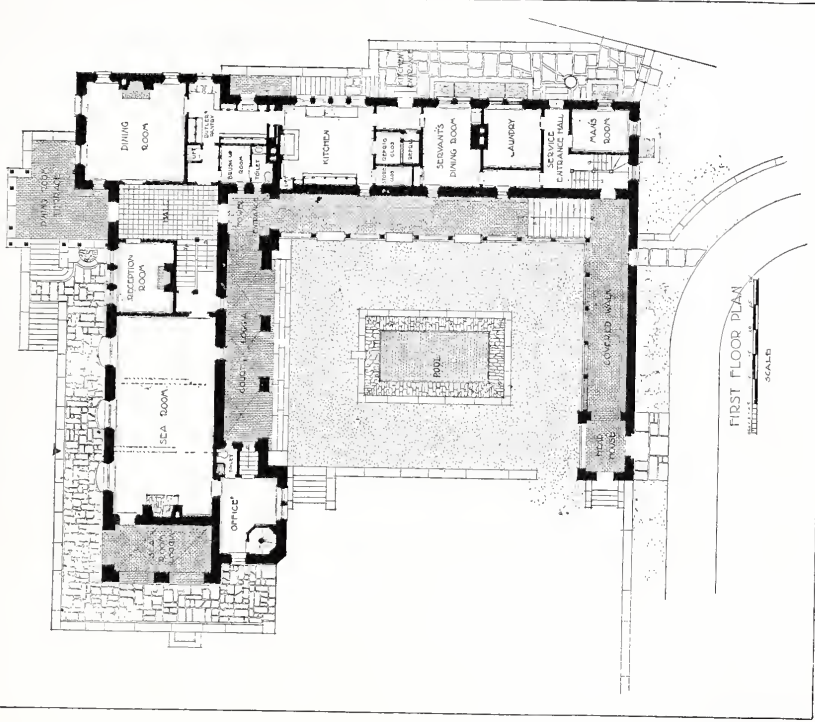
HOUSE AT EASTERN POINT-GLOUCESTER, MASS F-00 F-G HALL EQQ ARCHITECTS WILLIAM A. ALDRICH DESIGNED 1904
