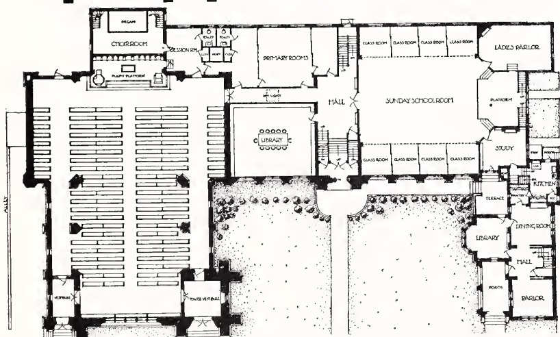
FIG. 8. RICHARDSON MEMORIAL PRESBYTERIAN CHURCH, PHILADELPHIA, PA. Charles W. Bolton & Sons, Architects.
