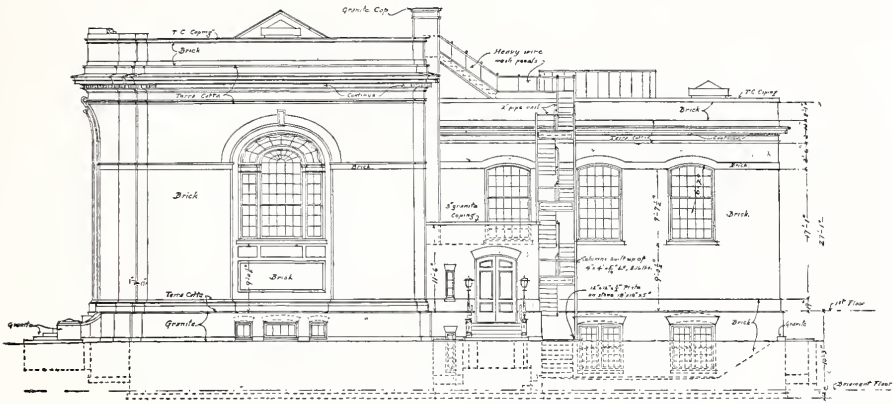
NORTH ELEVATION
