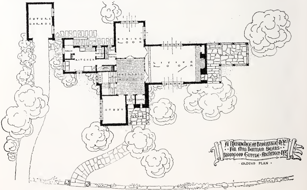
PLAN OF GROUNDS AND FIRST FLOOR—HOUSE OF MRS. BERTRAM SEARS, BRONXVILLE, N. Y. Bloodgood Tuttle, Architect.
