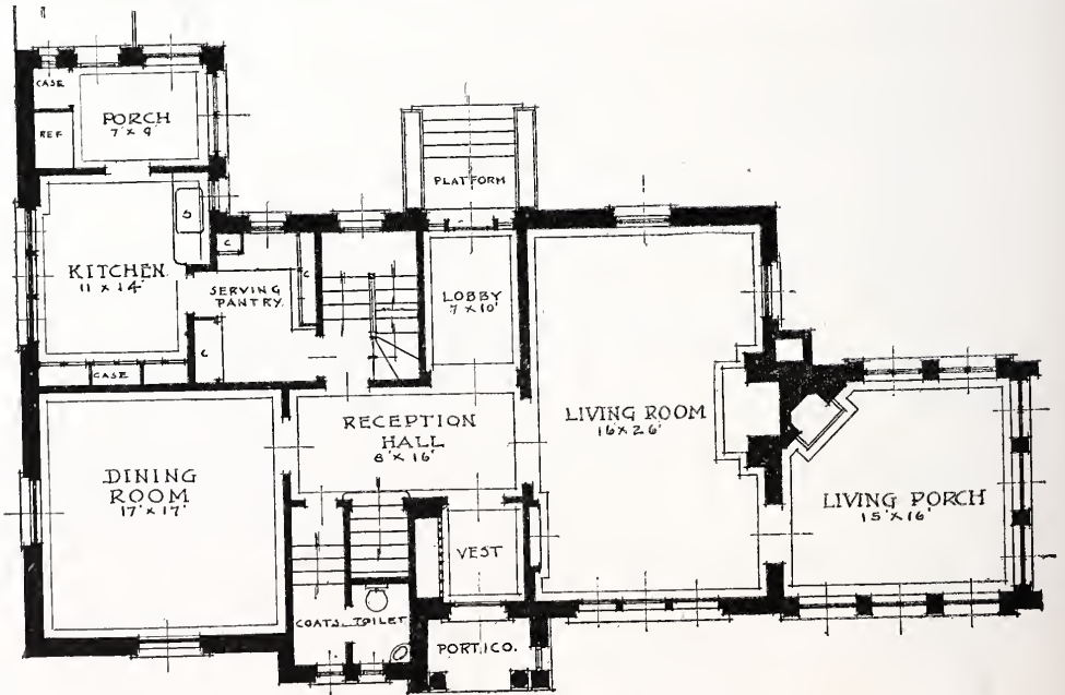
FIG. 13. VIEW AND FIRST FLOOR PLAN— HOUSE OF MORTON R. MAVOR, ESQ., HIGHLAND PARK, ILL. N. MAX DUNNING, ARCHITECT.
