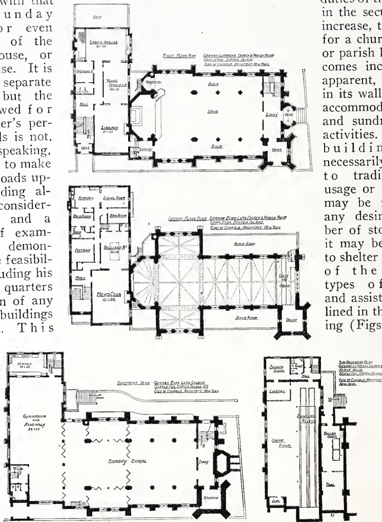
FIG. 5. GERMAN EVANGELICAL LUTHERAN CHURCH AND PARISH HOUSE, STAPLETON, S. I. George W. Conable, Architect.
