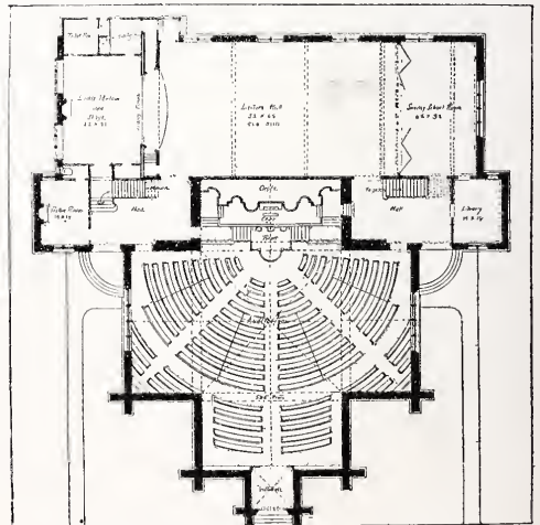
FIG. 29. PROPOSED UNITARIAN CHURCH, SOMERVILLE, MASS. TOWER APPEARS OVER ENTIRE CROSSING OF TWO ARMS OF GREEK CROSS. Cram, Wentworth & Goodhue, Architects.
