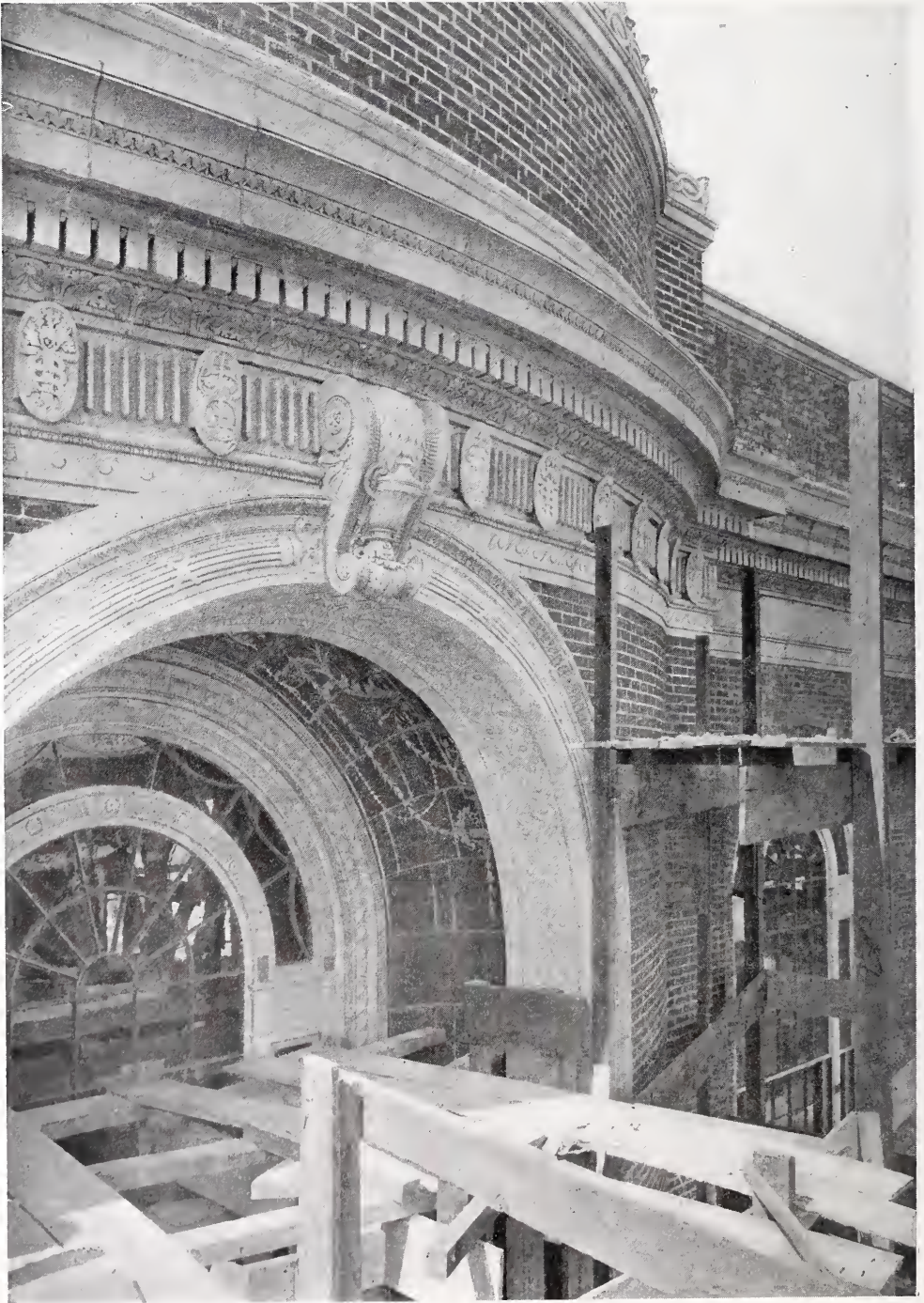
DETAIL OF MAIN ENTRANCE—HADDINGTON BRANCH OF THE FREE LIBRARY OF PHILA- DELPHIA. ALBERT KELSEY, ARCHITECT.
