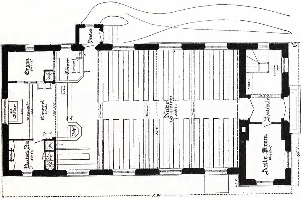
FIG. 15. ST. MARK'S ENGLISH LUTHERAN CHURCH, ROXBURY, MASS. SIMPLE MODERN PLAN. Gay & Proctor, Architects.
