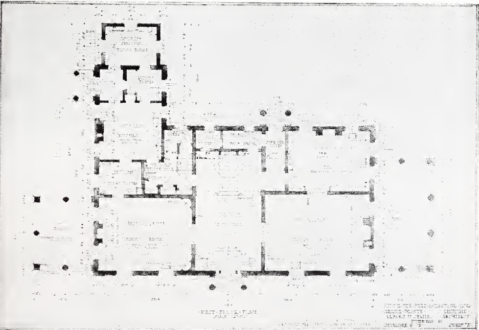
FIG. 29—VIEW AND FIRST FLOOR PLAN—HOUSE OF FORD BALLANTYNE, ESQ., GROSSE POINTE, MICH. ALBERT H. SPAHR, ARCHITECT.
