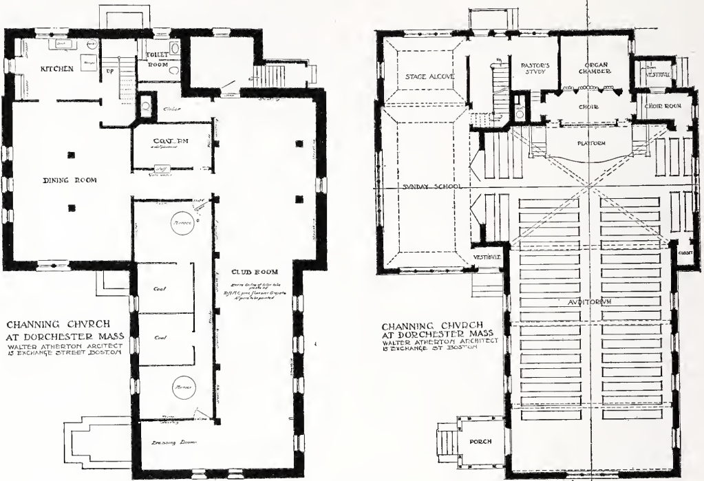
FIG. 13. BASEMENT AND MAIN FLOOR—CHANNING CHURCH, DORCHESTER, MASS.
