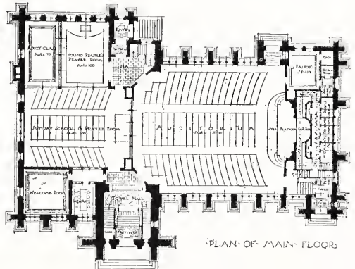
FIG. 24. FIRST PRESBYTERIAN CHURCH, GOVERN-NEUR, N. Y. S. R. Badgley, Architect.
