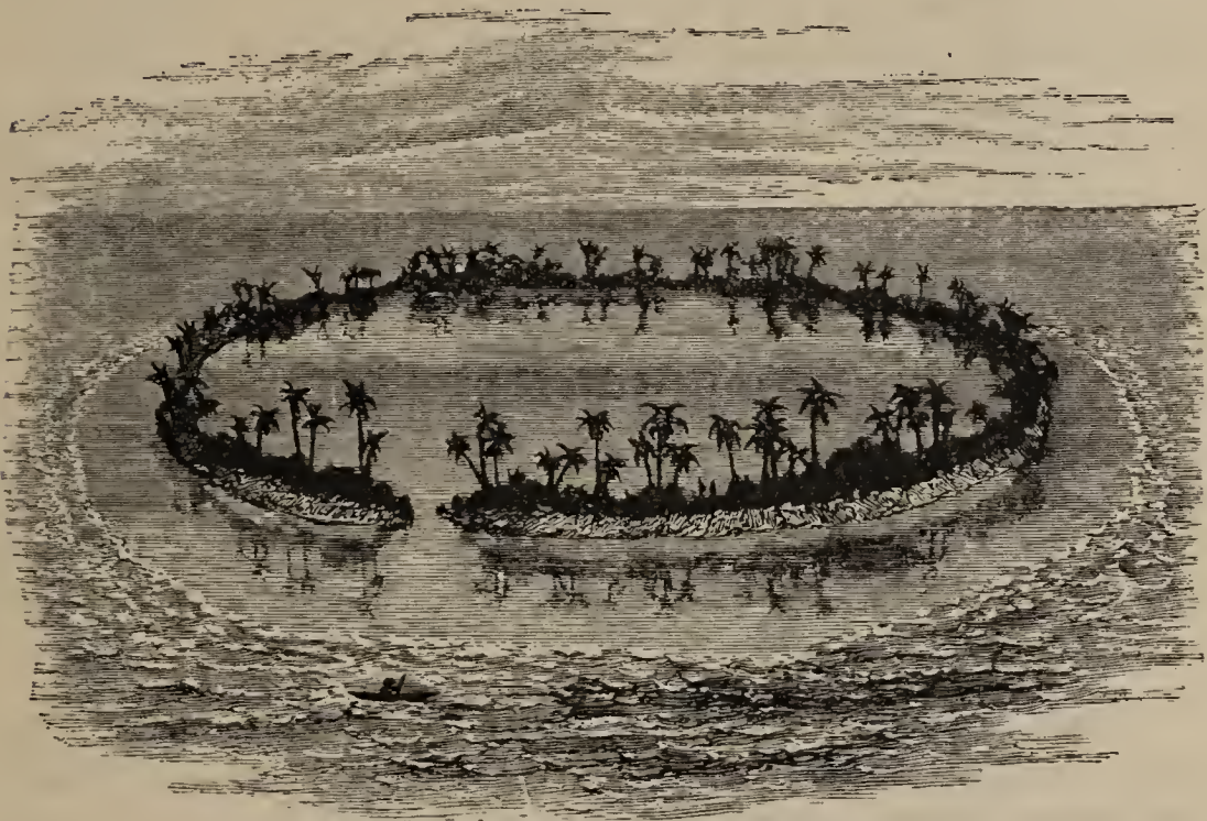
FIG. 26.—Atoll in the Pacific Ocean.
