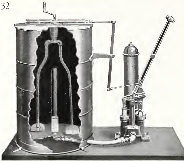
Cobb Park and Farm Sprayer.
