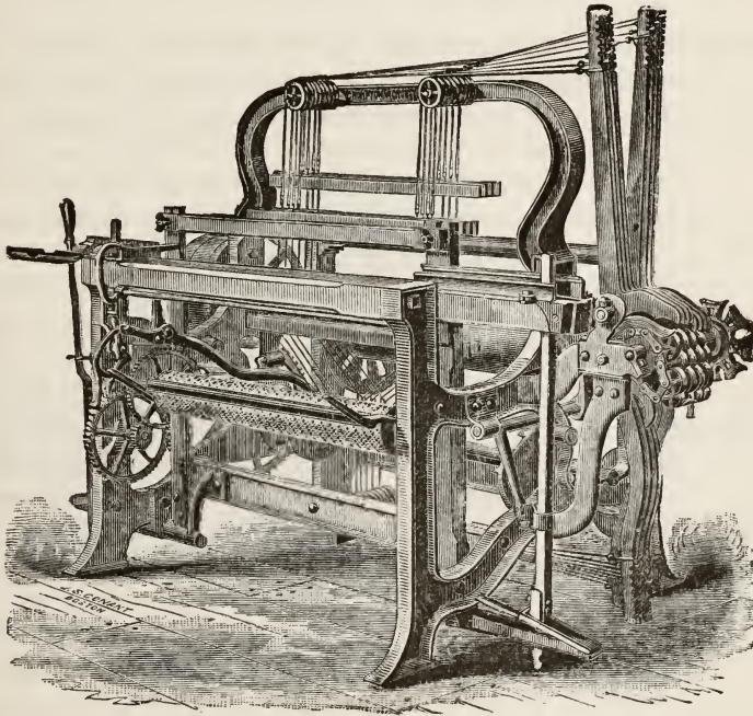
SATINET-LOOM.
