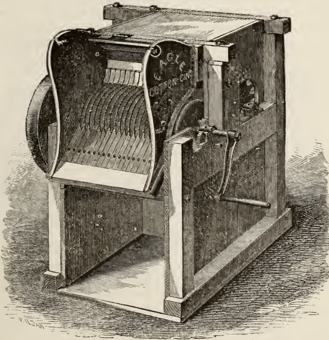
COTTON-GIN.
