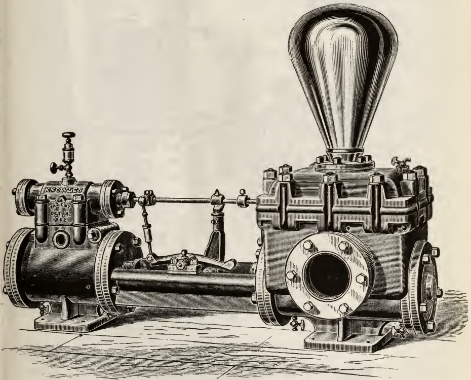
STEAM-PUMP.
