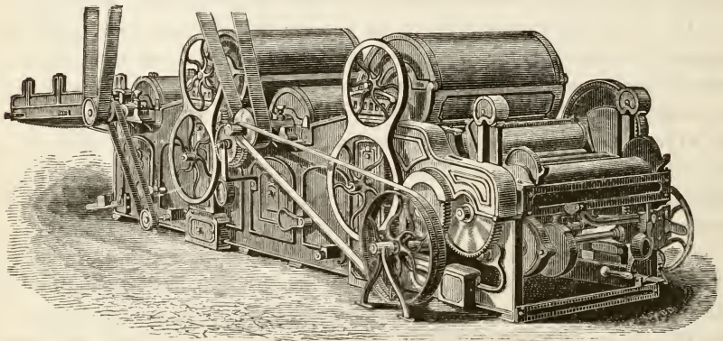
KITSON'S COTTON-PICKER.
