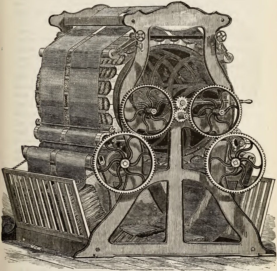
DOUBLE-ACTING GIG.
