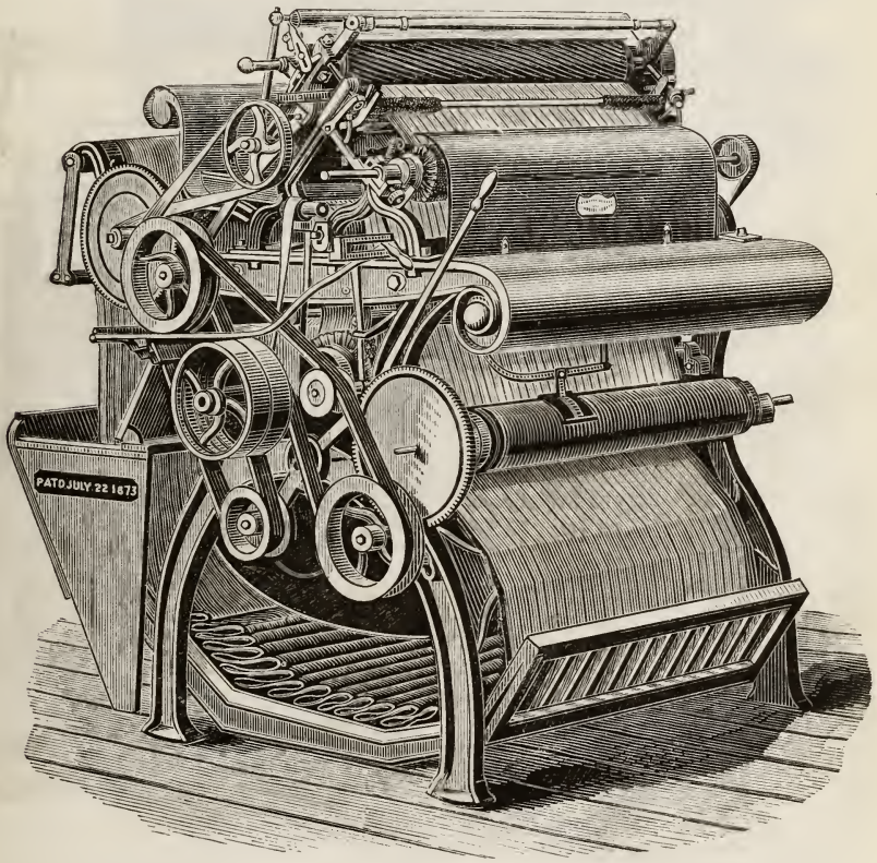
SHEARING-MACHINE.
