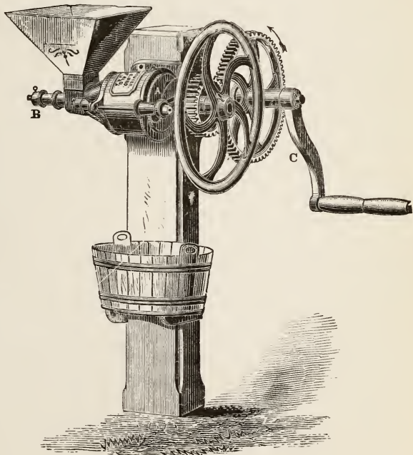
COFFEE-HULLER.
