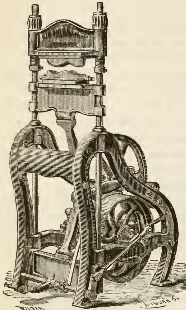
POWER SOLE-MOULDER.
