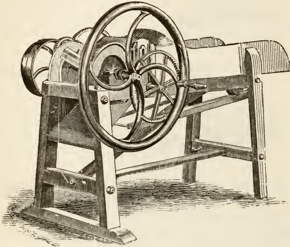
FODDER-CUTTER.
