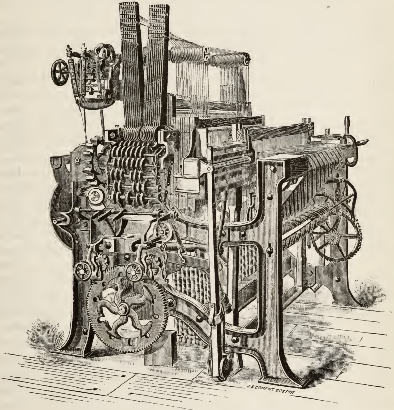
CHAIN TAPPET-LOOM.
