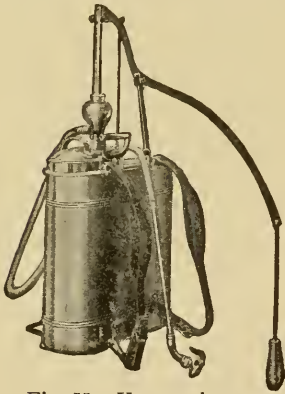
Fig. 55.—Knapsack sprayer.
